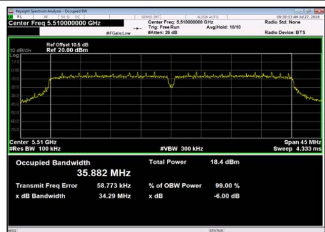
U-NII-2c 6dB Bandwidth-802.11n(40MHz) ,5510MHz
