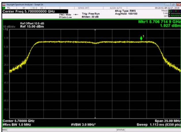
U-NII-2c Power spectral density-802.1 1n(20MHz),5700MHz
