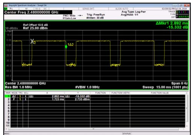
pi/4DQPSK,2480,2DH5,Transmission Time
