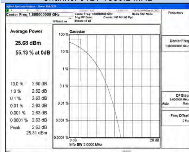
Channel 661 / 1880 MHz
