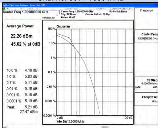
Channel 810 / 1909.8 MHz
