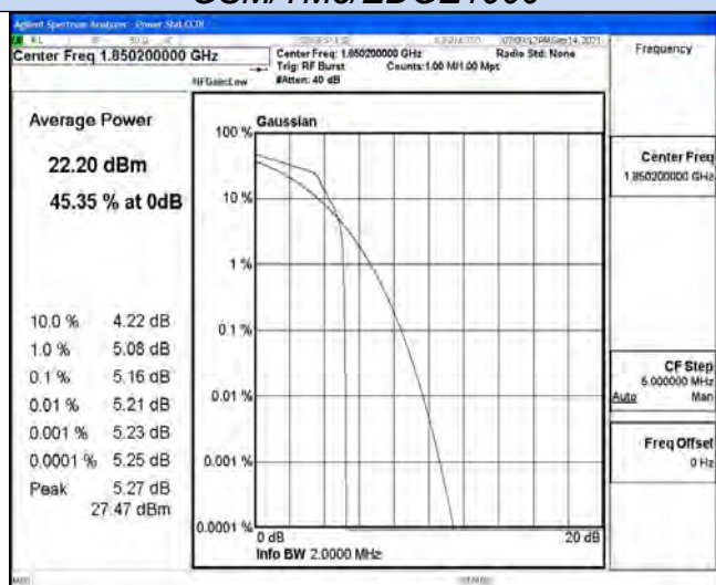
Channel 512 / 1850.2 MHz
