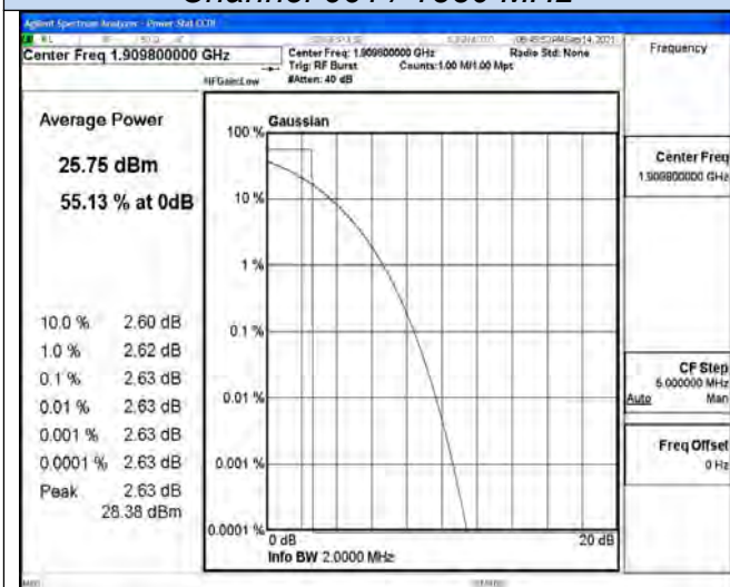
Channel 810 / 1909.8 MHz
