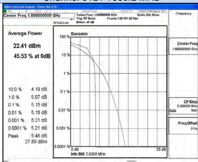
Channel 661 / 1880 MHz
