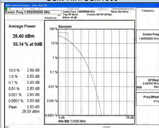
Channel 512 / 1850.2 MHz
