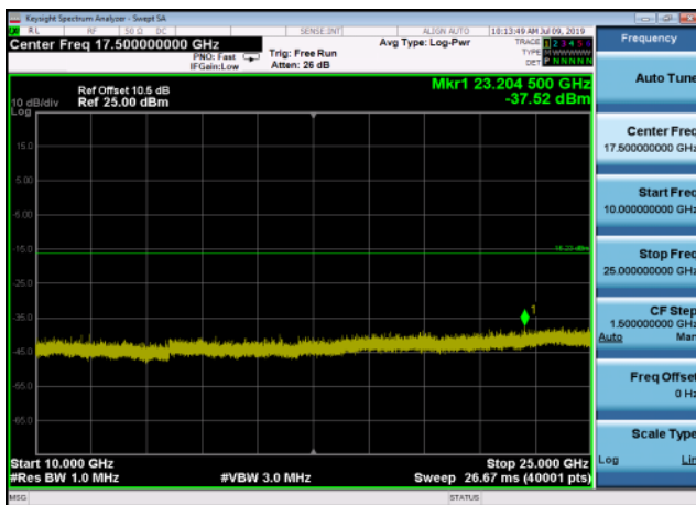
Conducted Emission: 8PSK,2480,3DH5 ,10000MHz~25000MHz
