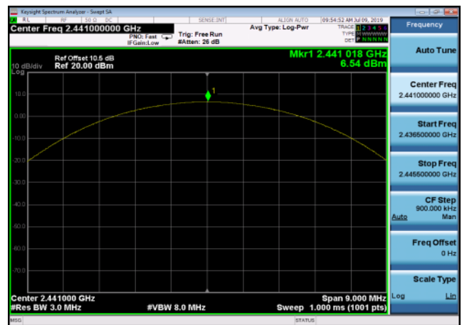
Output Power: 8PSK,2441MHz,3DH5
