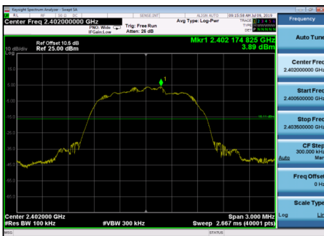
Conducted Emission: 8PSK,2402,3DH5 ,Reference Level
