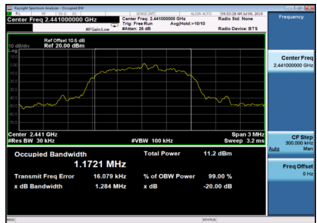
20dB Bandwidth: 8PSK,2441MHz,3DH5
