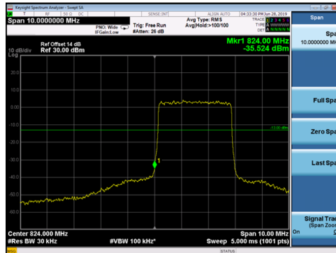
LowRange_FDD05_5MHz_826.5_OneRB _low_QPSK
