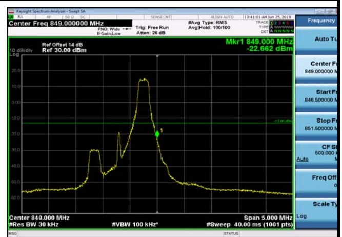
HighRange_FDD05_1.4MHz_848.3_fullRB _High_Q16
