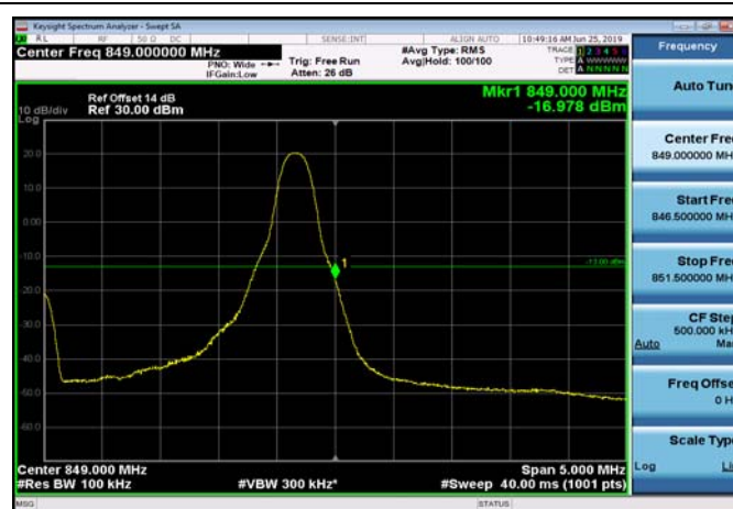
HighRange_FDD05_5MHz_846.5_fullRB _High_QPSK
