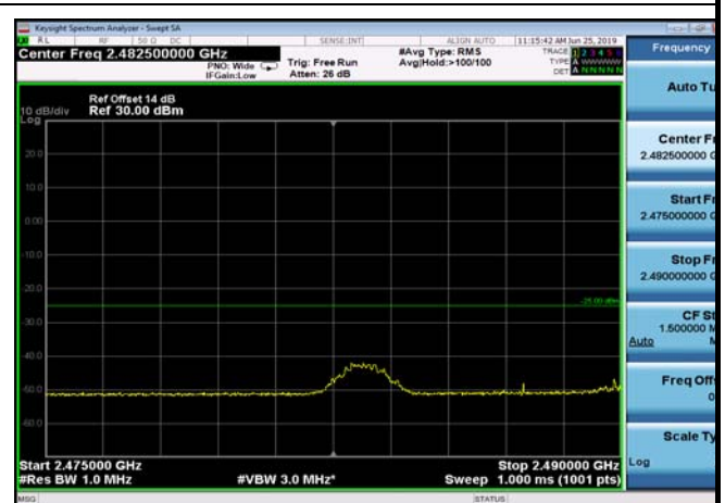
LowRange_FDD07_20MHz_2510_fullRB _Low_QPSK
