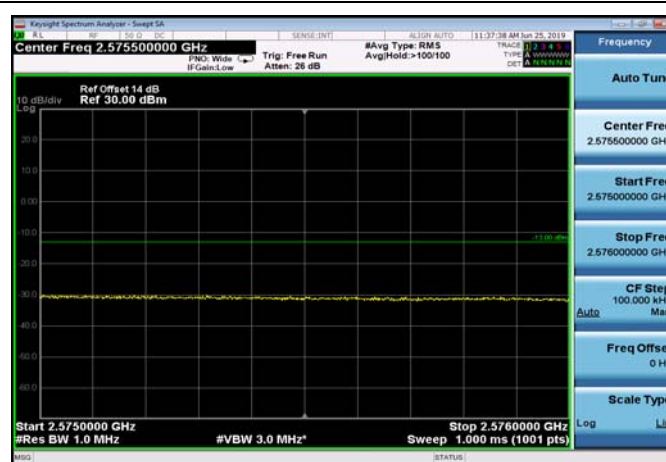
FDD07_15MHz_2562.5_QPSK_fullRB _ExtraBands_Range_2575~2576
