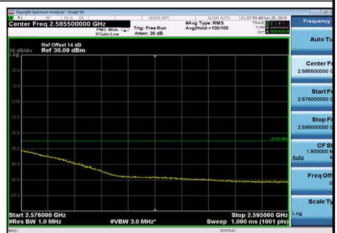
FDD07_15MHz_2562.5_QPSK_fullRB _ExtraBands_Range_2576~2595
