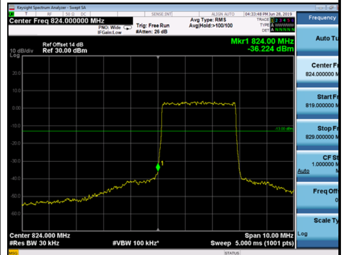
LowRange_FDD05_5MHz_826.5_OneRB _low_Q16
