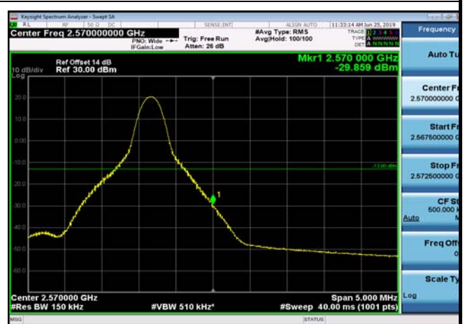
HighRange_FDD07_15MHz_2562.5_OneRB _high_Q16
