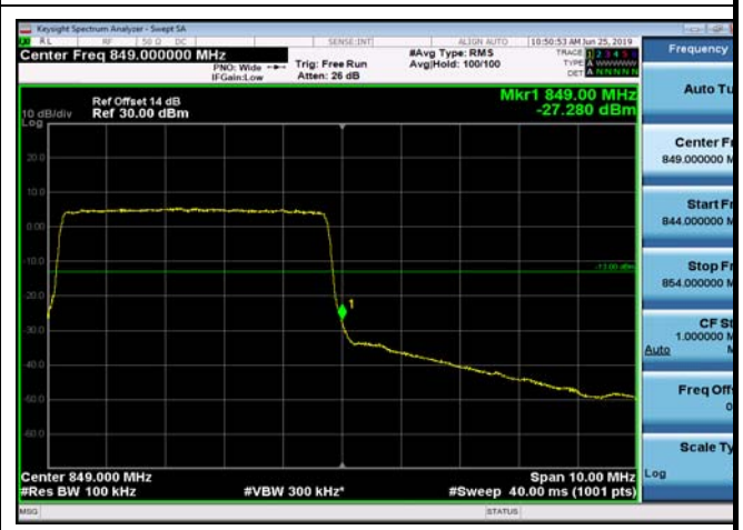
HighRange_FDD05_5MHz_846.5_fullRB _High_Q16
