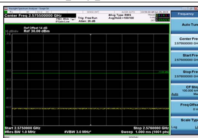
FDD07_5MHz_2502.5_Q16_fullRB_ExtraBan ds_Range_2575~2576
