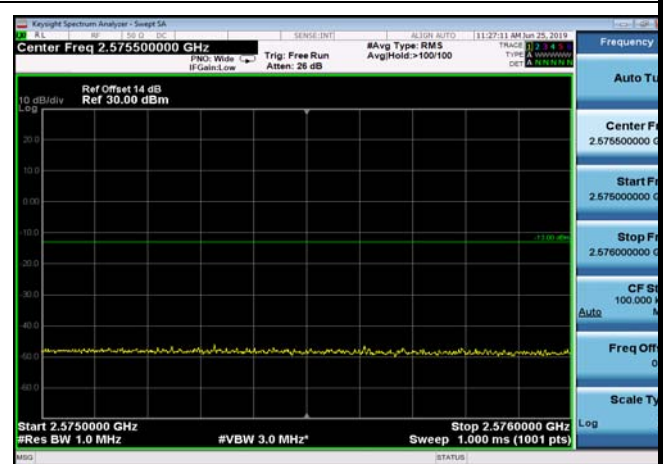
FDD07_10MHz_2565_Q16_OneRB_high_ExtraBands_Range_2575~2576
