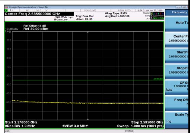
HighRange_FDD07_10MHz_2565_OneRB_high_Q16
