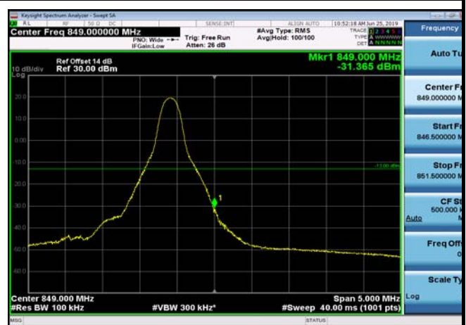
HighRange_FDD05_10MHz_844_fullRB _High_Q16
