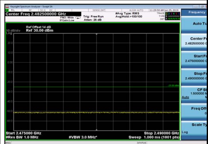
FDD07_10MHz_2565_QPSK_fullRB_ExtraBands_Range_2475~2490
