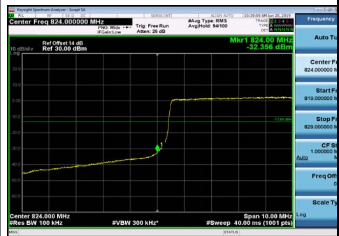
LowRange_FDD05_10MHz_829_fullRB _Low_Q16
