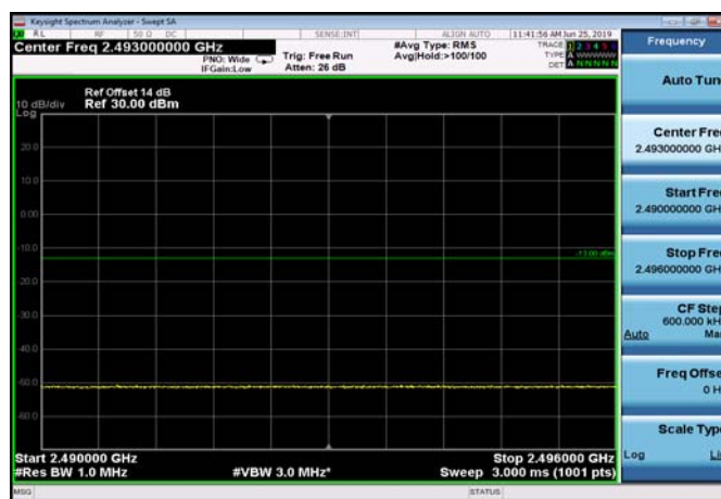
HighRange_FDD07_20MHz_2560_fullRB _High_Q16
