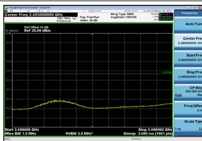
LowRange_FDD07_10MHz_2505_fullRB _Low_Q16
