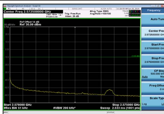
FDD07_10MHz_2565_Q16_OneRB_high_ExtraBands_Range_2570~2575
