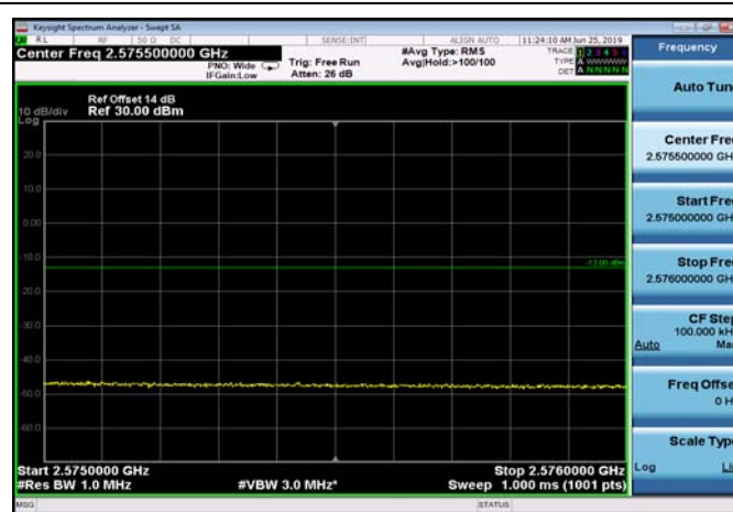
HighRange_FDD07_10MHz_2565_OneRB_high_QPSK
