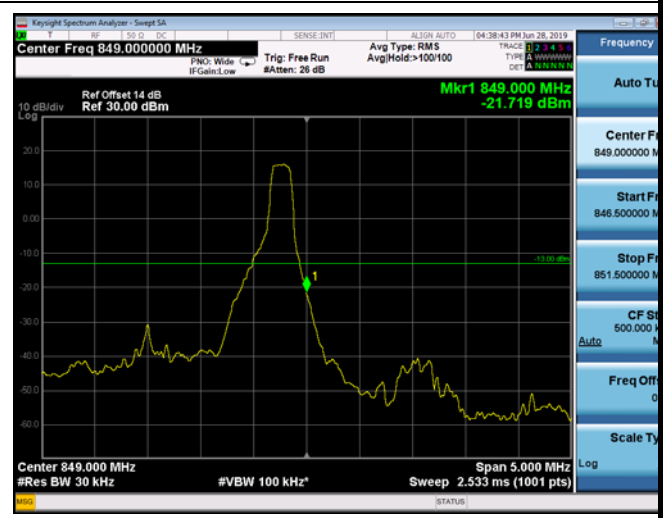
HighRange_FDD05_3MHz_847.5_OneRB _high_Q16
