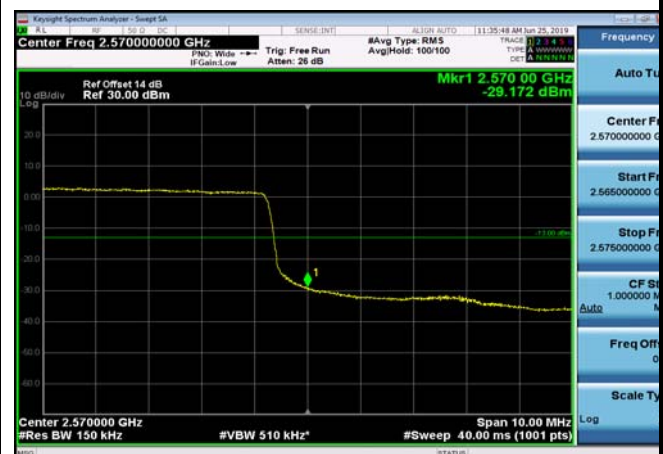
HighRange_FDD07_15MHz_2562.5_fullRB _High_QPSK
