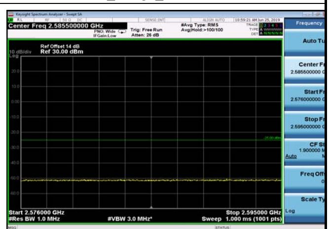
FDD07_5MHz_2502.5_Q16_fullRB_ExtraBan ds_Range_2576~2595
