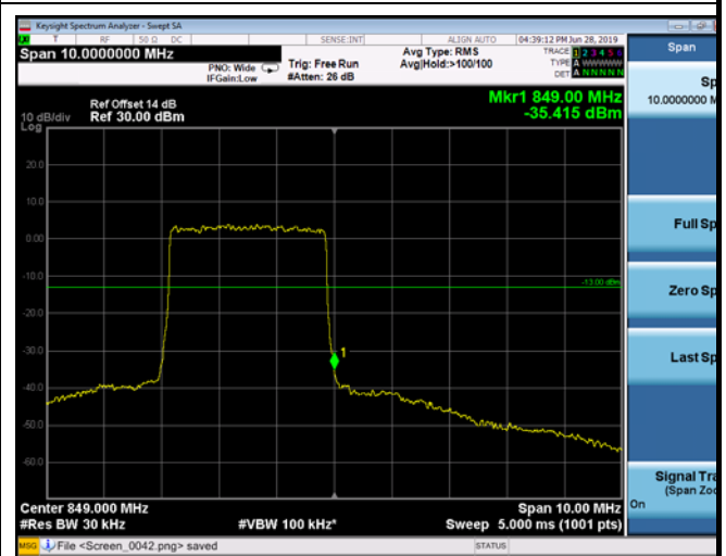
HighRange_FDD05_5MHz_846.5_OneRB _high_Q16
