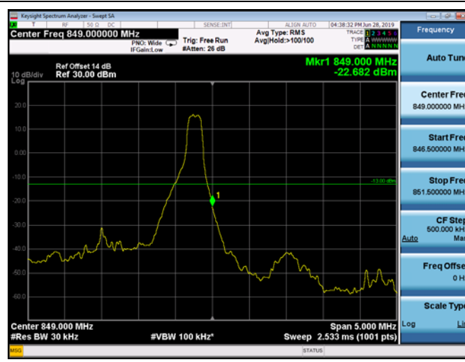
HighRange_FDD05_3MHz_847.5_OneRB _high_QPSK
