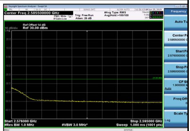
HighRange_FDD07_15MHz_2562.5_OneRB _high_Q16
