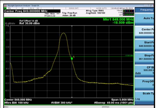
HighRange_FDD05_5MHz_846.5_fullRB _High_Q16
