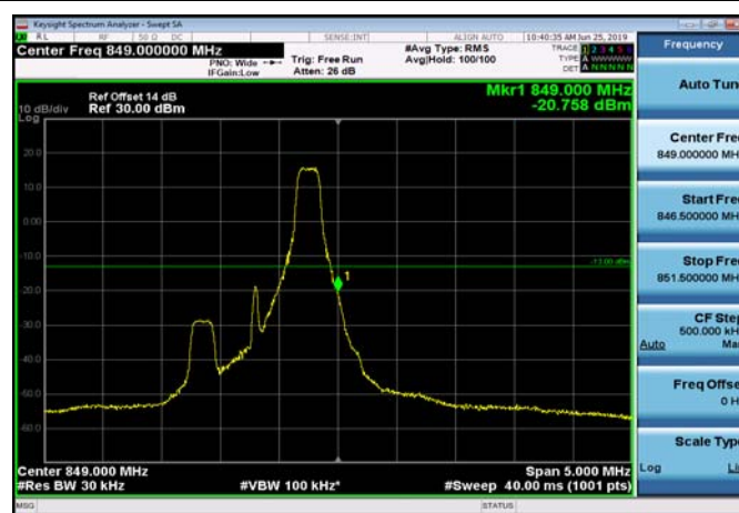
HighRange_FDD05_1.4MHz_848.3_fullRB _High_QPSK
