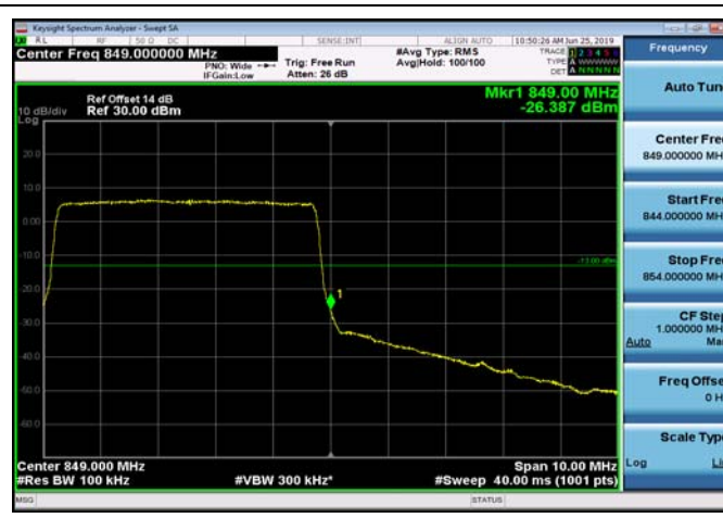
HighRange_FDD05_5MHz_846.5_fullRB _High_QPSK
