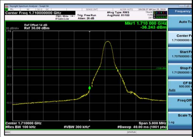
LowRange_FDD04_10MHz_1715_OneRB _low_Q16
