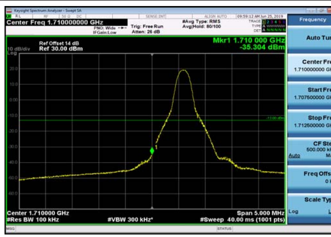
LowRange_FDD04_10MHz_1715_OneRB _low_QPSK
