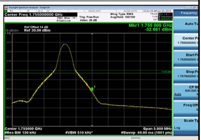
HighRange_FDD04_15MHz_1747.5_fullRB _High_Q16
