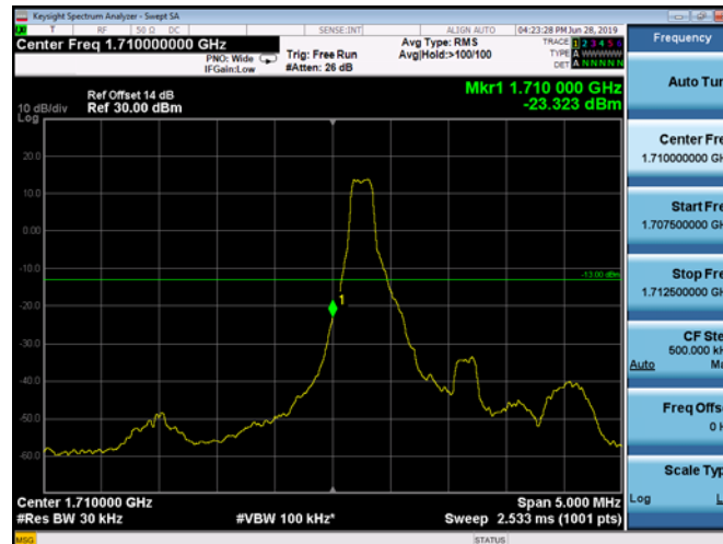
LowRange_FDD04_1.4MHz_1710.7_fullRB _Low_QPSK
