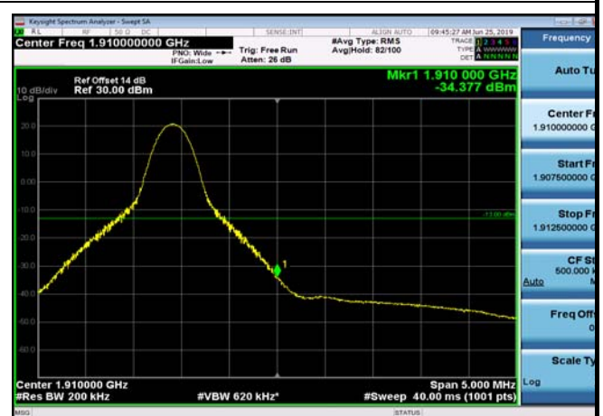
HighRange_FDD02_20MHz_1900_fullRB _High_Q16
