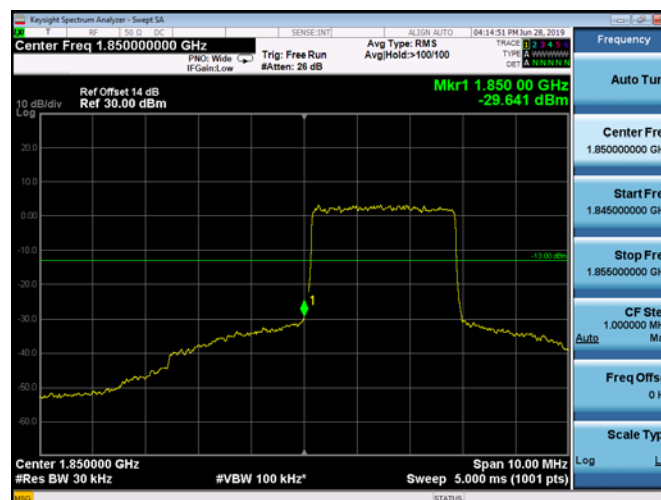
LowRange_FDD02_3MHz_1851.5_fullRB _Low_QPSK
