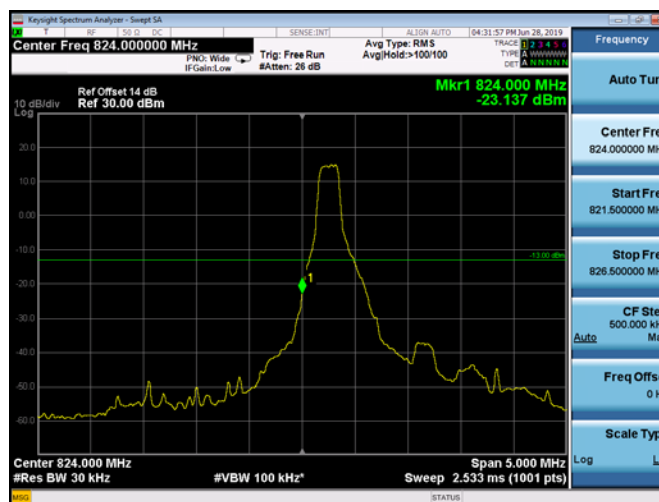
LowRange_FDD05_1.4MHz_824.7_OneRB _low_QPSK
