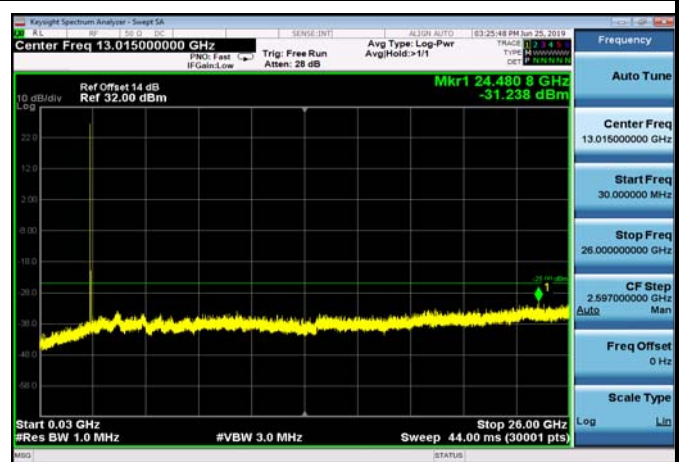
FDD07_LowRange_5MHz_30MHz~26GHz
