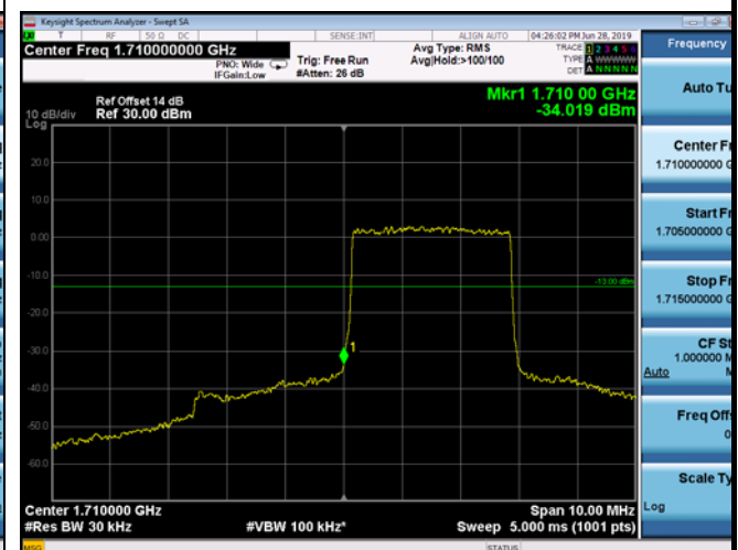
LowRange_FDD04_3MHz_1711.5_fullIRB _Low_Q16
