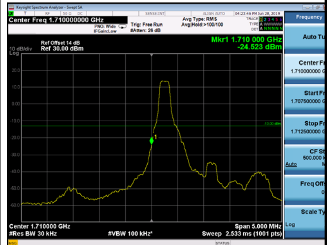
LowRange_FDD04_1.4MHz_1710.7_fullRB _Low_Q16
