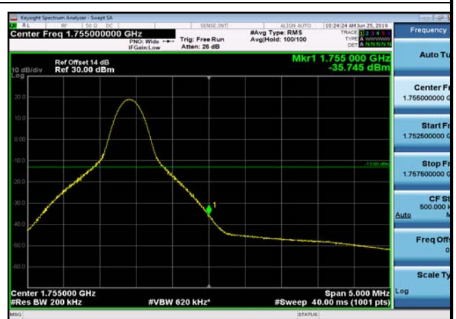
HighRange_FDD04_20MHz_1745_OneRB _high_Q16
