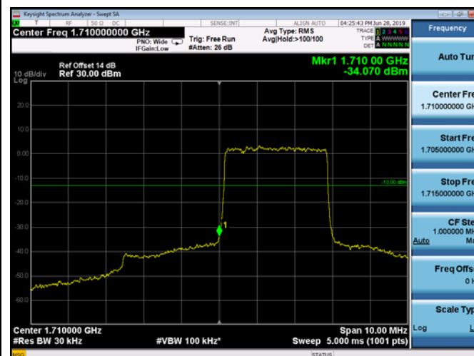
LowRange_FDD04_3MHz_1711.5_fullIRB _Low_QPSK
