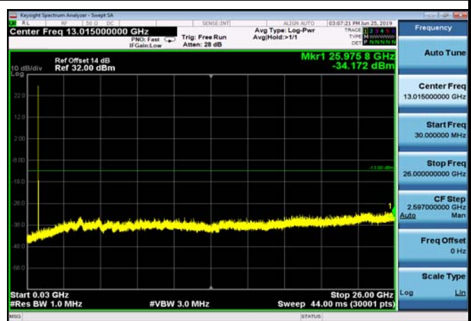
FDD07_HighRange_15MHz_30MHz~26GHz
