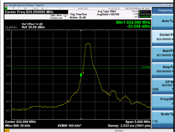
LowRange_FDD05_1.4MHz_824.7_OneRB _low_Q16
