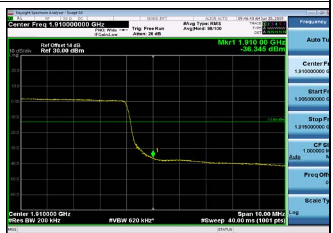
HighRange_FDD02_20MHz_1900_fullRB _High_Q16
