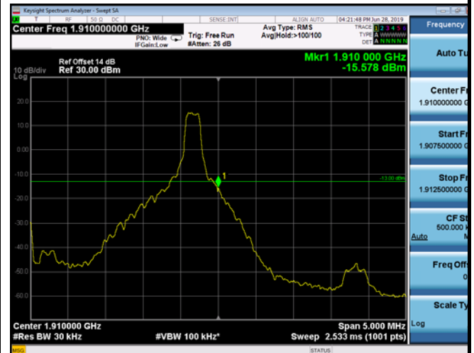
HighRange_FDD02_5MHz_1907.5_fullIRB _High_Q16
