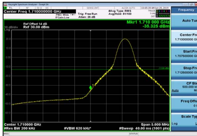
LowRange_FDD04_20MHz_1720_fullIRB _Low_QPSK
