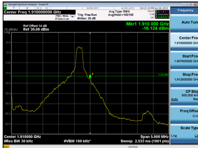
HighRange_FDD02_5MHz_1907.5_fullIRB _High_QPSK
