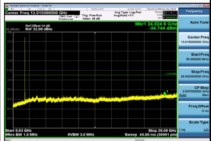
FDD02_HighRange_20MHz_30MHz~26GHz
