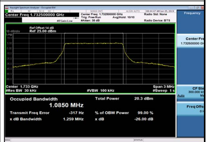
FDD04_MidRange_3_1732.5_Q16
