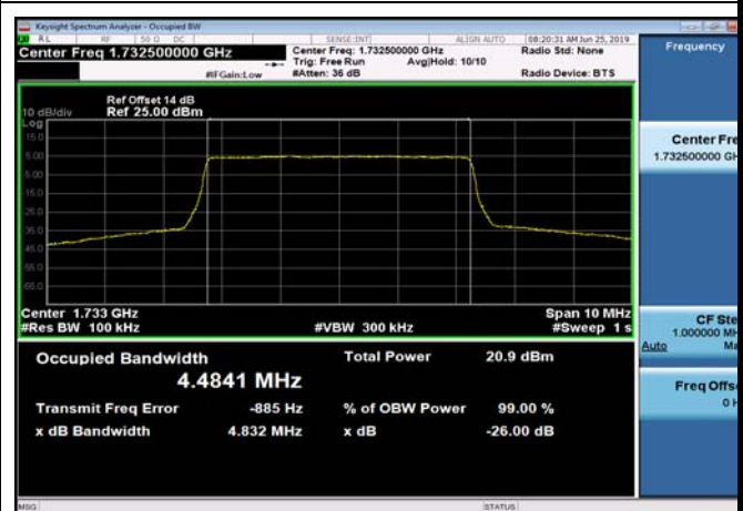
FDD04_MidRange_5MHz_1732.5MHz_QPSK
