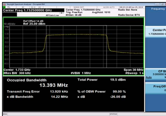
FDD04_MidRange_15MHz_1732.5MHz _Q16
