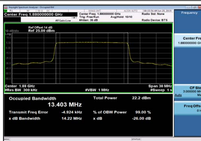
FDD02_MidRange_15MHz_1880MHz_QPSK
