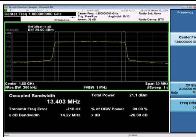
FDD02_MidRange_15MHz_1880MHz_Q16
