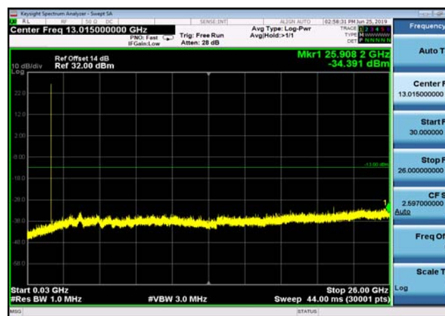
FDD05_HighRange_1.4MHz_30MHz~26GHz
