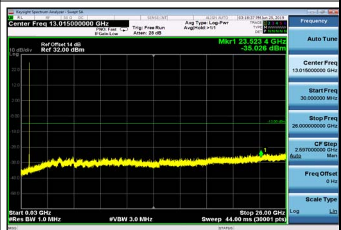
FDD05_HighRange_10MHz_30MHz~26GHz
