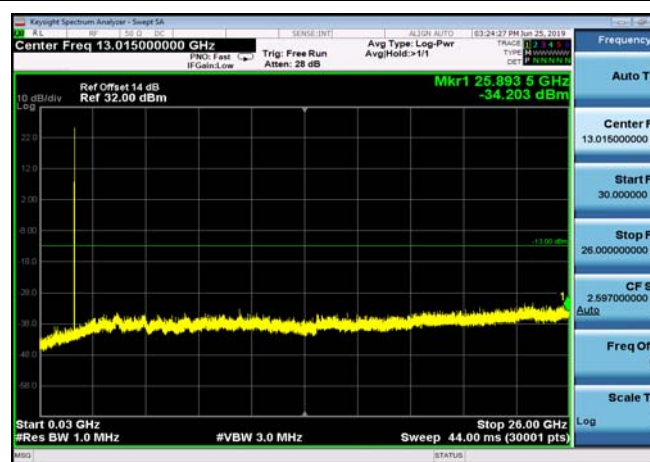
FDD04_MidRange_3MHz_30MHz~26GHz
