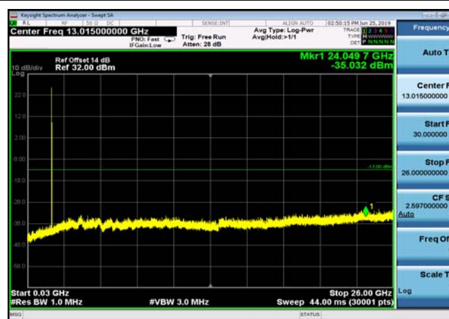
FDD04_HighRange_15MHz_30MHz~26GHz
