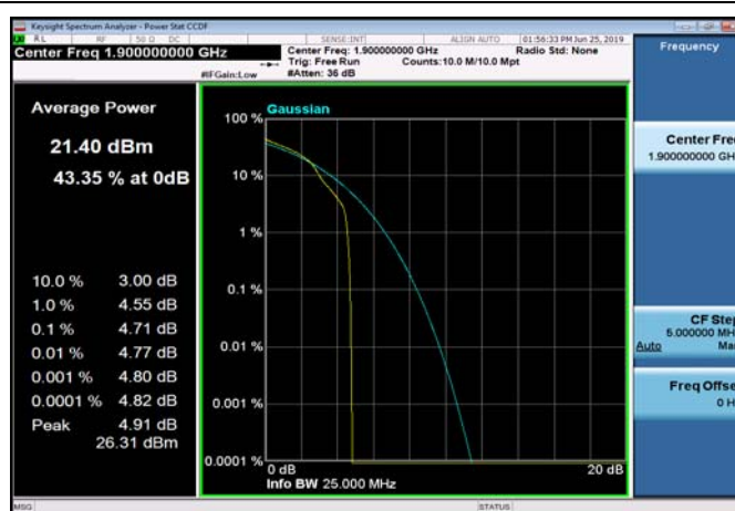
FDD02_HighRange_20MHz_1900_OneRB _high_Q16
