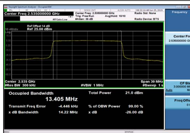
FDD07_MidRange_15MHz_2535MHz_Q16
