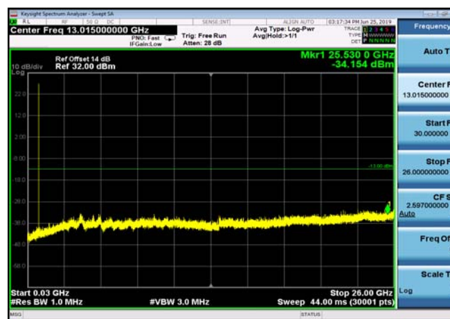
FDD05_MidRange_1.4MHz_30MHz~26GHz
