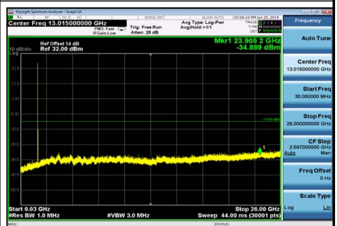
FDD04_HighRange_5MHz_30MHz~26GHz
