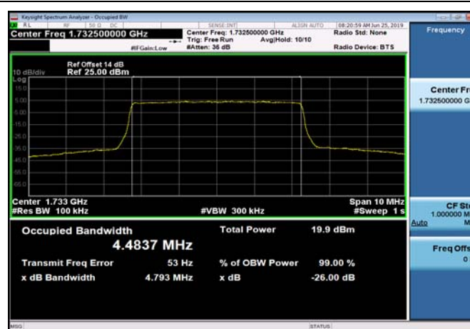
FDD04_MidRange_5MHz_1732.5MHz_Q16
