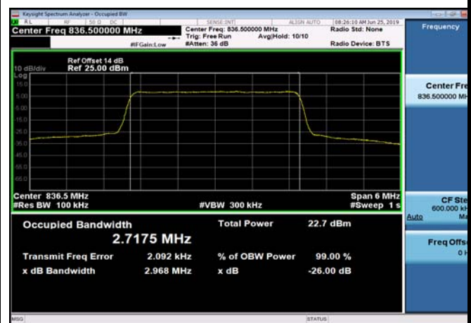
FDD05_MidRange_3MHz_836.5MHz_QPSK
