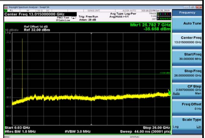
FDD04_MidRange_10MHz_30MHz~26GHz
