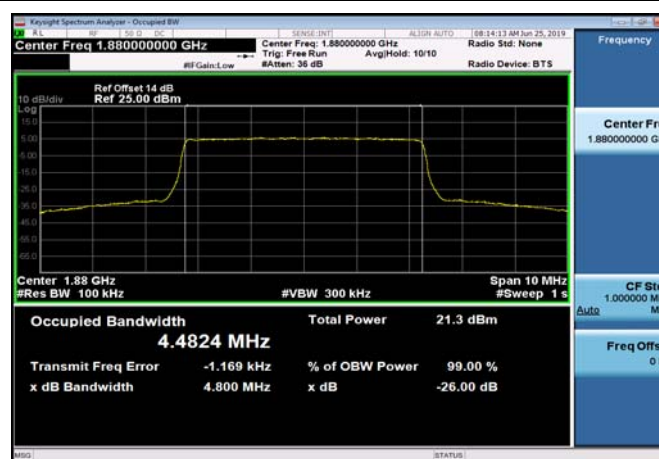
FDD02_MidRange_5MHz_1880MHz_Q16
