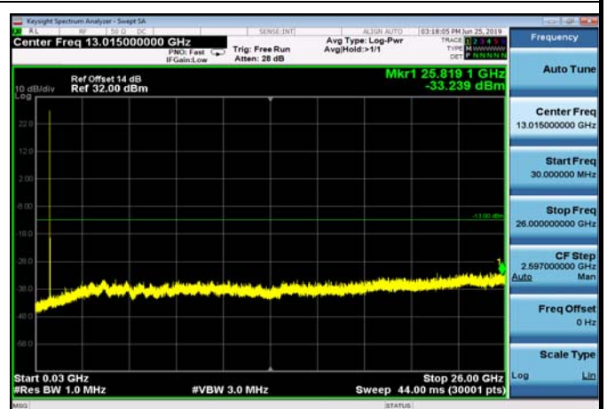
FDD05_MidRange_10MHz_30MHz~26GHz
