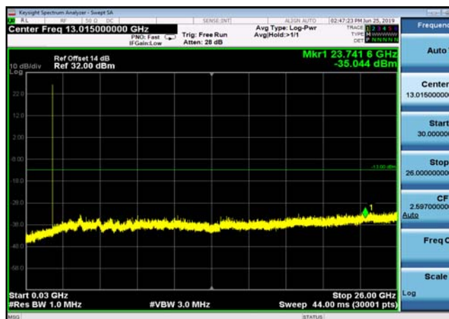
FDD02_HighRange_15MHz_30MHz~26GHz
