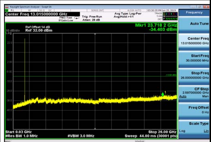
FDD02_HighRange_5MHz_30MHz~26GHz
