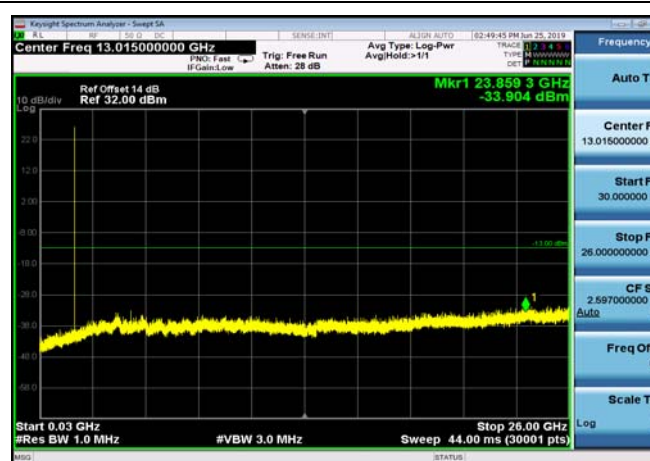
FDD04_MidRange_1.4MHz_30MHz~26GHz
