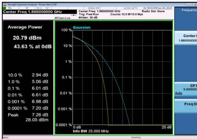
FDD02_MidRange_20MHz_1880_fullIRB _Q16
