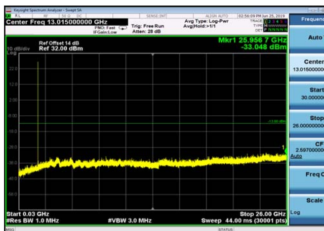
FDD02_HighRange_3MHz_30MHz~26GHz
