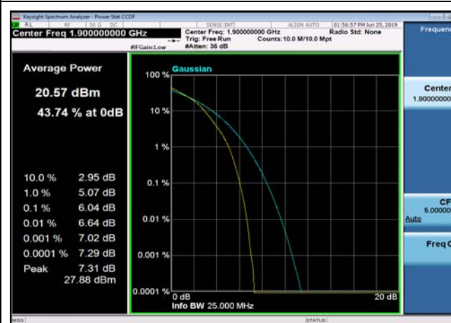
FDD02_HighRange_20MHz_1900_fullRB _Q16
