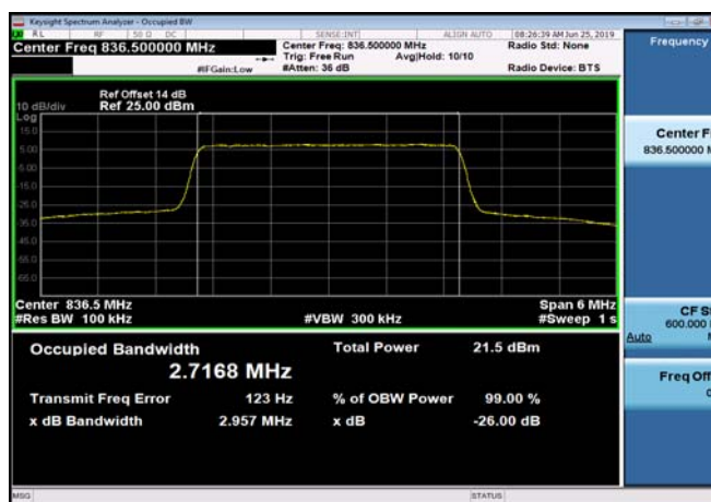
FDD05_MidRange_3MHz_836.5MHz_Q16
