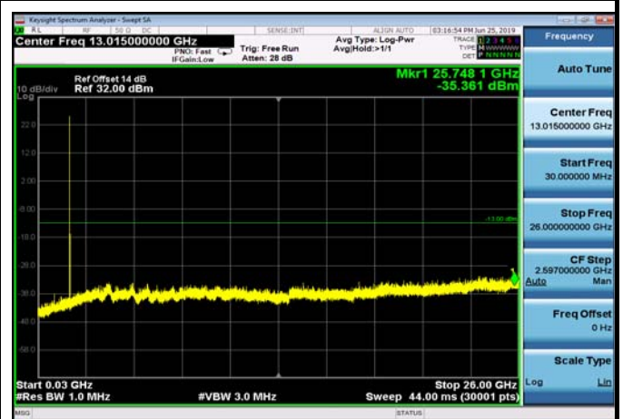
FDD04_HighRange_20MHz_30MHz~26GHz
