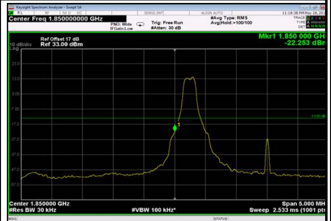
LowRange_FDD02_3MHz_1851.5_fullRB _LowQ16 22
