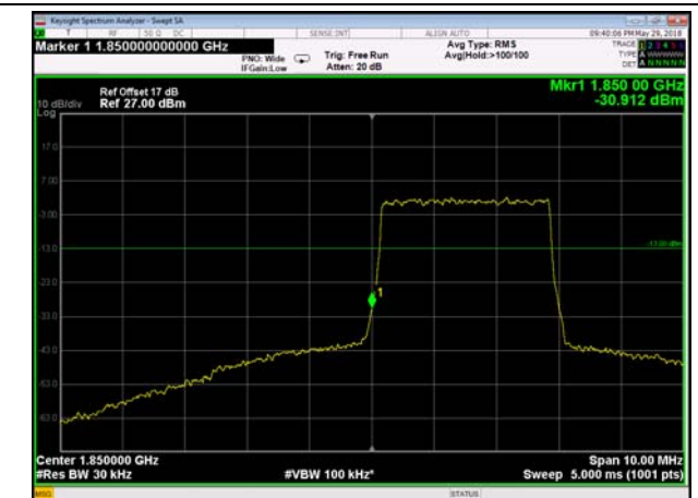
LowRange_FDD02_5MHz_1852.5_OneRB _low_Q16
