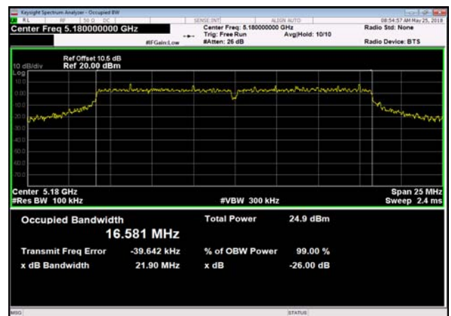
U-NII-1,802.11a(20MHz),5180MHz
