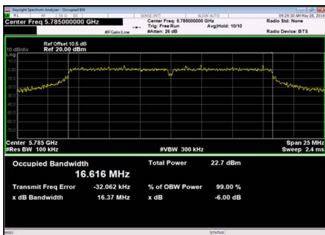
U-NII-3,802.11a(20MHz),5785MHz
