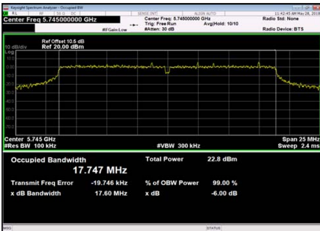
U-NII-3,802.11n(20MHz),5745MHz
