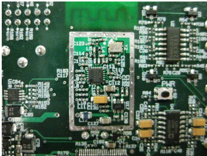
Close-Up of RF Section – Shield Removed
