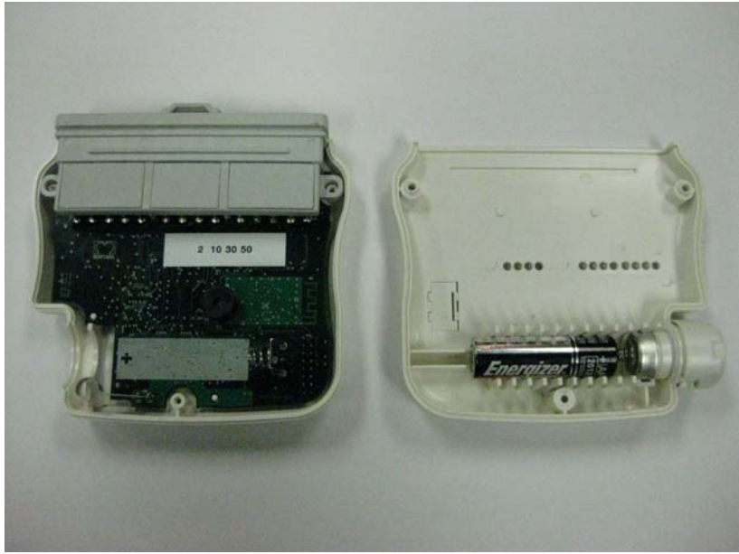
Open for Inspection, Showing Battery Compartment
