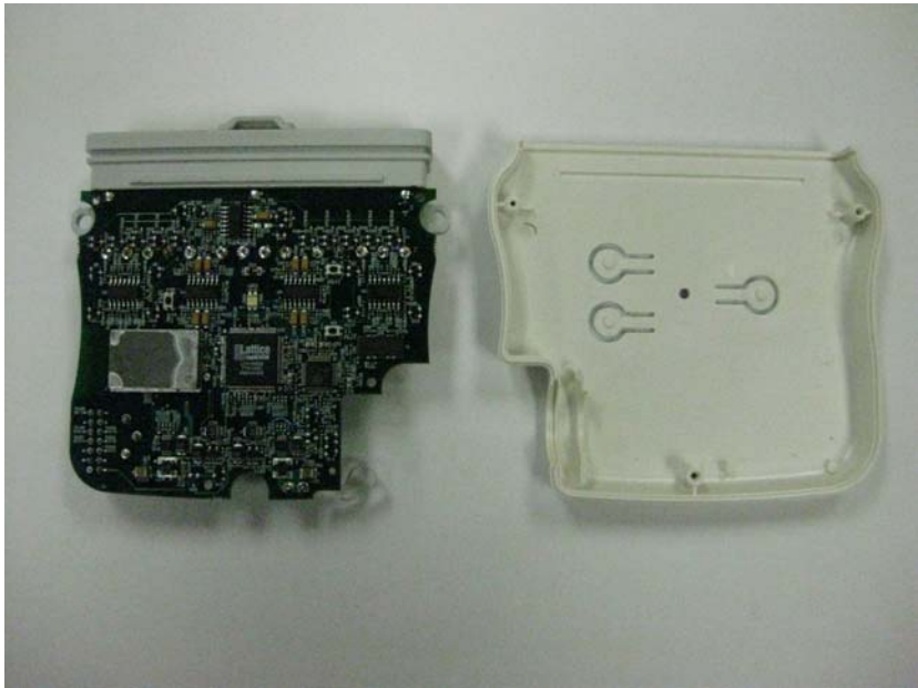
Open for Inspection, Showing RF Section
