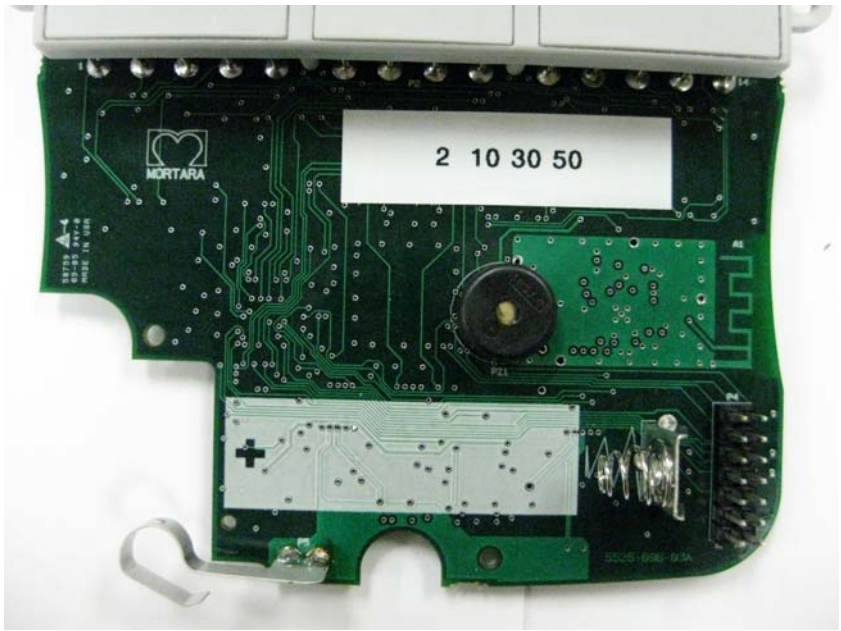
Close-Up of Back Side of Board
