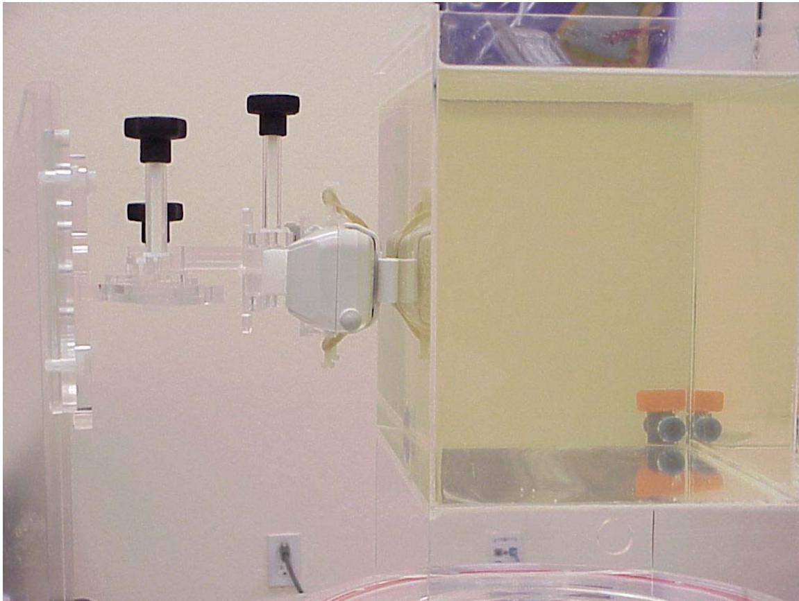
Photo 4. Body SAR
