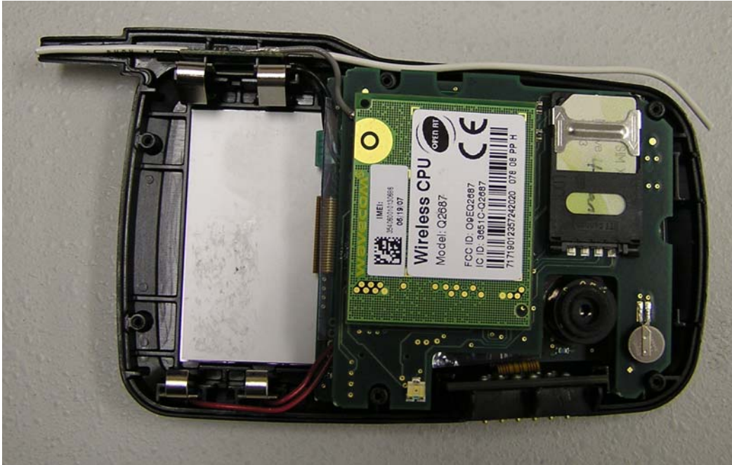
EUT - Assembled
