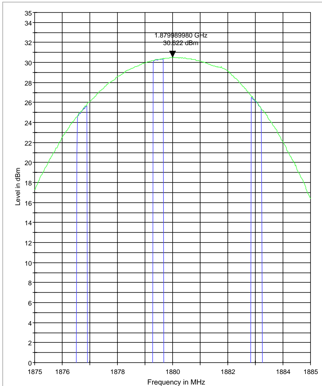
EIRP 1900 M
