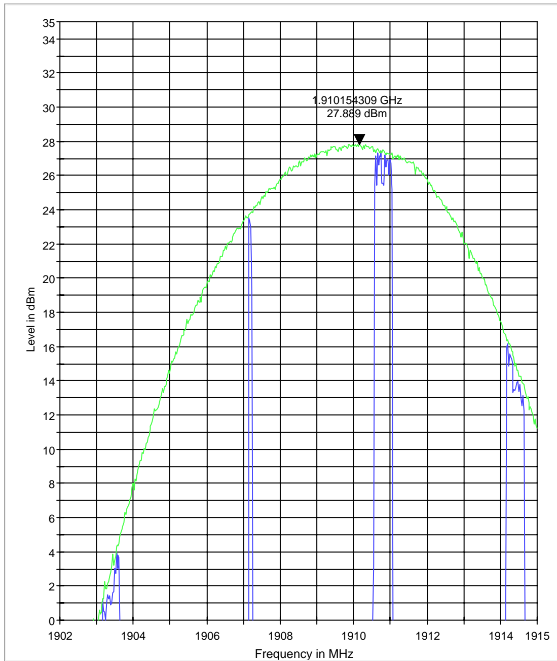
EIRP 1900 H
