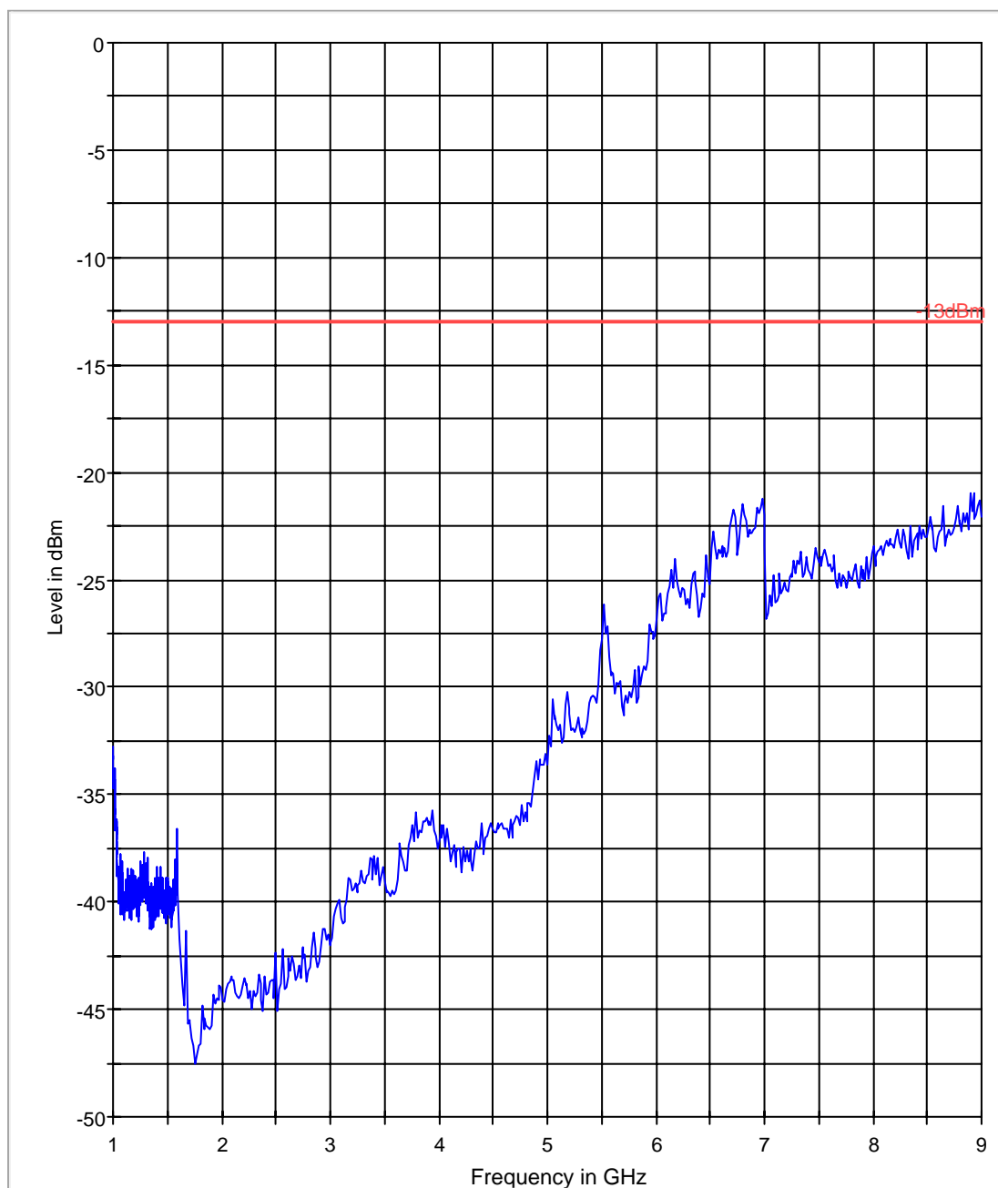
FCC 22 1-9GHz
