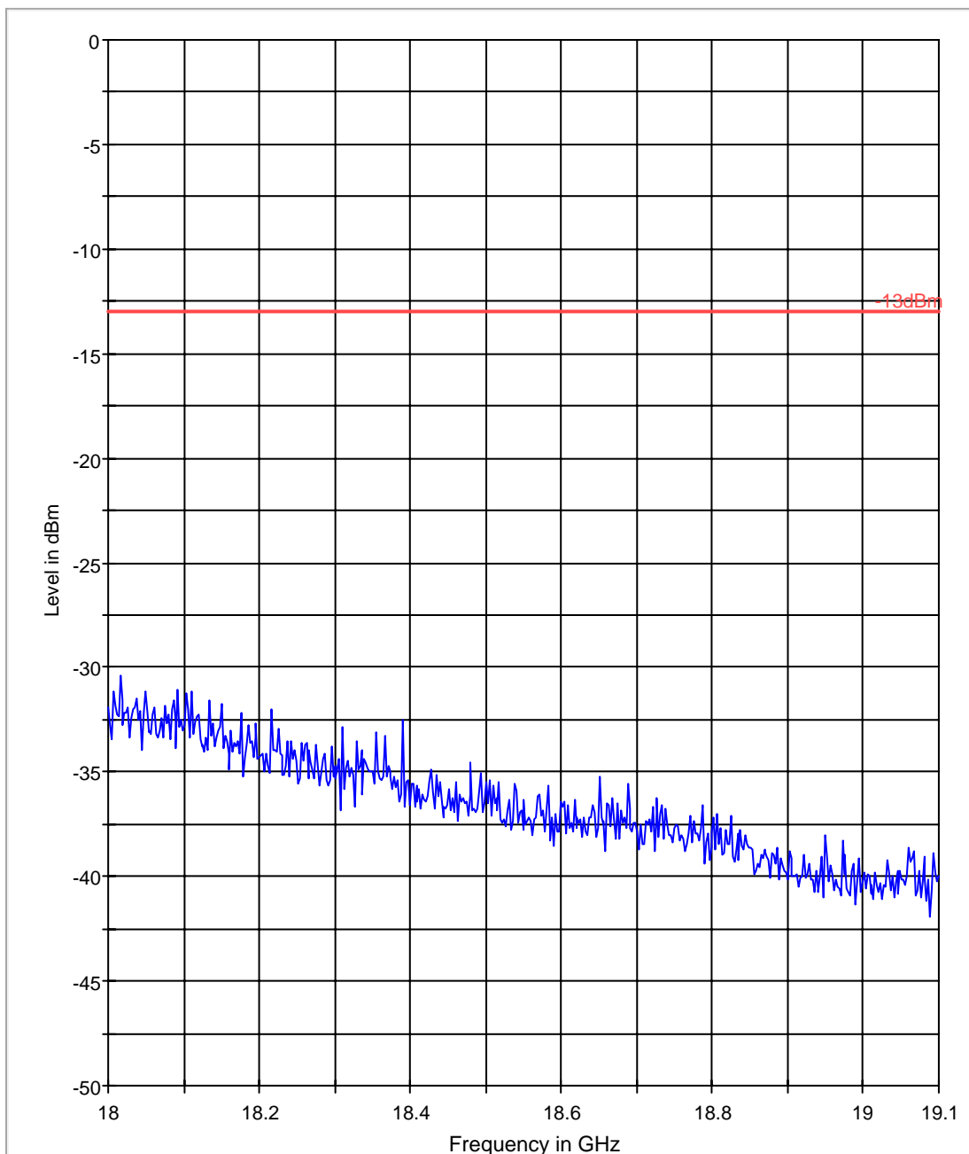
FCC 24 18-19.1GHz
