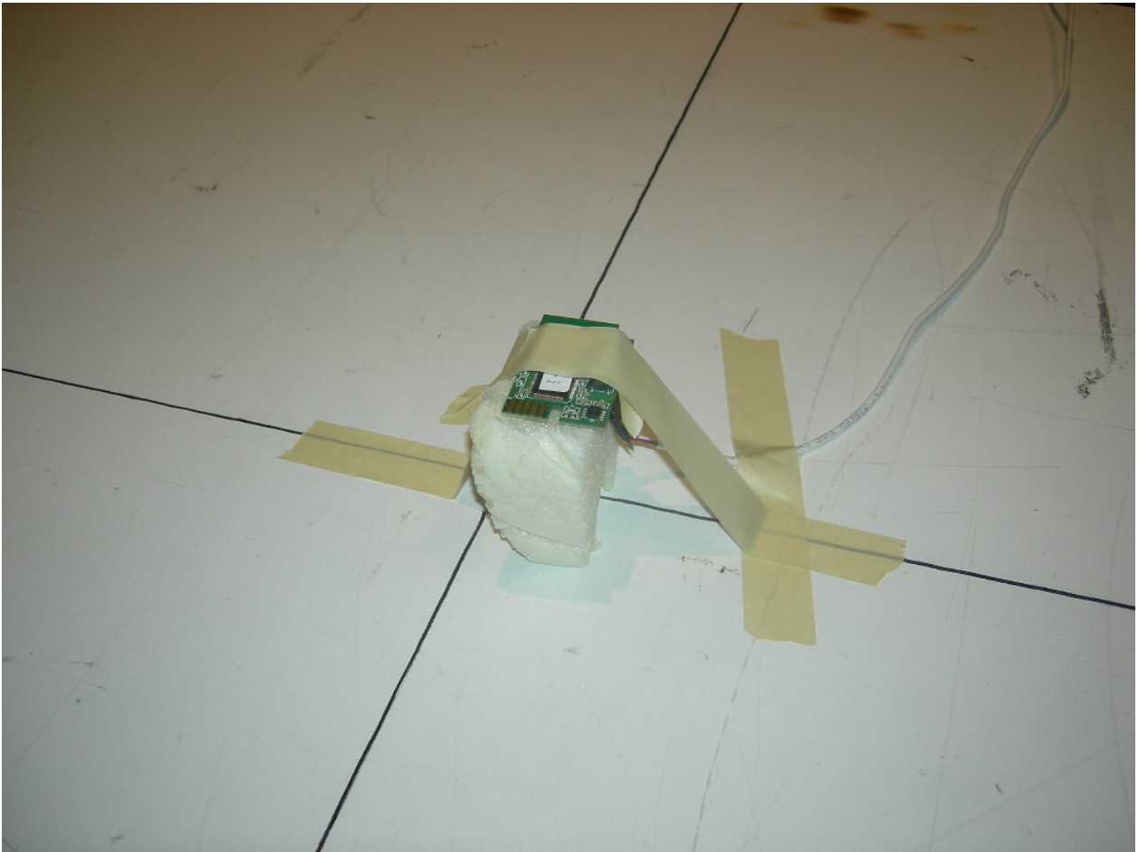
Figure 1: Radiated Emissions – Position X
