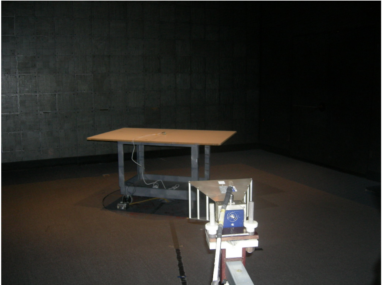
Figure 4: Radiated Emissions
