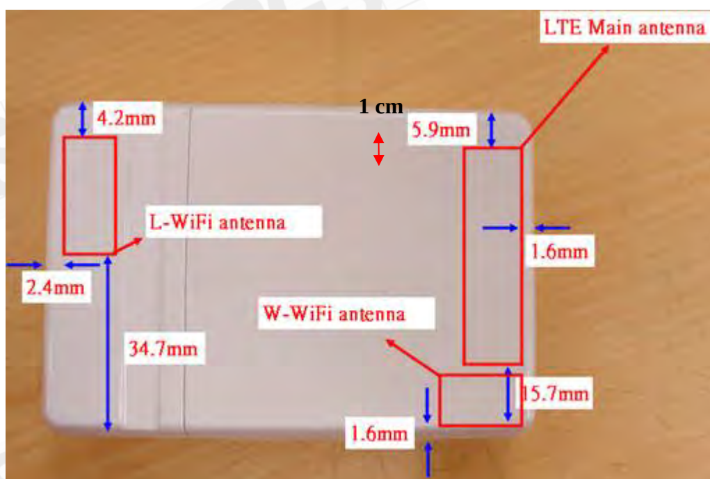
Fig.3 QD8 Antenna location & distance
