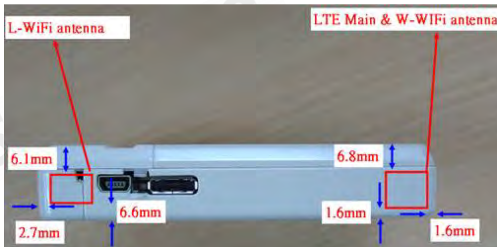
Fig.4 QD8 Antenna location & distance
