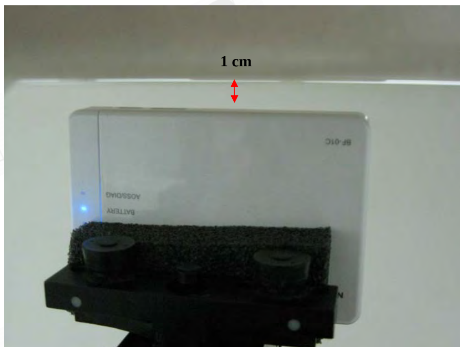
Fig.6 Bottom side to flat phantom
