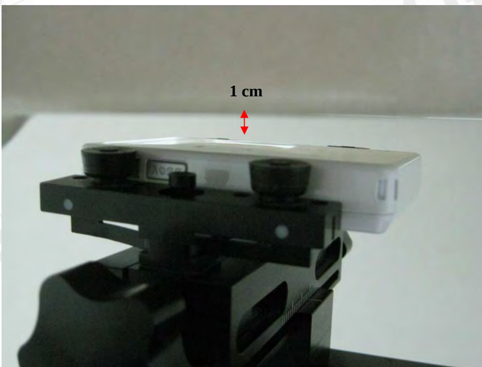
Fig.9 Front side to flat phantom
