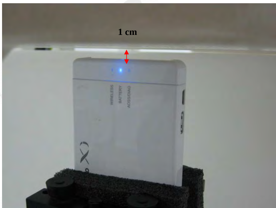
Fig.8 Right side to flat phantom
