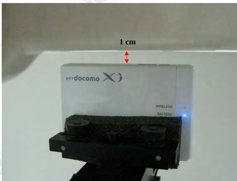
Fig.5 Top side to flat phantom
