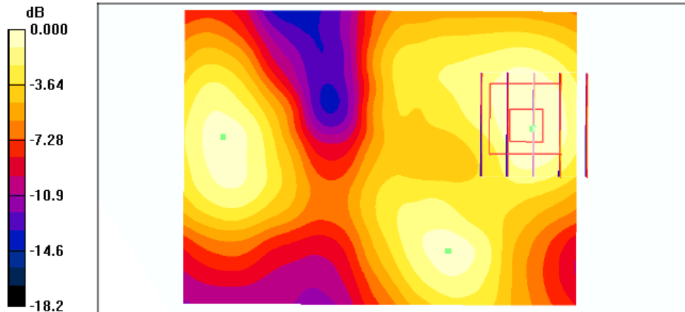
0 dB = 0.048mW/g
