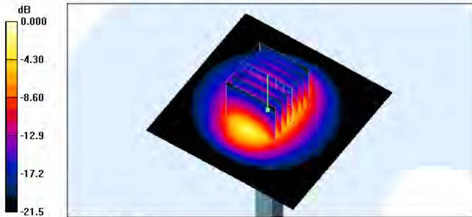
0 dB = 6.41mW/g
