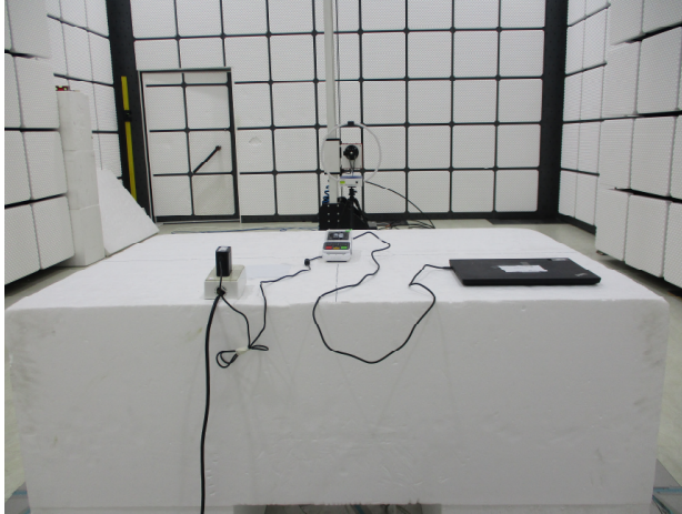
Part_15_247_BT_Radiated_Setup
