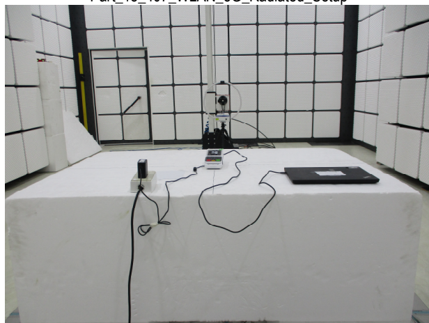
Part_15_407_WLAN_5G_Radiated_Setup
