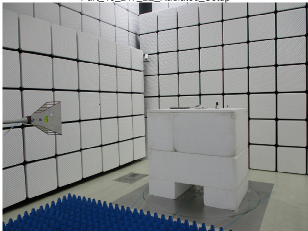
Part_15_247_LE_Radiated_Setup
