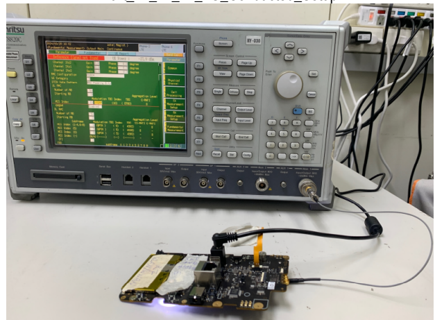
Part_22_24_27_4G_Conducted_Setup
