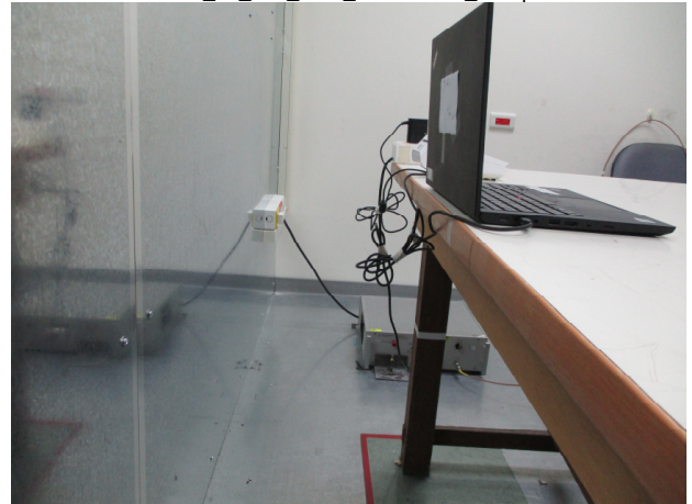
Part_15_225_NFC_Conduction_Setup
