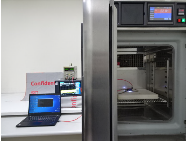
Part_15_247_BT_Conducted_Setup
