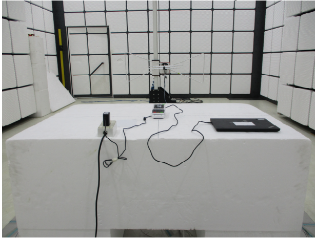
Part_15_225_NFC_Radiated_Setup
