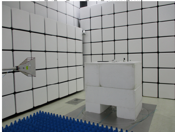
Part_15_247_WLAN_2.4G_Radiated_Setup
