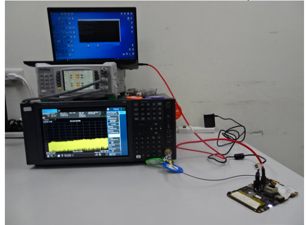
Part_15_407_WLAN_5G_Conducted_Setup
