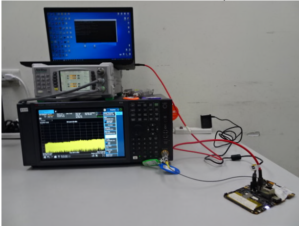
Part_15_247_LE_Conducted_Setup
