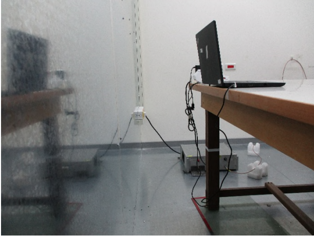
Part_15_225_NFC_Conduction_Setup
