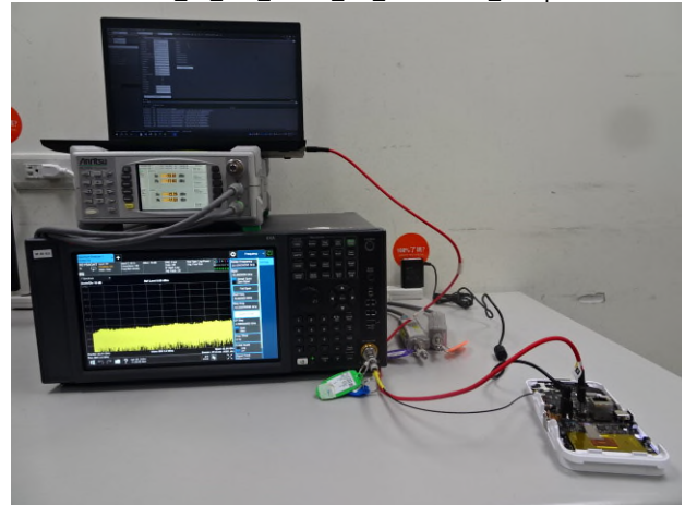
Part_15_225_NFC_Radiated_Setup
