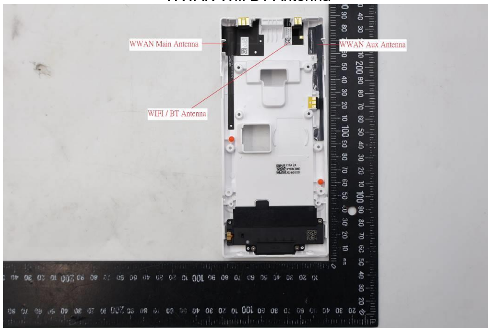
WWAN Wifi BT Antenna
