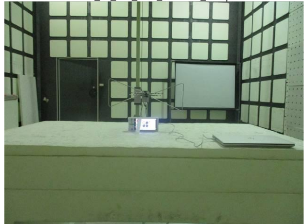
Part_15_225_NFC_Radiated_Setup
