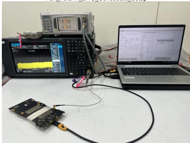
Part_15.247_BT_Conducted_Setup
