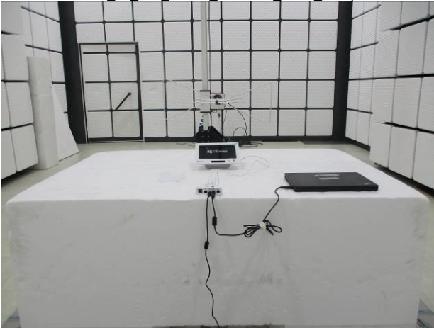
FCC_15_247_WLAN_Radiated_C505_Setup
