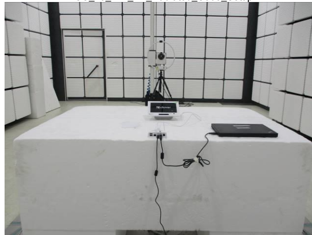
FCC_15_247_WLAN_Radiated_C305_Setup
