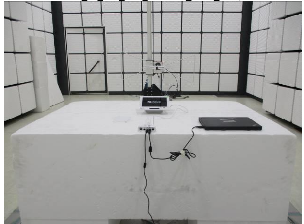
FCC_15_247_BLE_Radiated_C305_Setup
