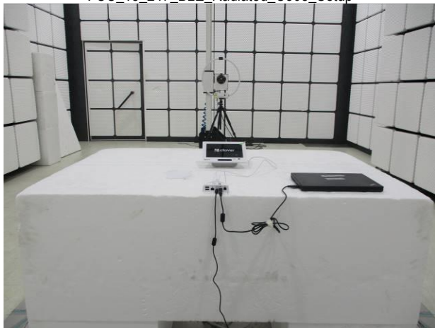
FCC_15_247_BT_Radiated_C305_Setup
