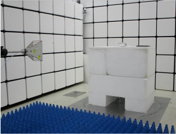
FCC_15_247_WLAN_Radiated_C305_Setup
