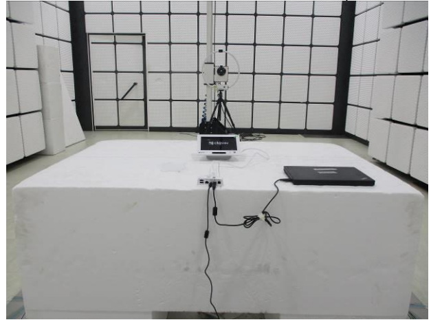
FCC_15_407_WLAN_Radiated_C505_Setup
