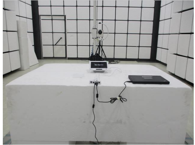
FCC_15_247_BLE_Radiated_C505_Setup
