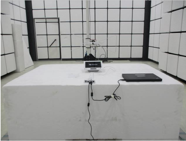
FCC_15_247_BLE_Radiated_C505_Setup
