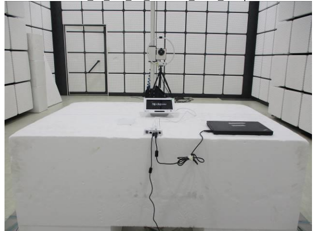
FCC_15_247_BT_Radiated_C505_Setup
