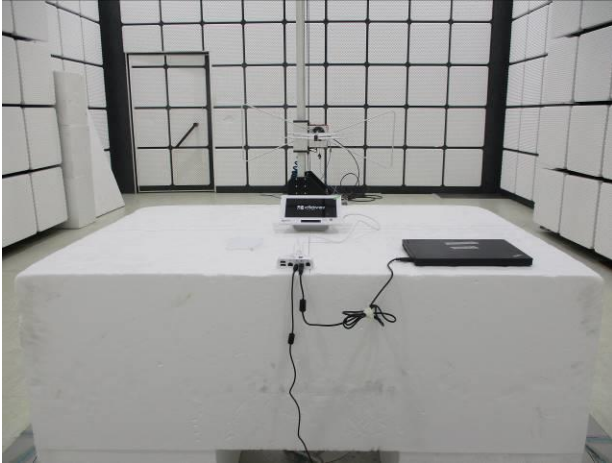
FCC_15_225_NFC_Radiated_C305_Setup
