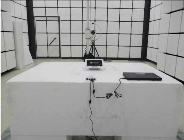
FCC_15_225_NFC_Radiated_C505_Setup
