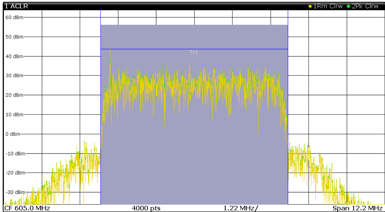
Figure 1 Plot of Antenna Port Power Output
