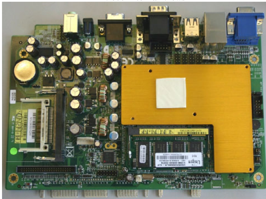
Figure 5 - MPT9600 CPU Board Top View
