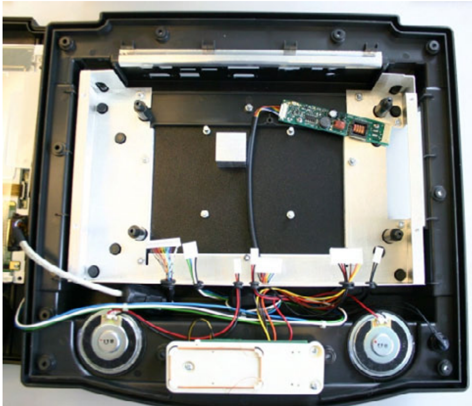
Figure 16 - MPT9600 Backlight Inverter Location
