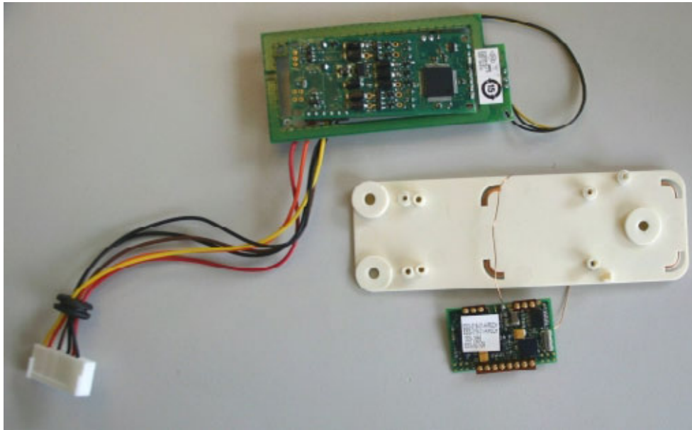
Figure 11 - MPT9600 HID Sub-Assembly
