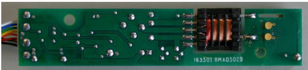
Figure 18 - MPT9600 Backlight Inverter Bottom View
