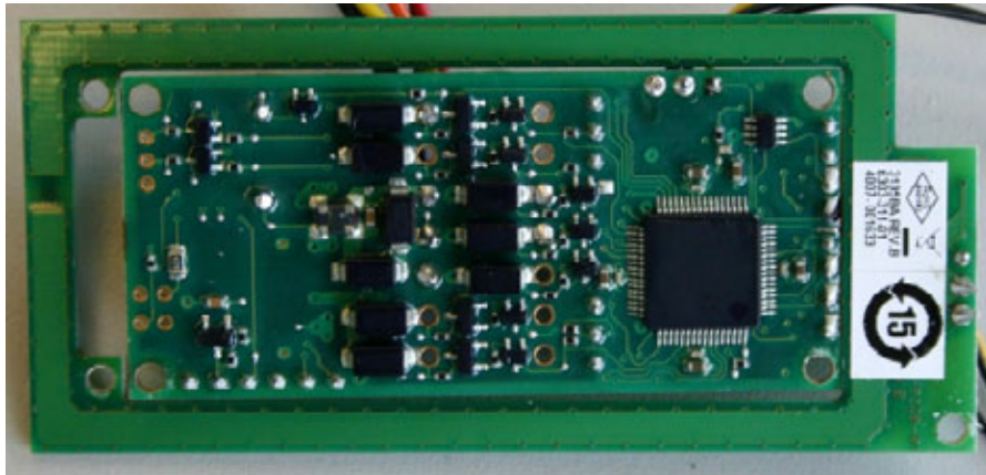
Figure 13 - MPT9600 HID Main Board – Bottom View
