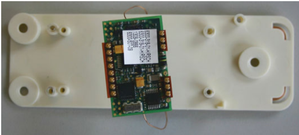
Figure 15 - MPT9600 HID Top Board – Top View
