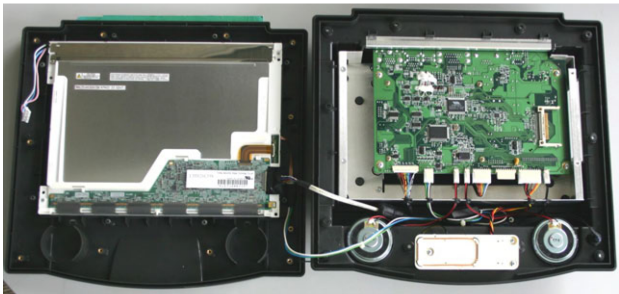
Figure 2 - MPT9600 Cable and Board Layout
