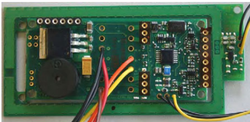
Figure 12 - MPT9600 HID Main Board – Top View
