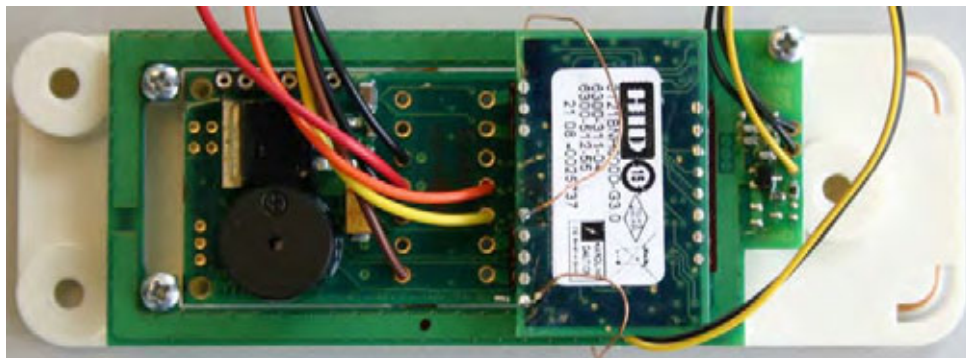
Figure 9 - MPT9600 HID Assembly
