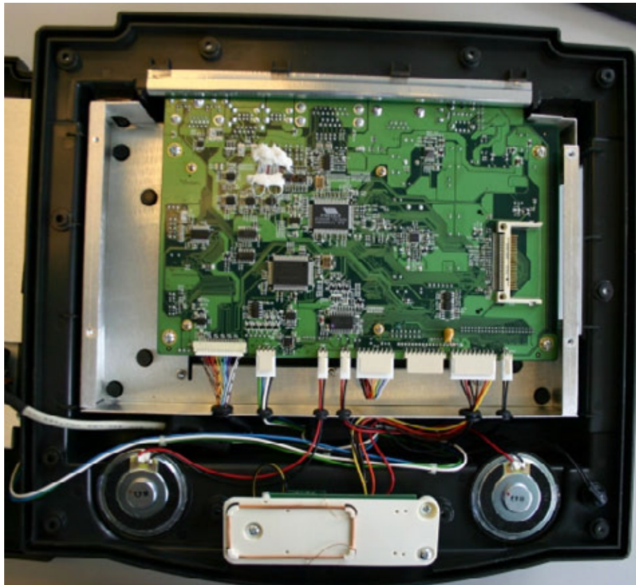
Figure 3 - MPT9600 Cable and Board Layout
