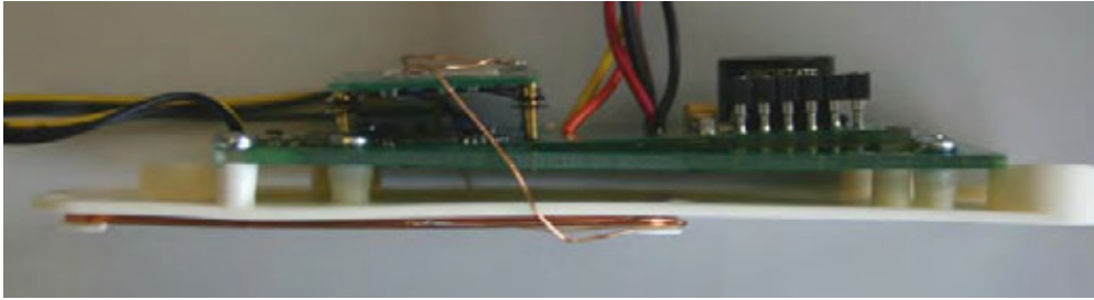
Figure 10 - MPT9600 HID Assembly Side View
