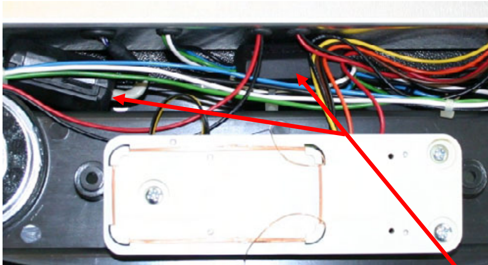
Figure 7 - MPT9600 Ferrite Chokes and HID reader
