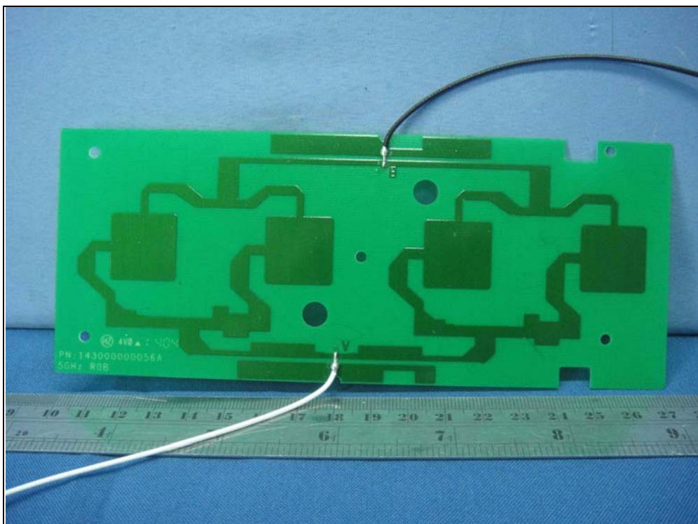
Internal antenna 3 (Brand Name: Accton / Model Name: OAP1232RL-FLF-EC)
