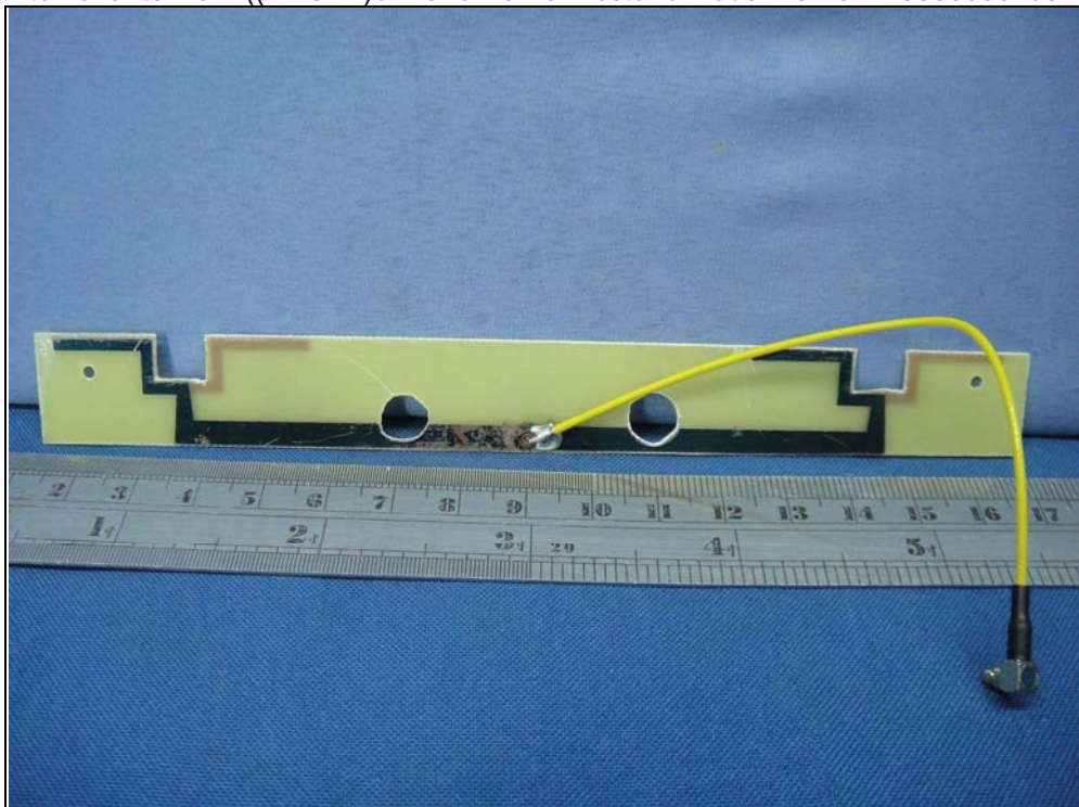
Internal antenna 2 ((2.4GHz) / Brand Name: Accton / Model Name: 123800000295A)
