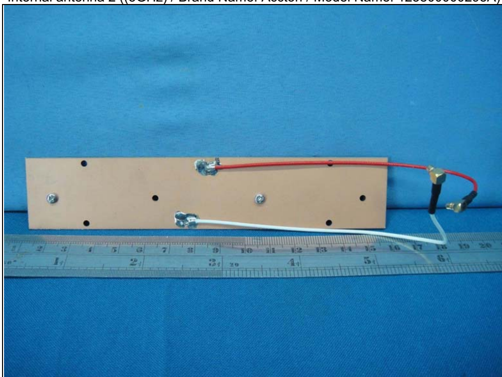
Internal antenna 2 ((5GHz) / Brand Name: Accton / Model Name: 123800000295A)
