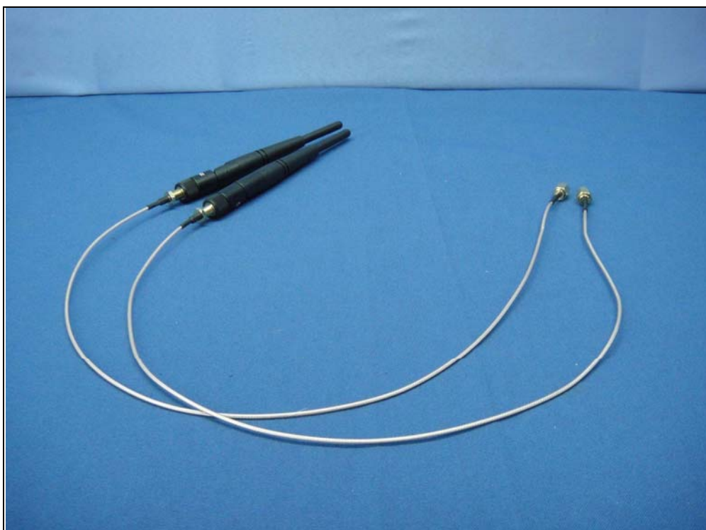
External Antenna 2 (Brand Name: Cortec / Model Name: AN5000-0301RS)
