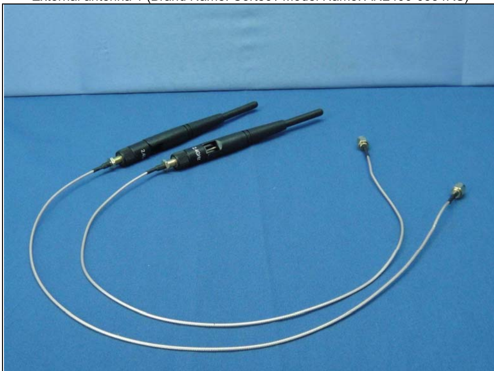
External antenna 1 (Brand Name: Cortec / Model Name: AN2400-0334RS)
