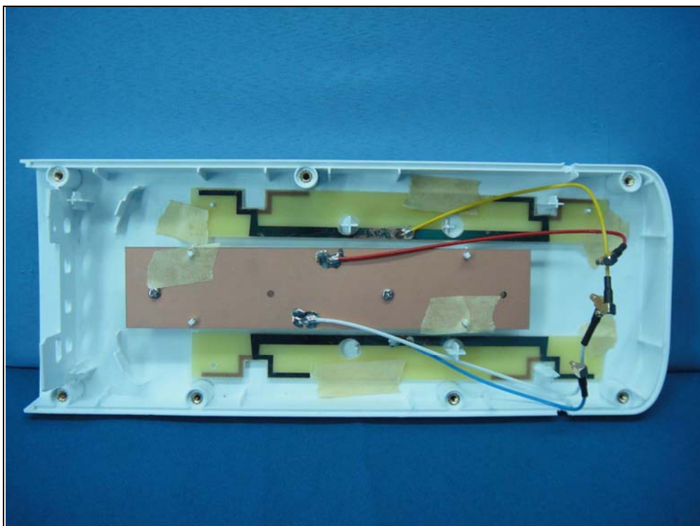
Internal Antenna 2 ((2.4GHz & 5GHz) / Brand Name: Accton / Model Name: 123800000295A)
