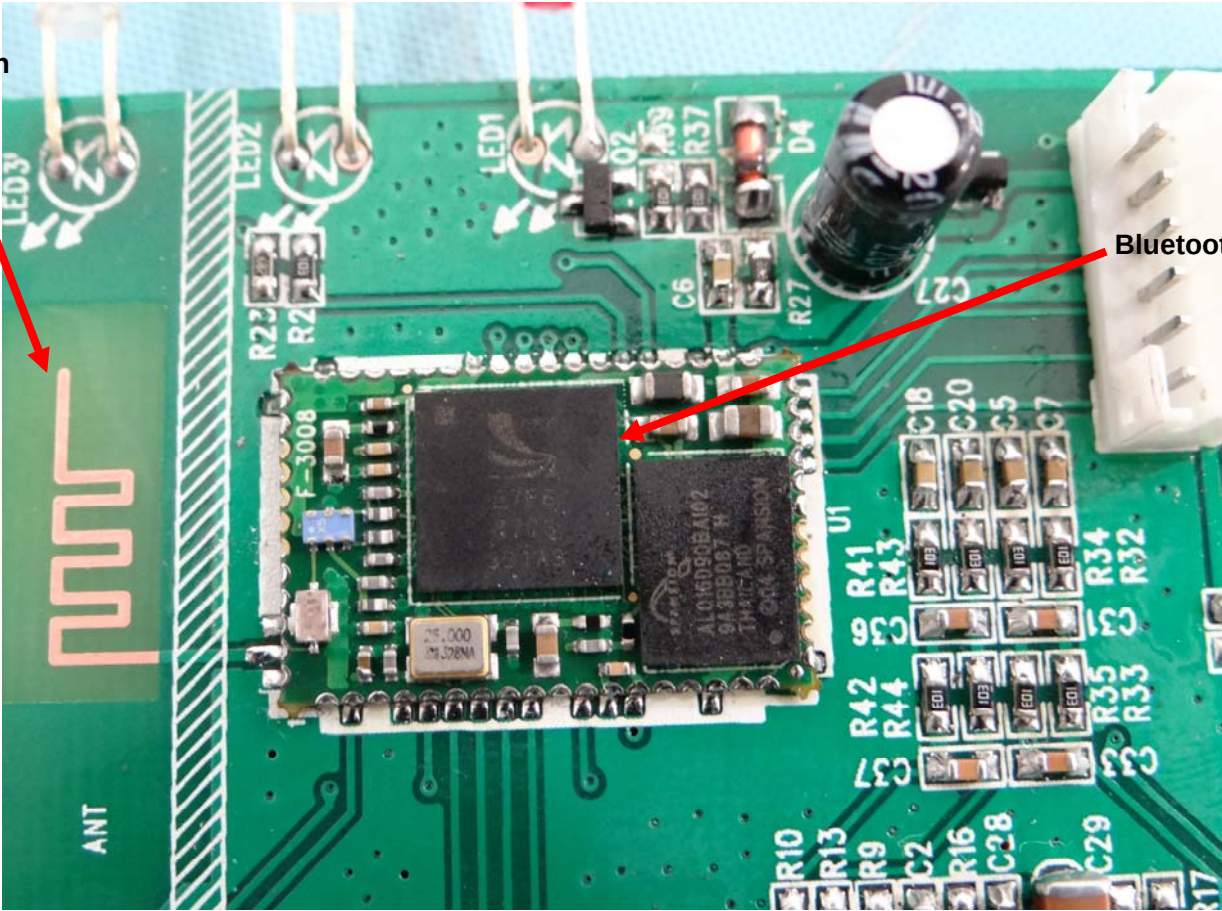
Bluetooth Antenna
