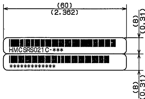
N+1/4in4out Subrack BARCODE LABEL
