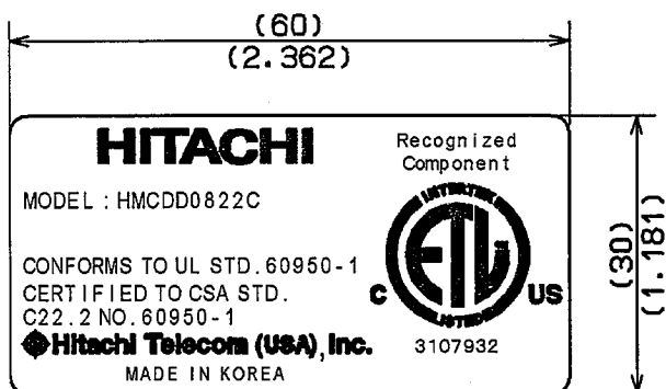
4X2 Tray(850M) MAIN LABEL
