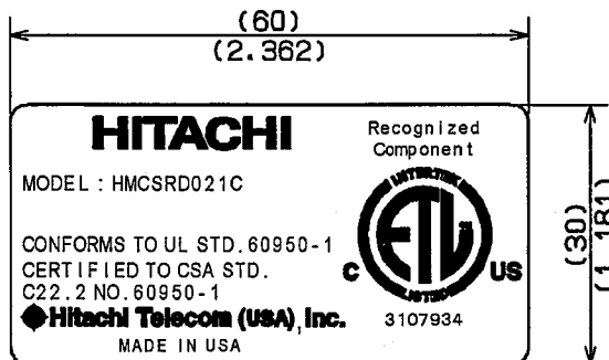
4x2 Subrack MAIN LABEL
