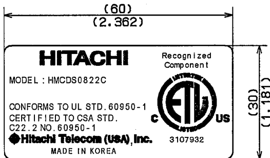
N+1/4in4out Tray(850M) MAIN LABEL
