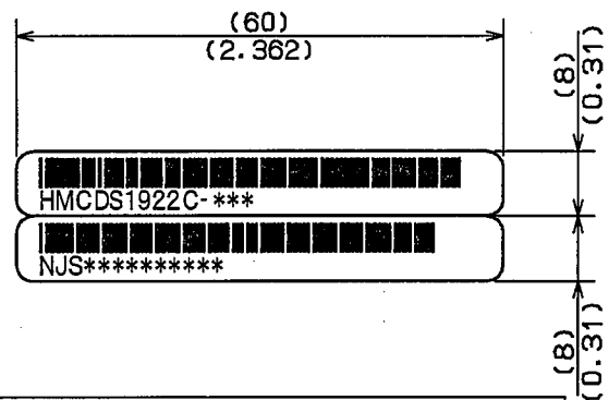
N+1/4in4out Tray(1900M) Barcode LABEL
