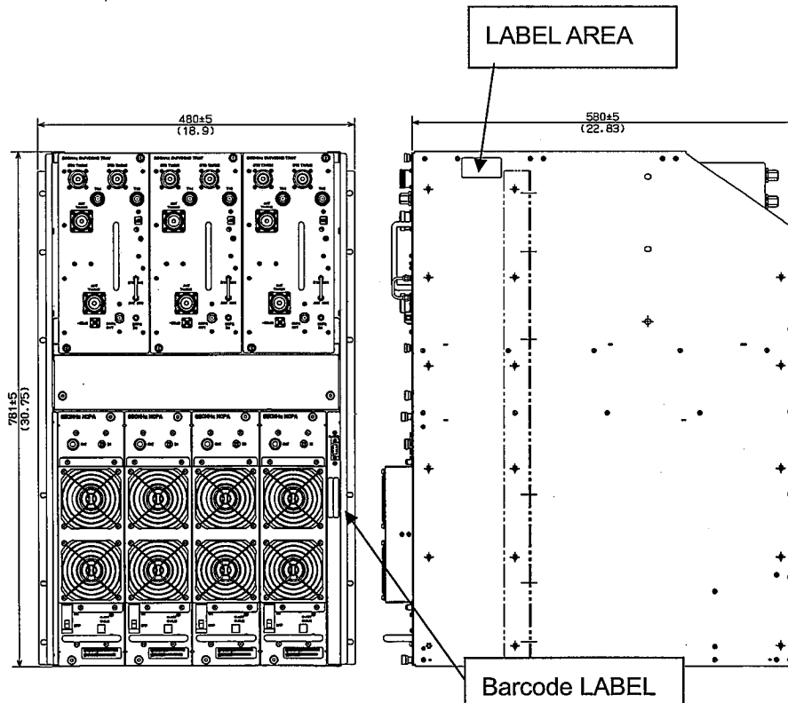
4in4out Subrack Appearance DWG.
