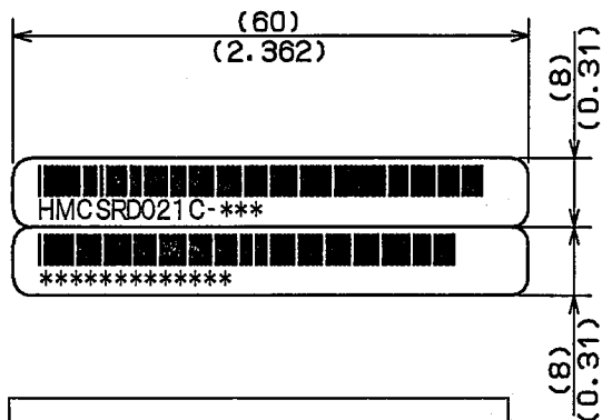
4x2 Subrack BARCODE LABEL
