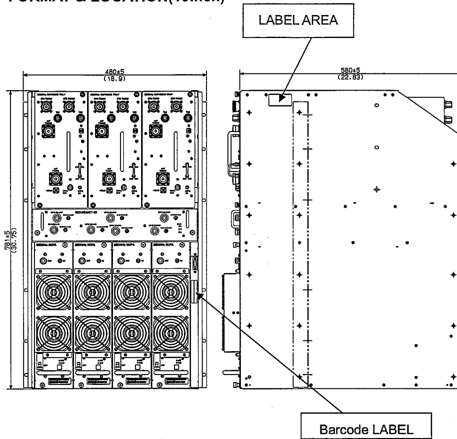
19in.N+1 Subrack Appearance DWG.
