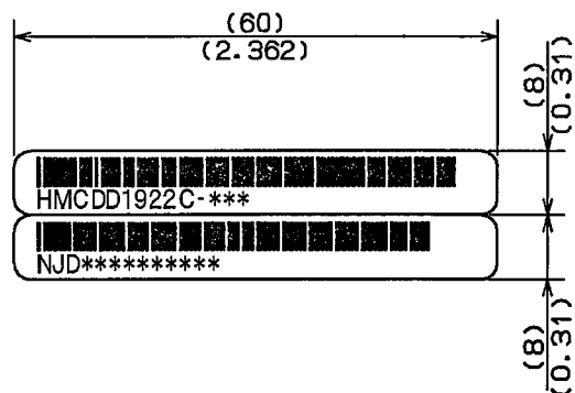
4X2t Tray(1900M) Barcode LABEL
