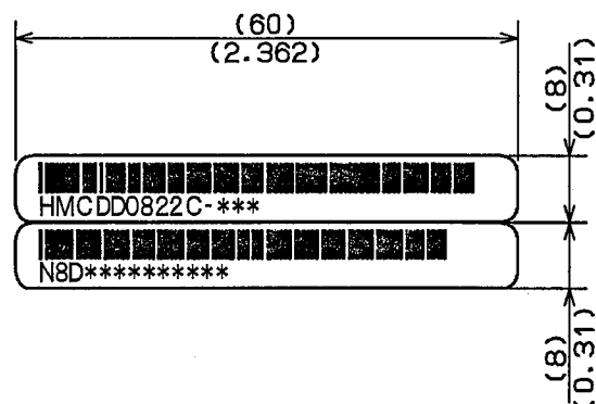
4X2 Tray(850M) Barcode LABEL
