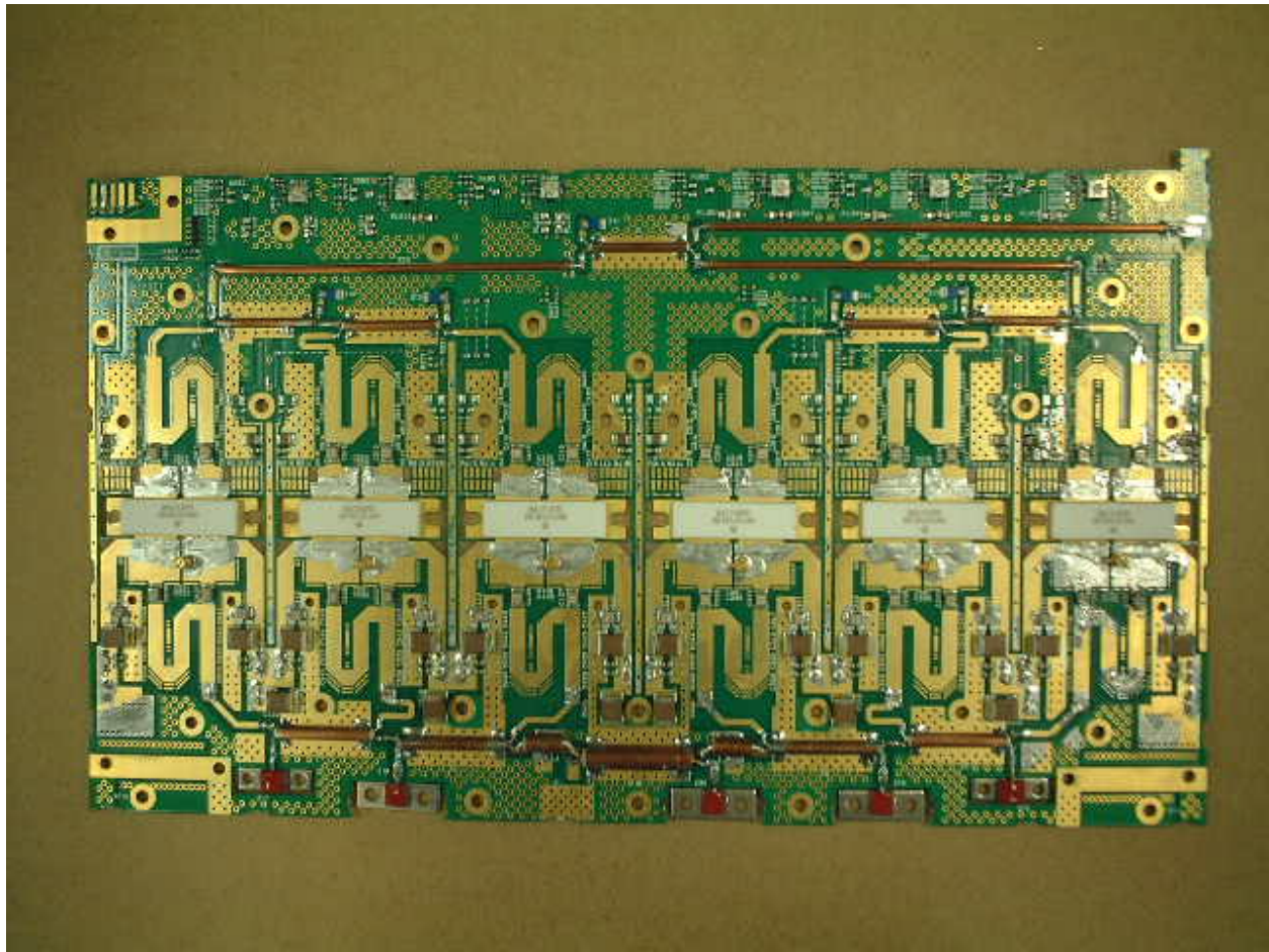
Figure 10: Main Board Side A
