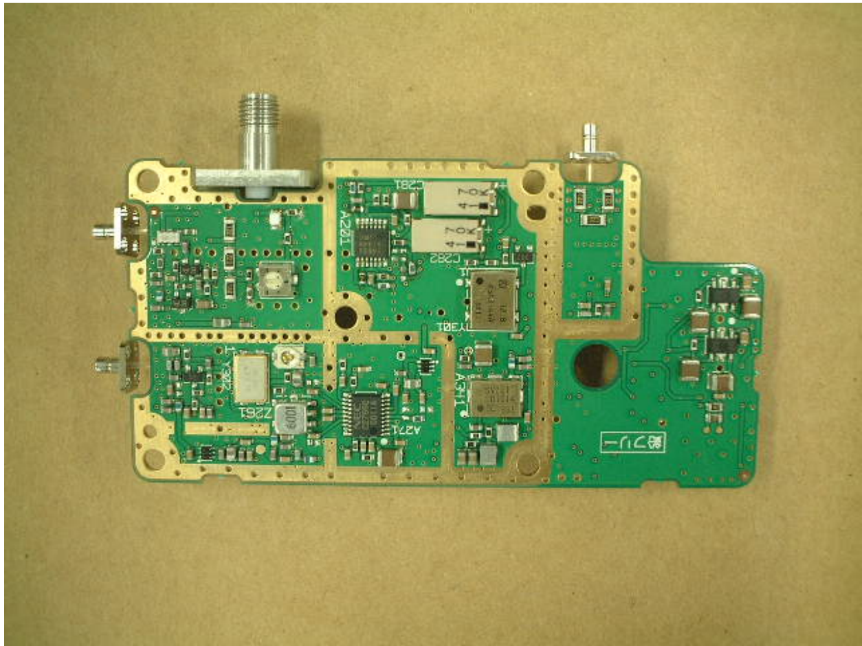
Figure 17: RX B1
