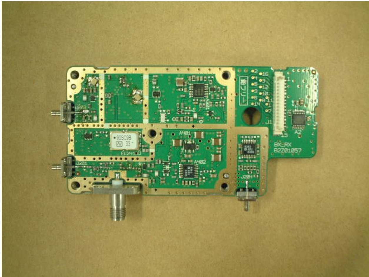
Figure 15: RX A1
