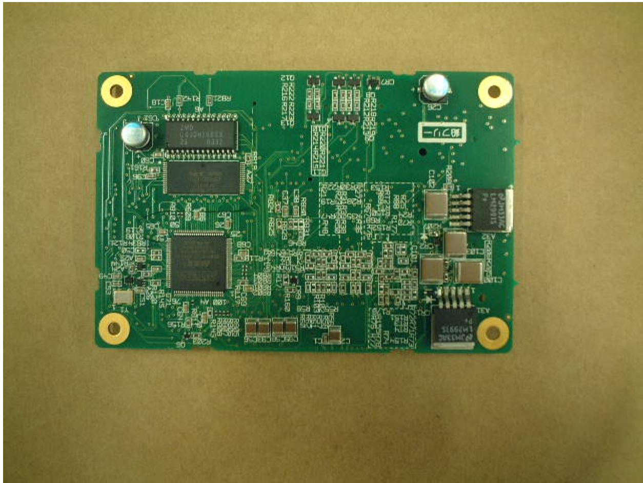
Figure 2: Cont Side B
