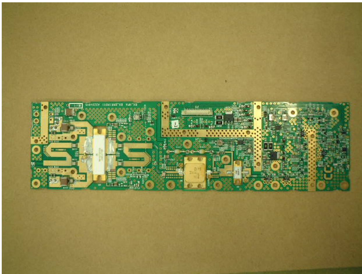
Figure 5: ERR Side A
