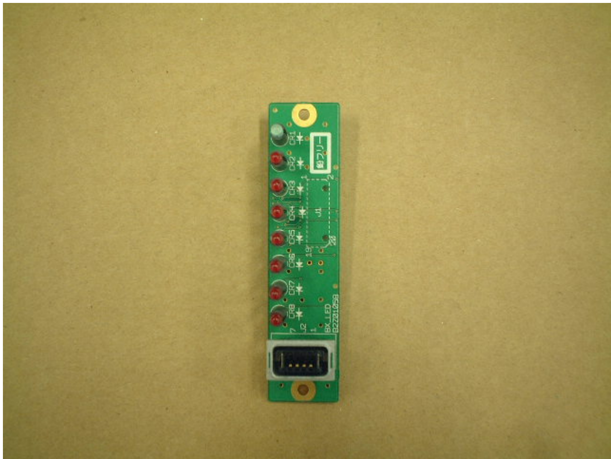
Figure 8: LED Board Side A
