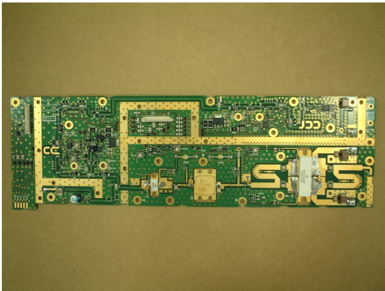
Figure 3: DRV Side A
