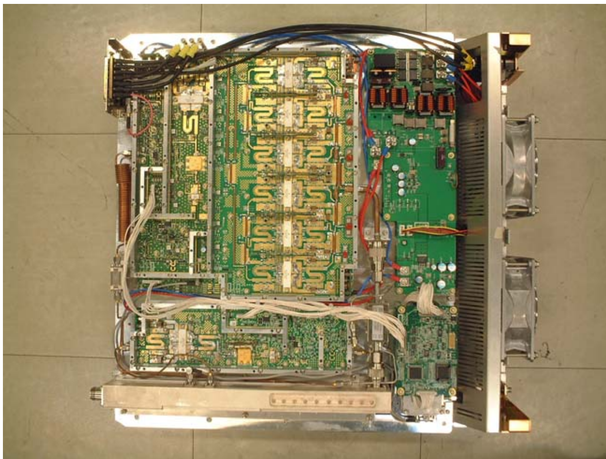
Figure 12: MCPA Assembly, cover and heat sink removed
