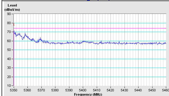
Bandedge (PK)
