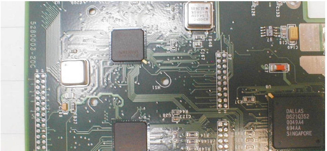
Baseband Board Top, Detail B
