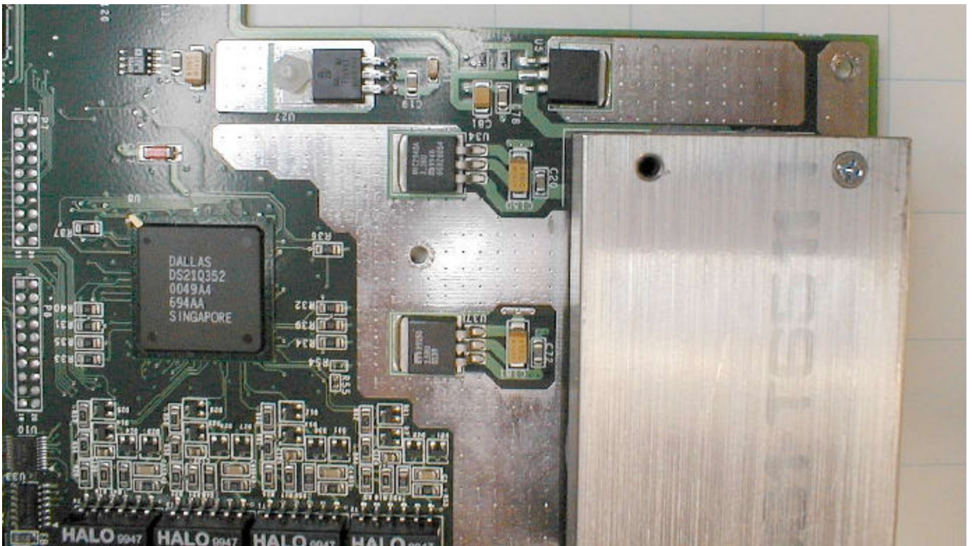
Baseband Board Top, Detail D
