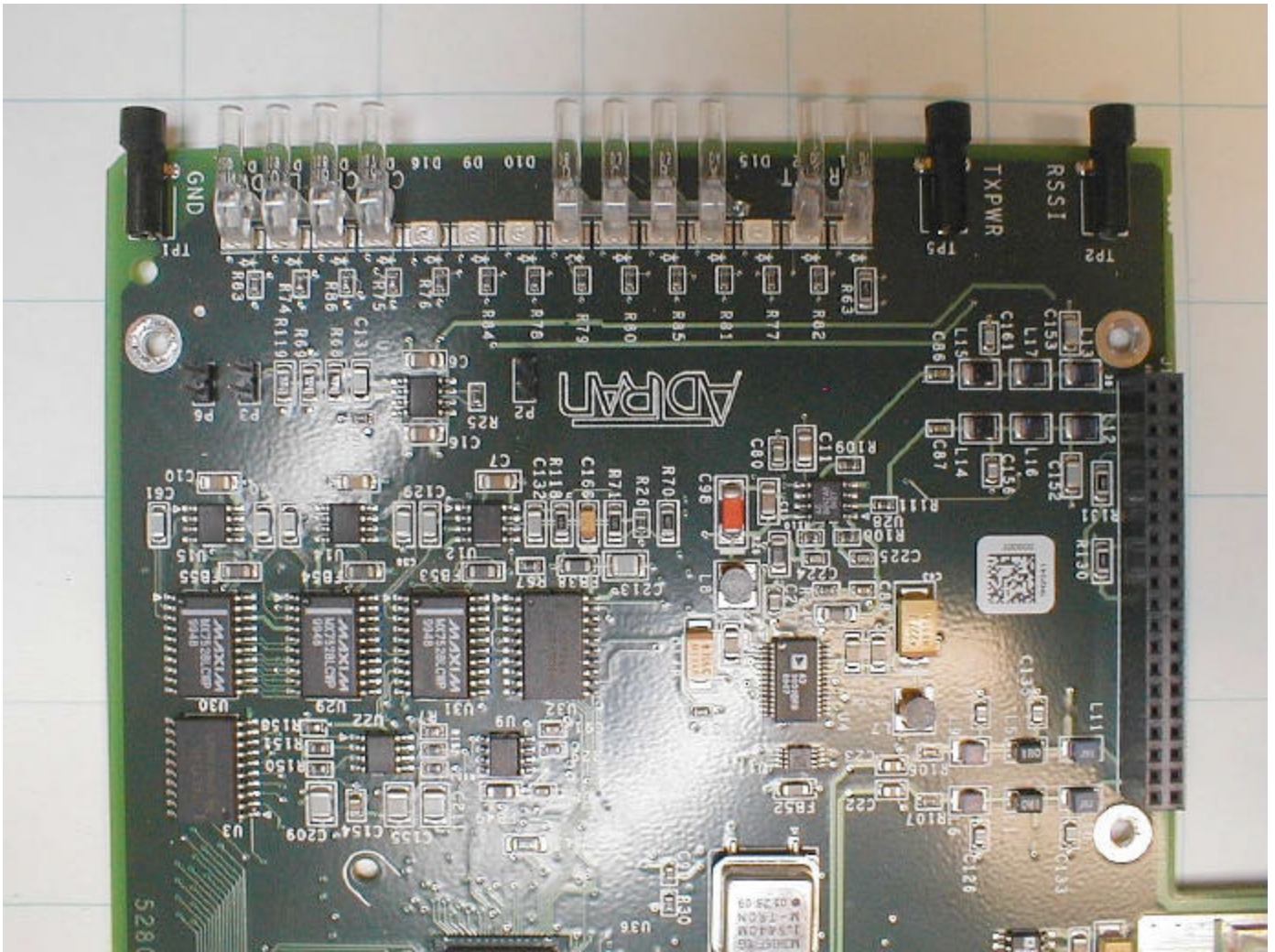
Baseband Board Top, Detail A
