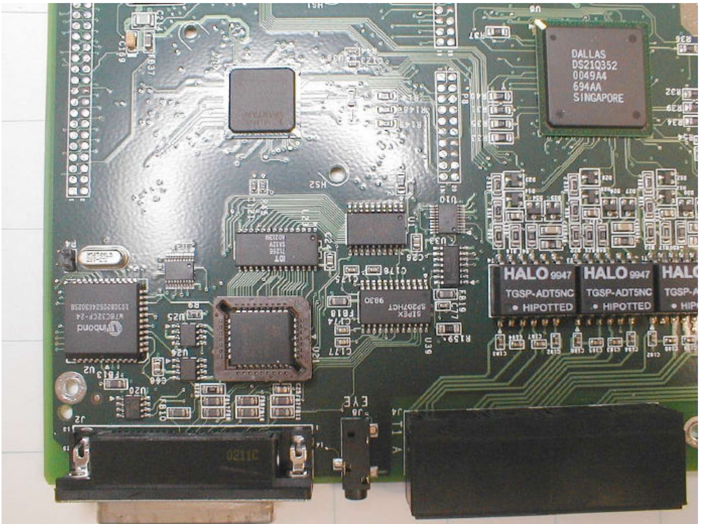
Baseband Board Top, Detail D
