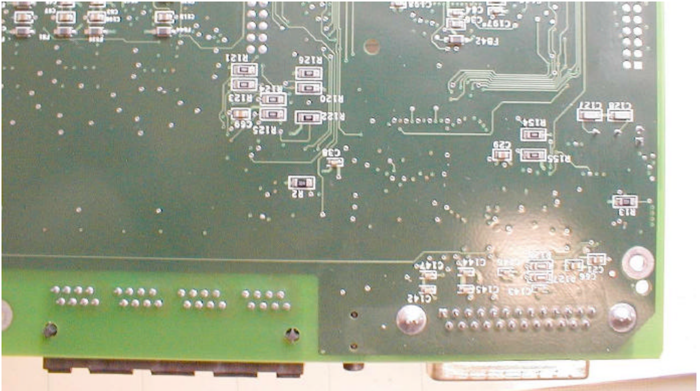
Baseband Board Bottom, Detail C
