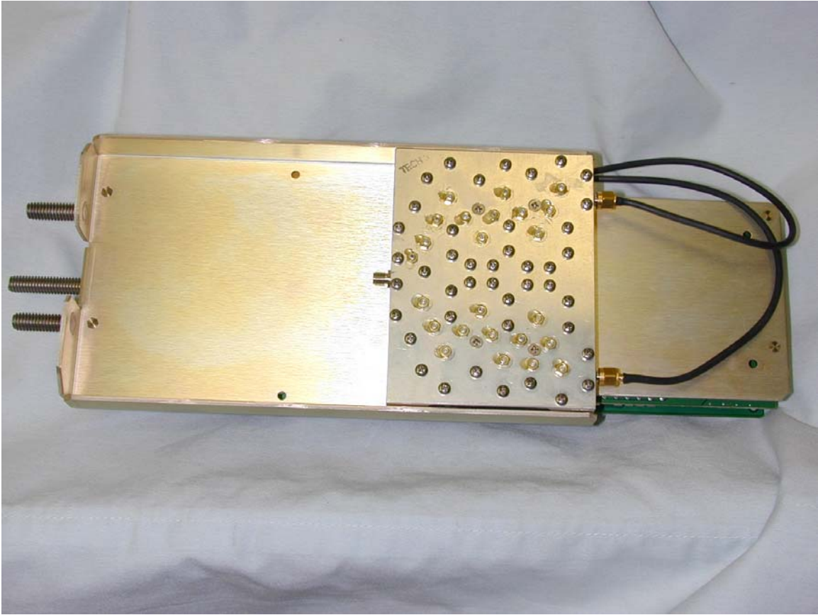
Bottom of Canister Boards
