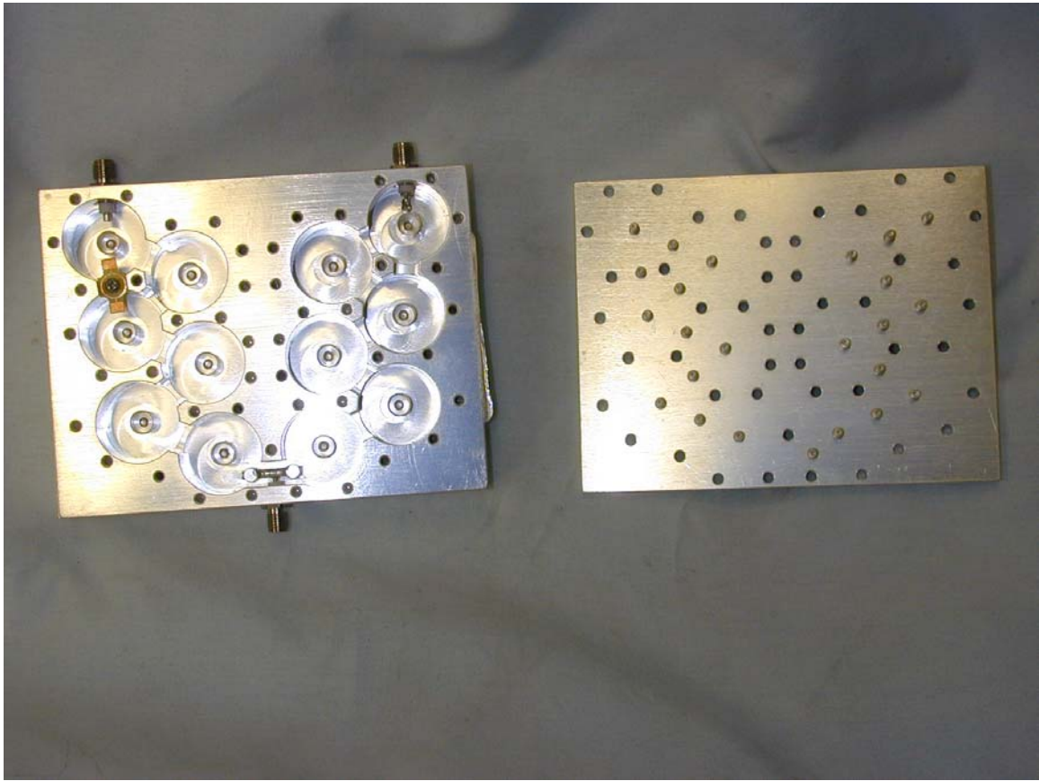
Internal Space Tuner
