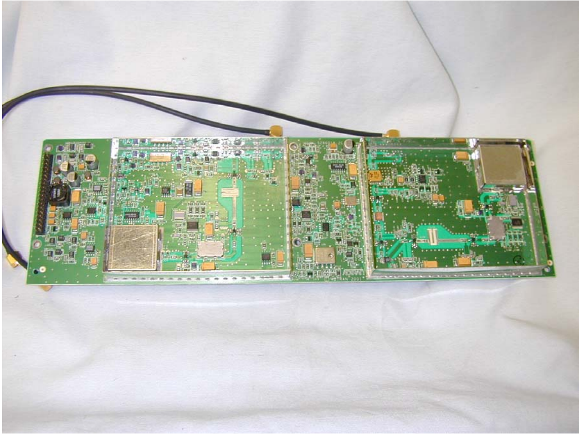
Canister Board With Small Shields
