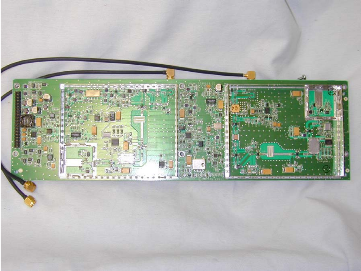
Canister Board Without Shields
