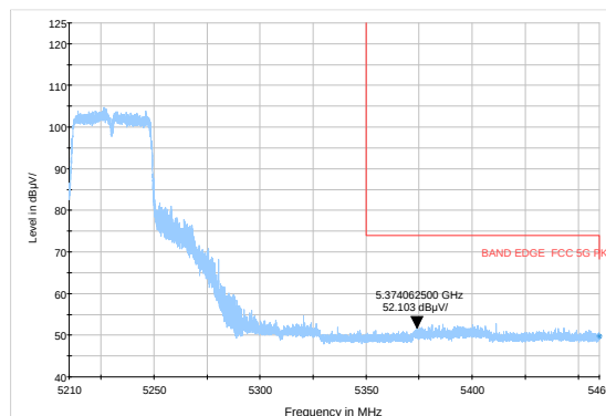
802.11ac HT40-Channel 46: Average
