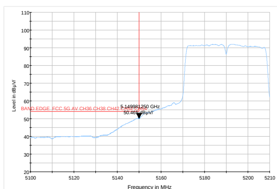
802.11ac HT40-Channel 38: Average
