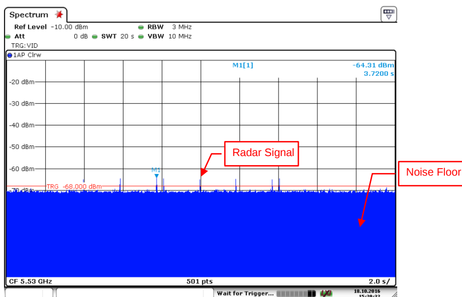
Single Burst of Radar Signal 4
