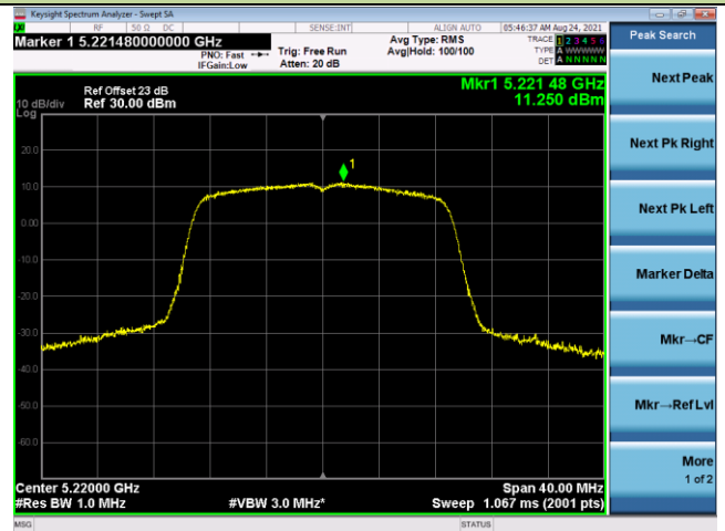
Channel 44 (5220MHz)
