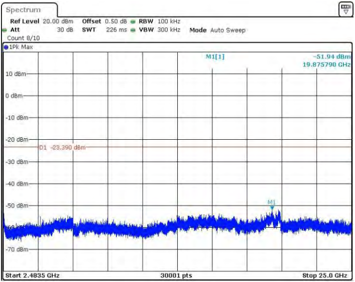
11B_Ant4_2437_2483.5~25000
