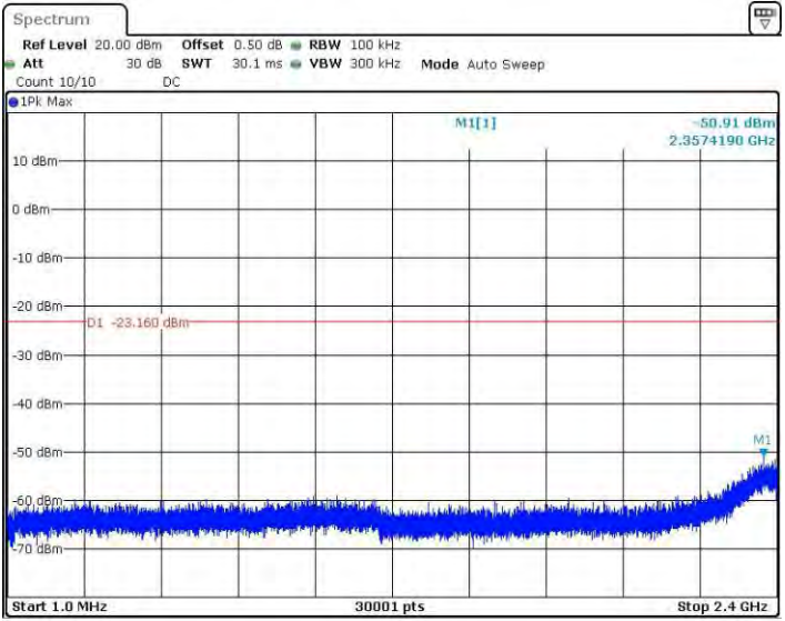
11B_Ant3_2462_1~2400
