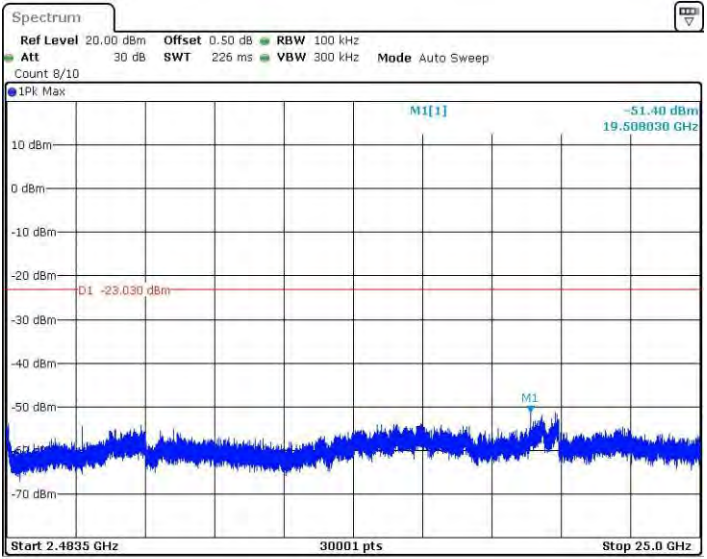
11B_Ant4_2462_2483.5~25000
