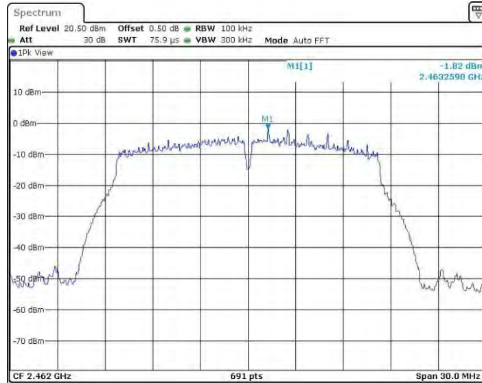
11G_Ant3_2462_0~Reference
