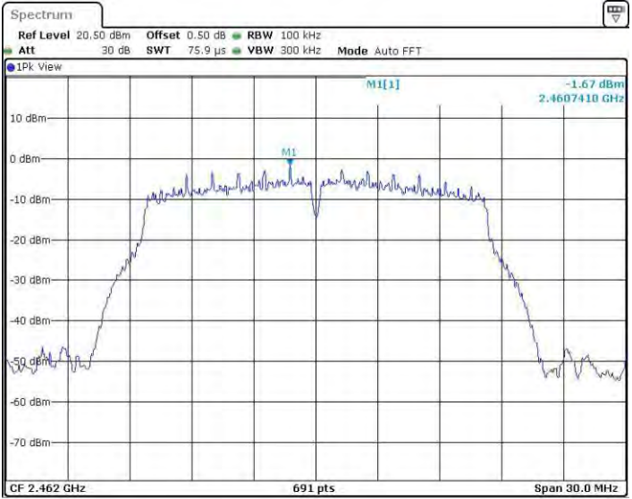
11GMINO_Ant3_2462_0-Reference
