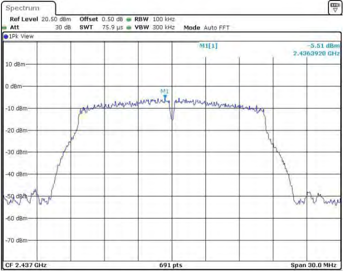
11G_Ant3_2437_0~Reference
