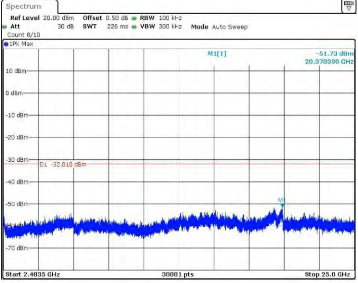
11G_Ant3_2412_2483.5~25000
