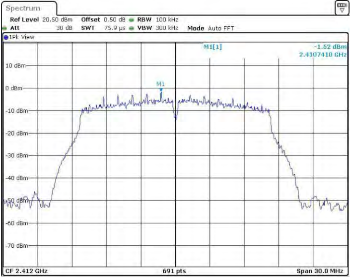
11G_Ant2_2412_0~Reference
