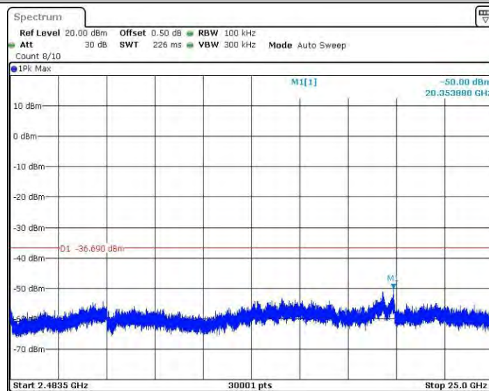
11N40SISO_Ant4_2452_2483.5~25000
