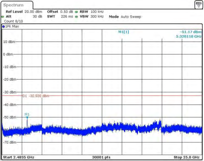
11N20SISO_Ant4_2437_2483.5~25000
