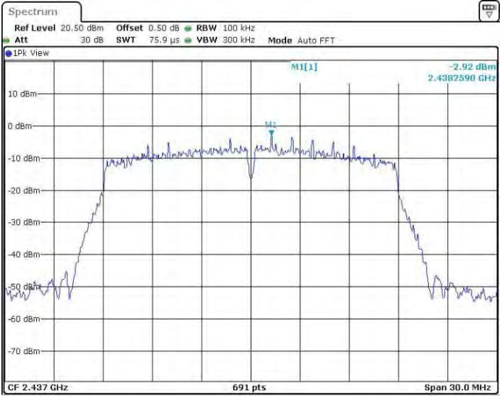
11N20SISO_Ant4_2437_0~Reference
