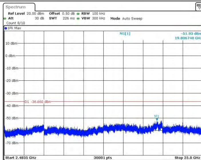
11N40SISO_Ant3_2437_2483.5~25000
