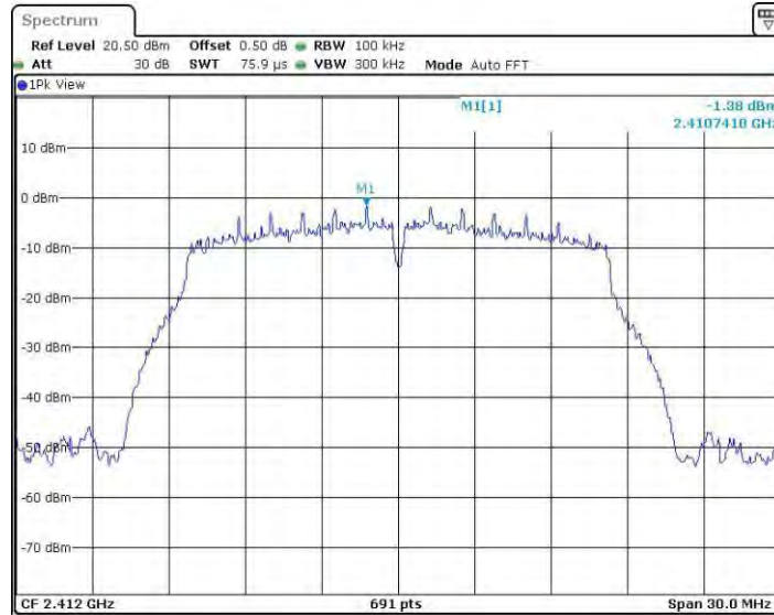
11G_Ant4_2412_0~Reference
