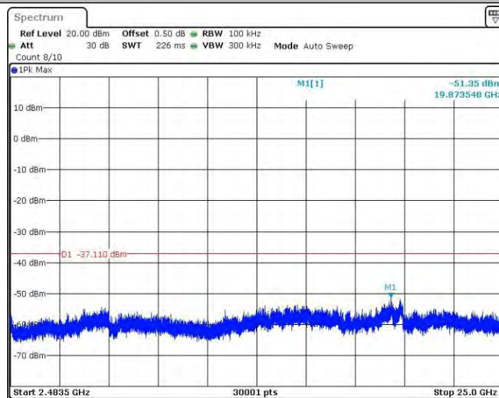
11N40SISO_Ant3_2422_1~2400
