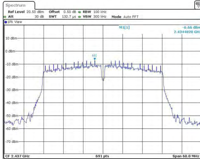
11N40SISO_Ant3_2437_0~Reference
