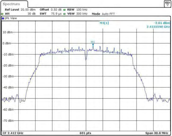
11G_Ant3_2412_0~Reference
