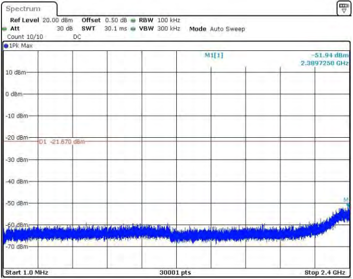
11GMINO_Ant3_2462_1~2400
