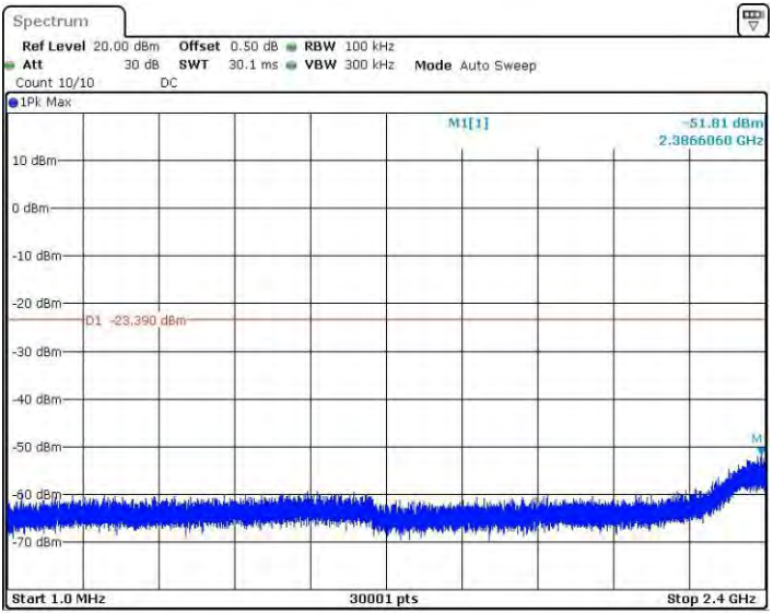
11B_Ant4_2437_1~2400
