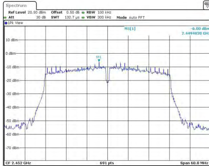
11N40SISO_Ant3_2452_0~Reference
