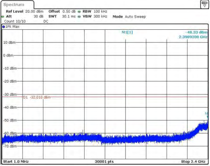
11G_Ant3_2412_1~2400
