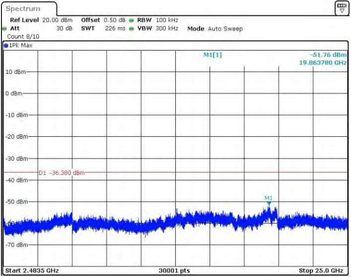
11N40SISO_Ant4_2422_2483.5~25000
