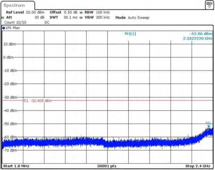
11G_Ant2_2437_1~2400
