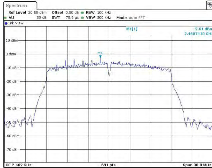
11N20SISO_Ant4_2462_0~Reference
