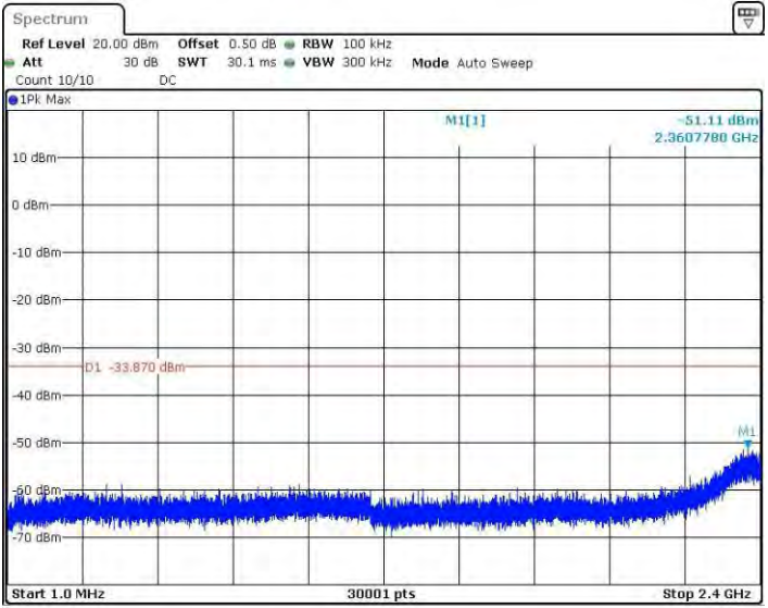
11N20SISO_Ant3_2462_1~2400
