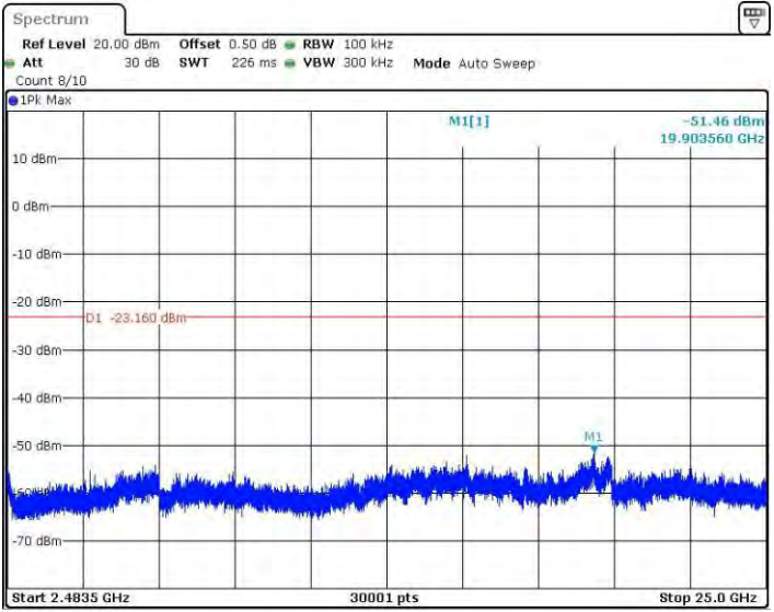
11B_Ant3_2462_2483.5~25000
