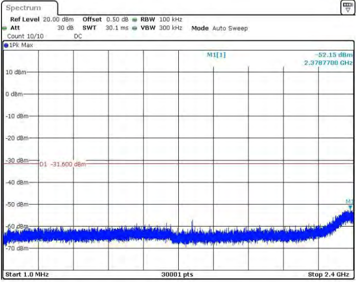
11G_Ant4_2462_1~2400
