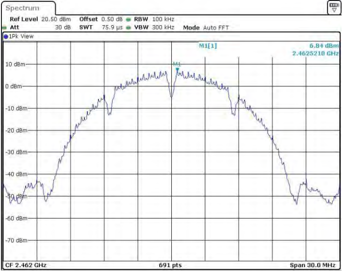
11B_Ant3_2462_0~Reference
