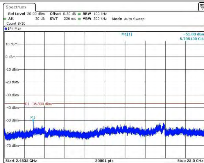
11N40SISO_Ant4_2437_2483.5~25000
