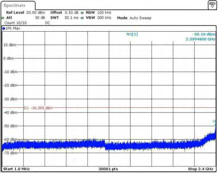
11N40SISO_Ant4_2422_1~2400
