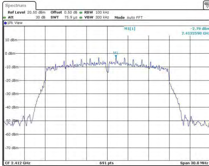
11N20SISO_Ant2_2412_0~Reference
