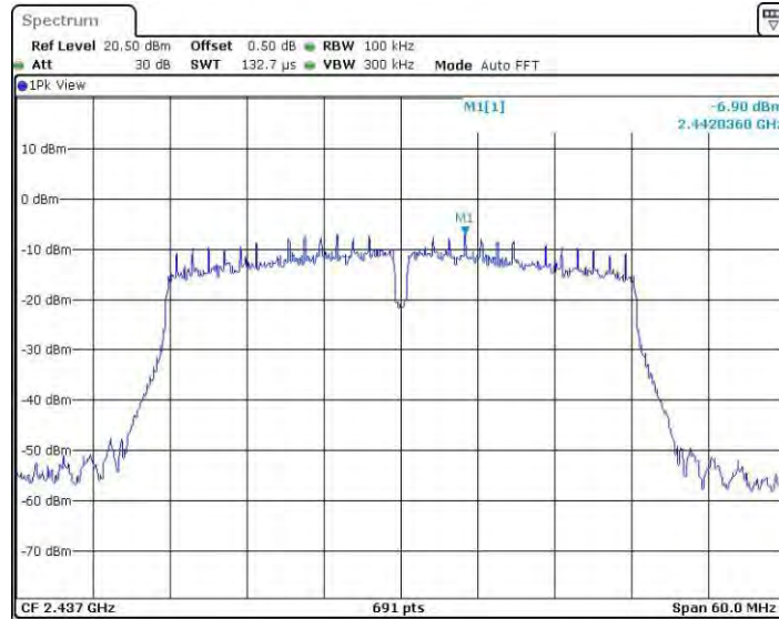
11N40SISO_Ant4_2437_0~Reference
