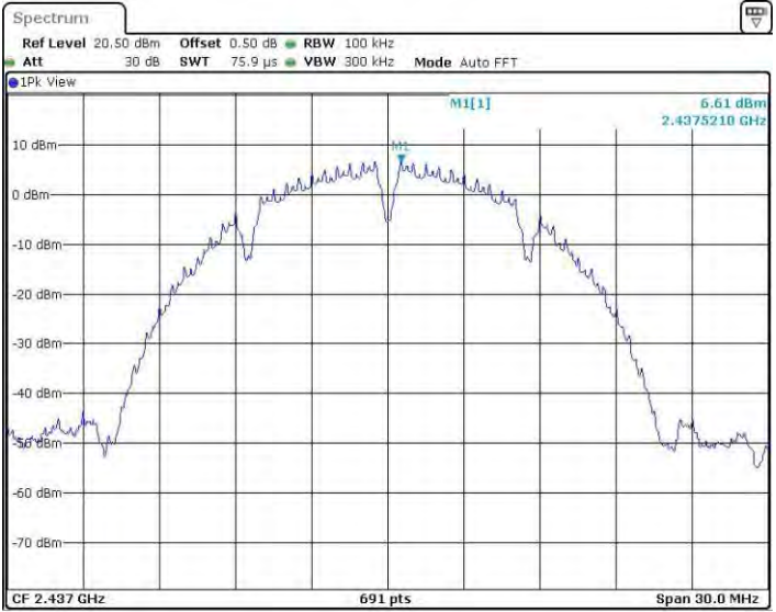
11B_Ant4_2437_0-Reference
