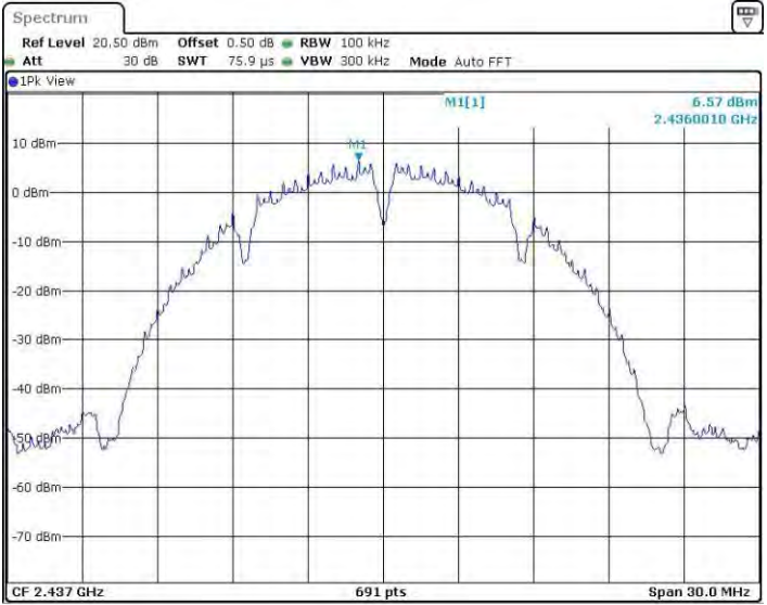
11B_Ant3_2437_0~Reference
