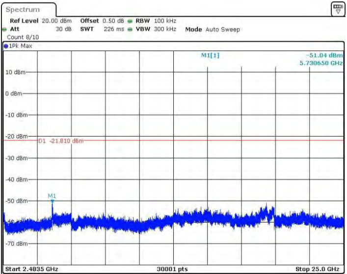
11GMINO_Ant4_2437_2483.5~25000
