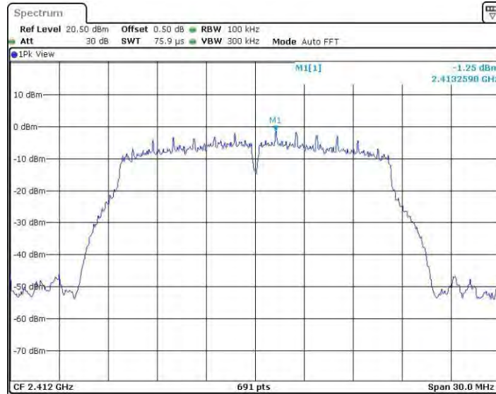
11GMINO_Ant4_2412_0~Reference
