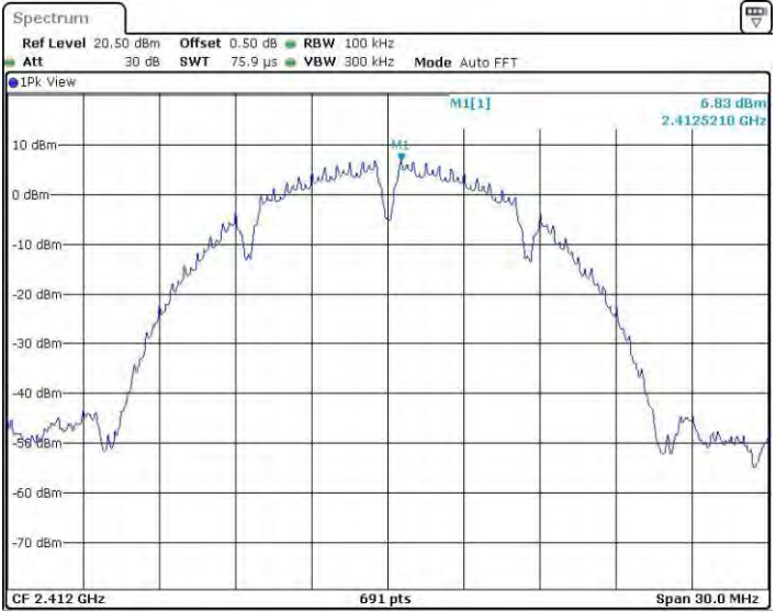
11B_Ant2_2412_0~Reference
