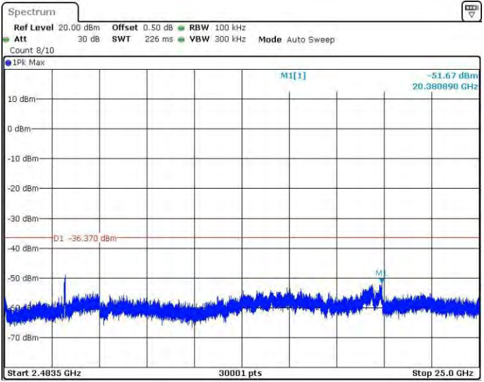
11N40SISO_Ant1_2437_2483.5~25000
