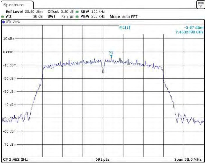
11N20SISO_Ant3_2462_0~Reference
