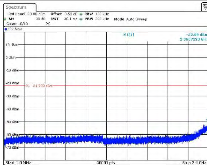
11GMINO_Ant1_2462_0~Reference
