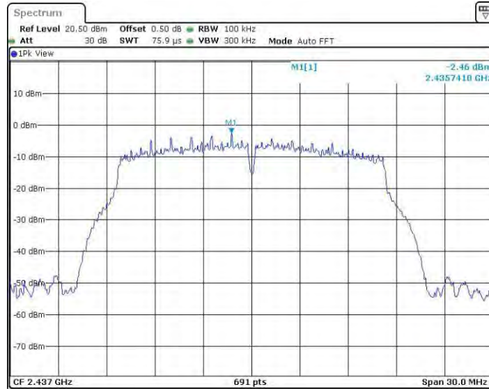
11GMINO_Ant2_2437_0-Reference
