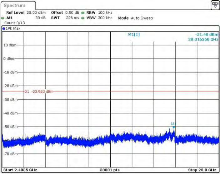
11B_Ant2_2437_2483.5~25000
