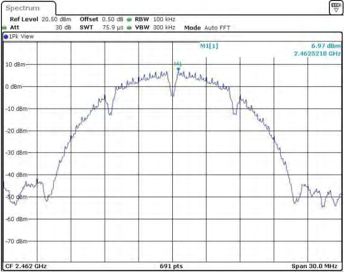
11B_Ant4_2462_0~Reference
