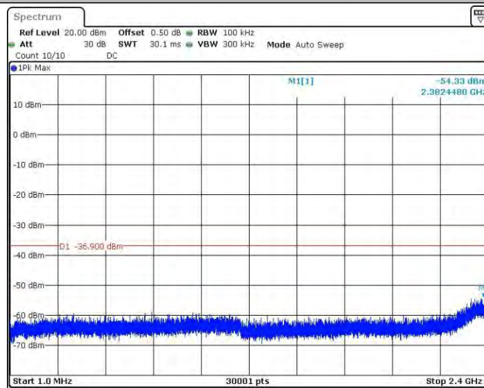
11N40SISO_Ant4_2437_0~Reference
