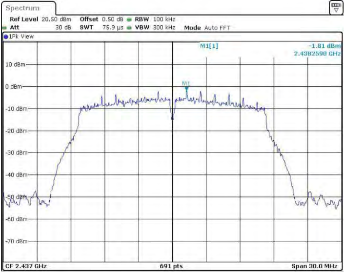
11GMINO_Ant4_2437_0-Reference
