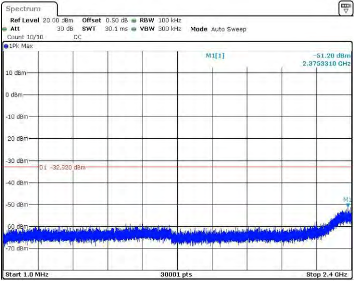
11N20SISO_Ant4_2437_1~2400
