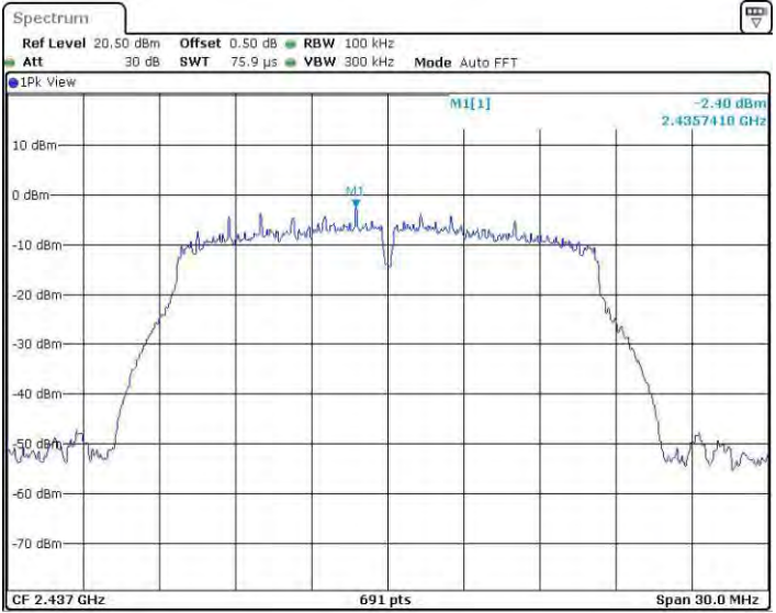
11G_Ant2_2437_0~Reference
