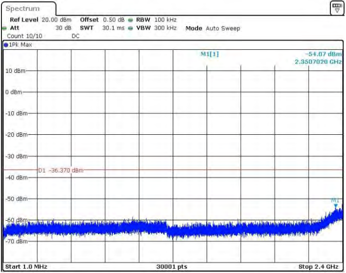
11N40SISO_Ant1_2437_1~2400
