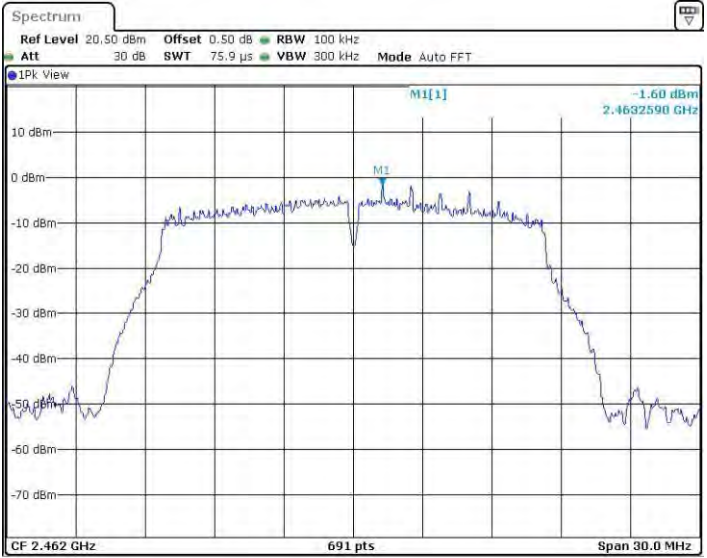
11G_Ant4_2462_0~Reference
