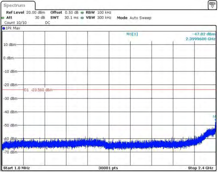
11B_Ant3_2412_1~2400
