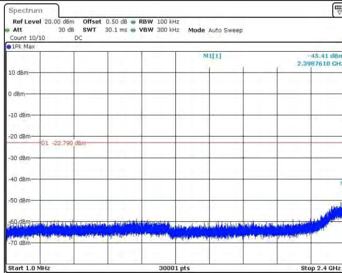
11B_Ant4_2412_0~Reference
