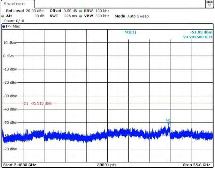
11G_Ant3_2437_2483.5~25000
