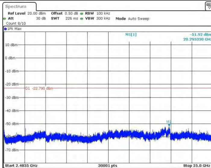
11B_Ant4_2412_2483.5~25000
