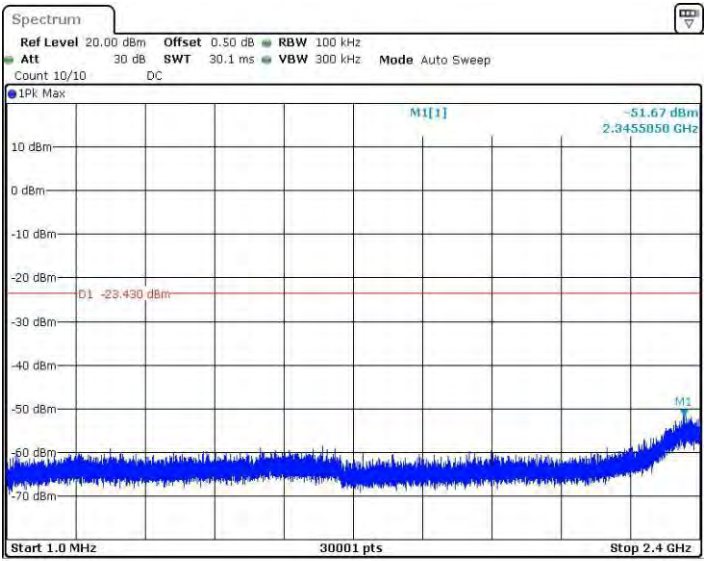
11B_Ant3_2437_1~2400
