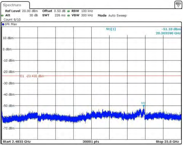
11B_Ant3_2437_2483.5~25000
