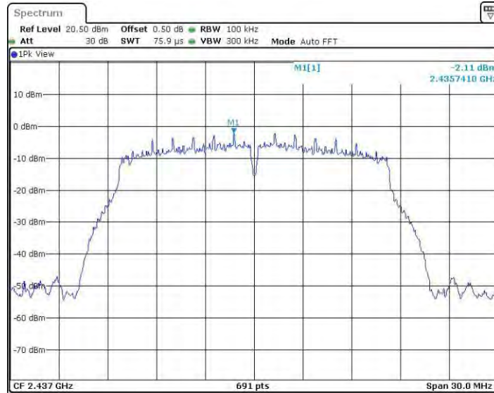
11G_Ant4_2437_0~Reference
