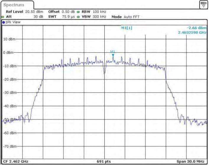
11N20SISO_Ant2_2462_0~Reference
