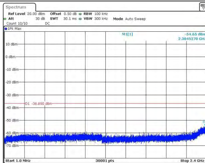
11N40SISO_Ant4_2452_0~Reference
