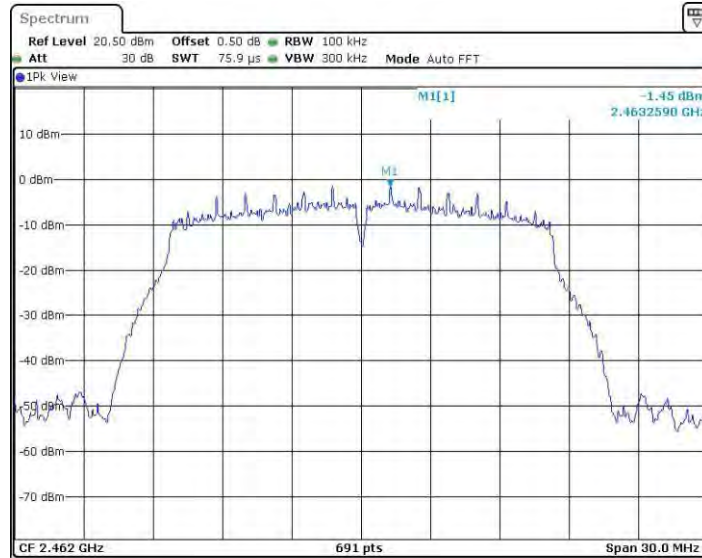
11GMINO_Ant4_2462_0-Reference
