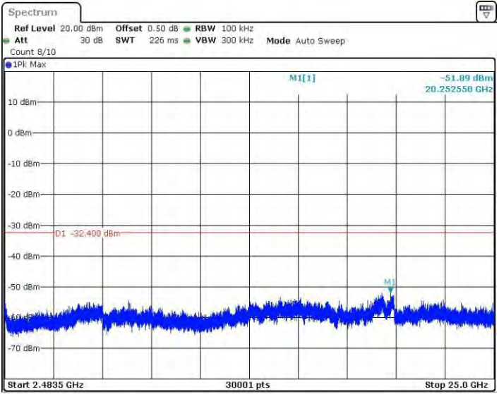
11G_Ant2_2437_2483.5~25000
