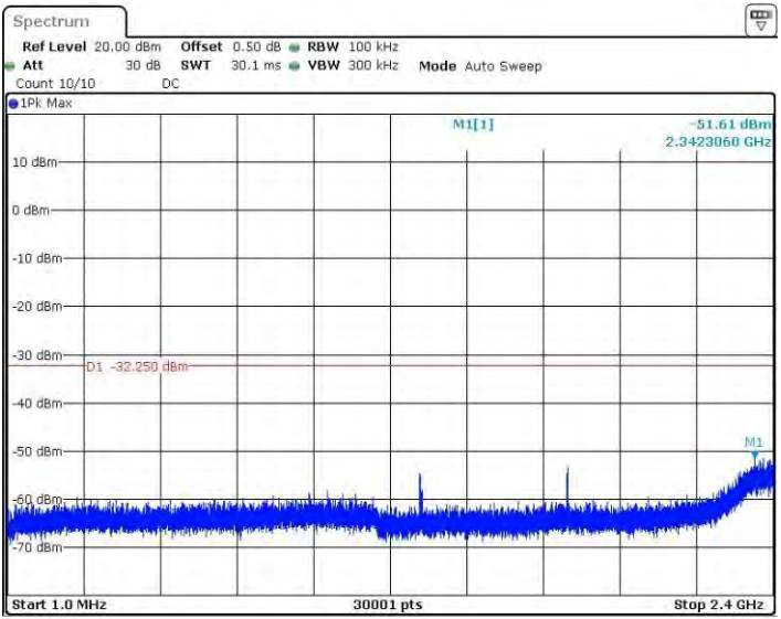
11G_Ant1_2437_1~2400
