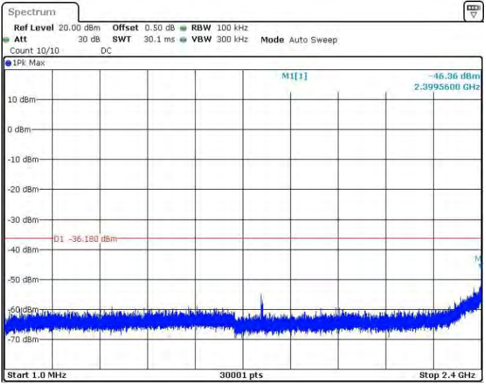
11N40SISO_Ant1_2422_1~2400
