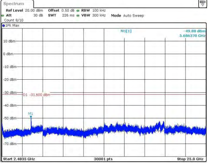
11G_Ant4_2462_2483.5~25000
