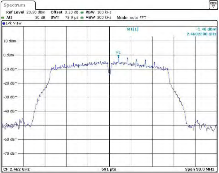
11G_Ant2_2462_0~Reference
