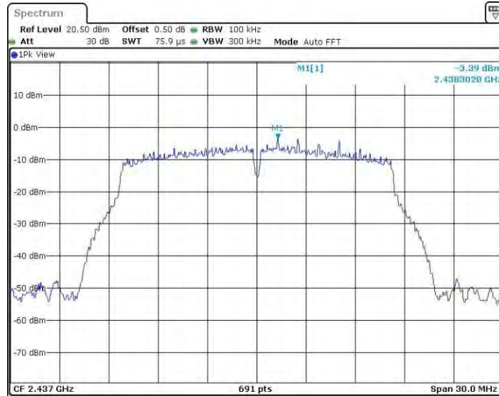
11GMINO_Ant3_2437_0-Reference
