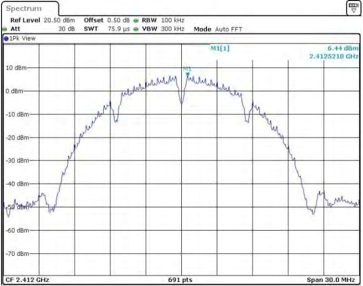
11B_Ant3_2412_0~Reference
