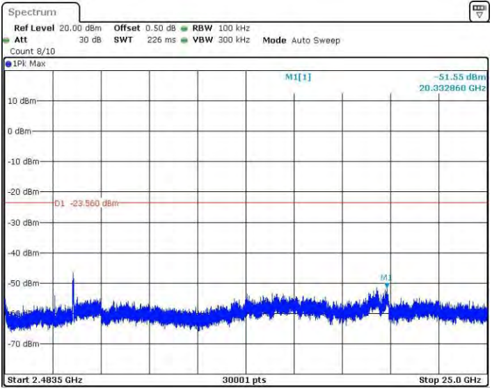
11B_Ant3_2412_2483.5~25000
