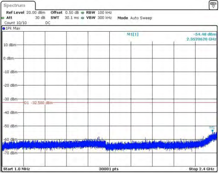
11N20SISO_Ant1_2462_1~2400
