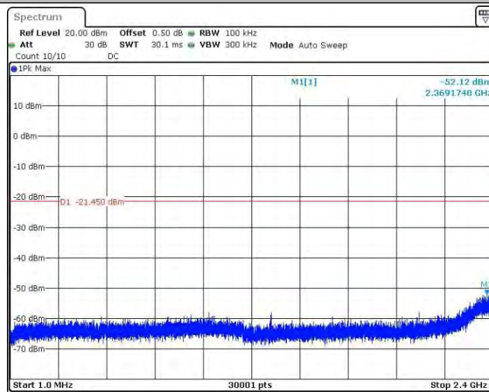
11GMINO_Ant4_2462_0-Reference
