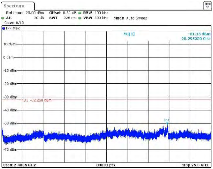
11G_Ant1_2437_2483.5~25000
