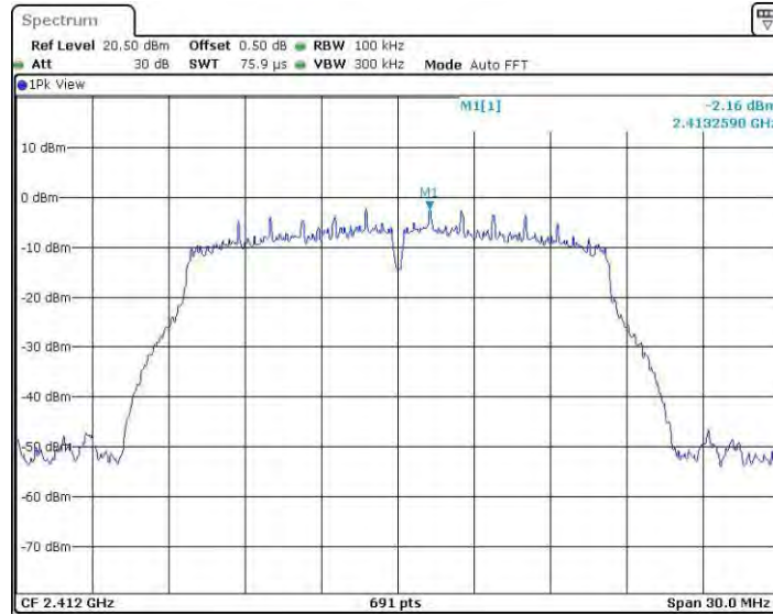
11GMINO_Ant3_2412_0~Reference
