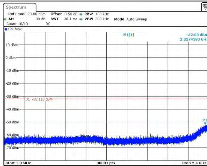
11G_Ant4_2437_0~Reference
