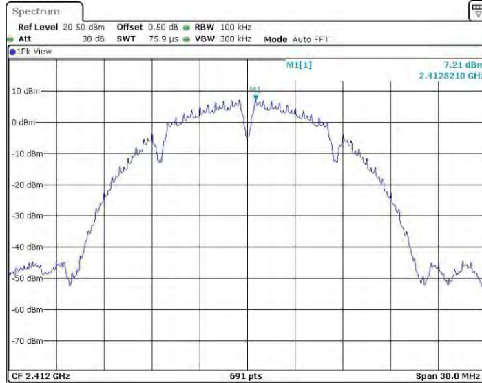
11B_Ant4_2412_0~Reference
