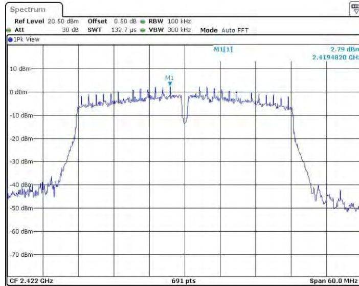
11N40SISO_Ant4_2422_0~Reference
