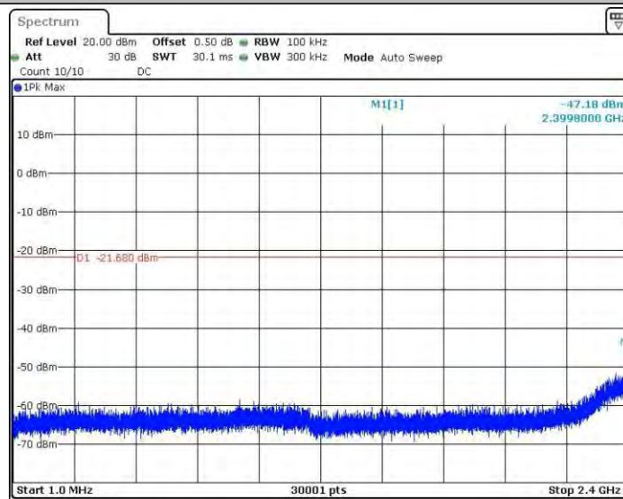
11GMINO_Ant1_2412_0~Reference
