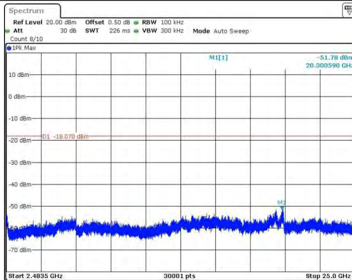
11N40SISO_Ant4_2437_2483.5~25000
