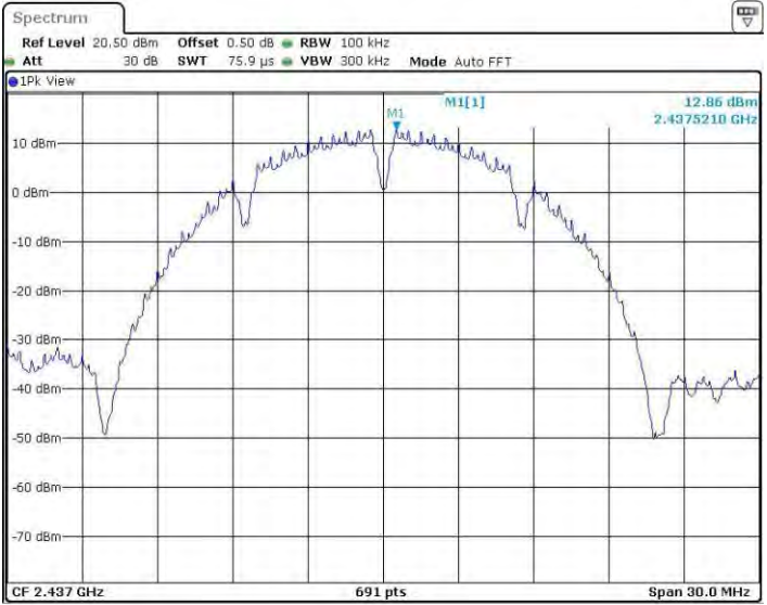
11BSISO_Ant2_2437_0~Reference
