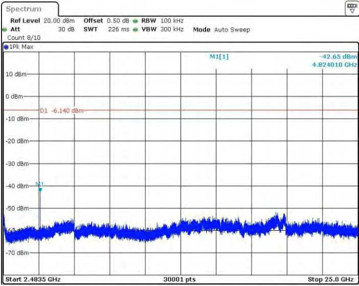
11BSISO_Ant1_2412_2483.5~25000
