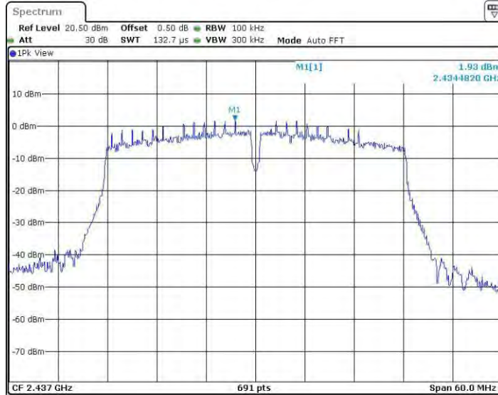
11N40SISO_Ant4_2437_0~Reference
