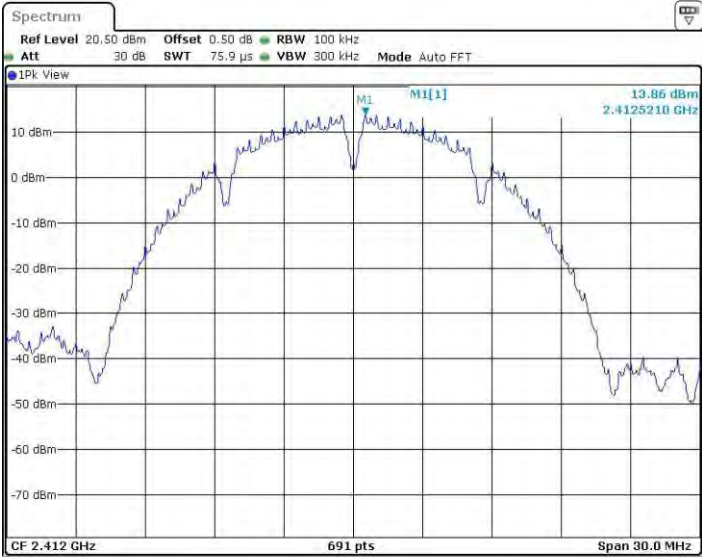
11BSISO_Ant1_2412_0~Reference
