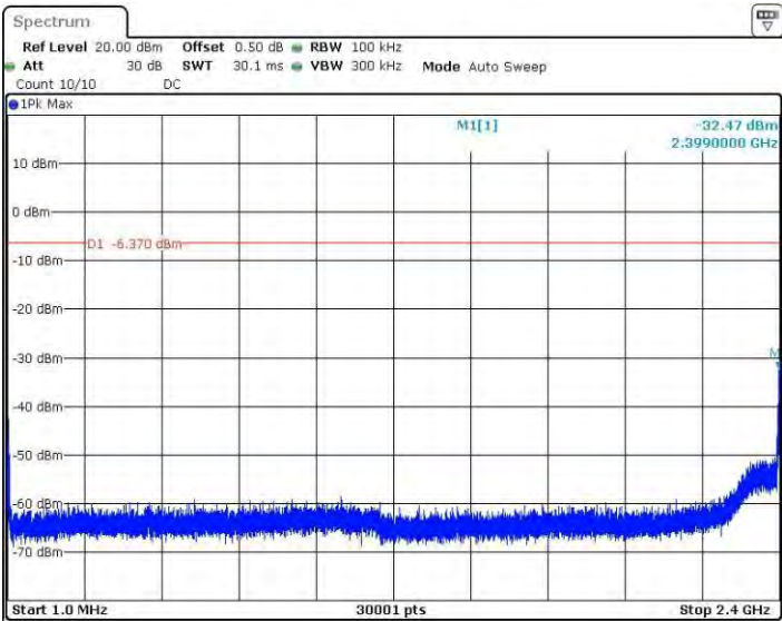
11BSISO_Ant2_2412_0~Reference
