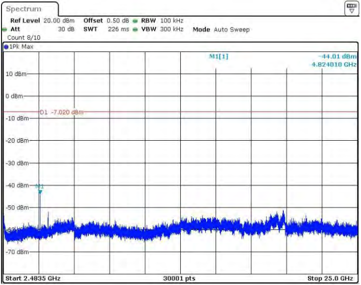
11BSISO_Ant4_2412_2483.5~25000
