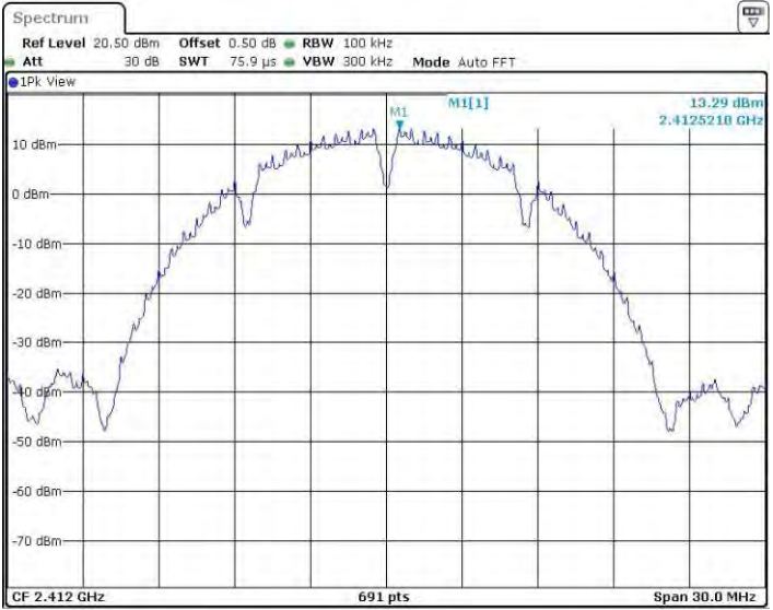
11BSISO_Ant3_2412_0~Reference
