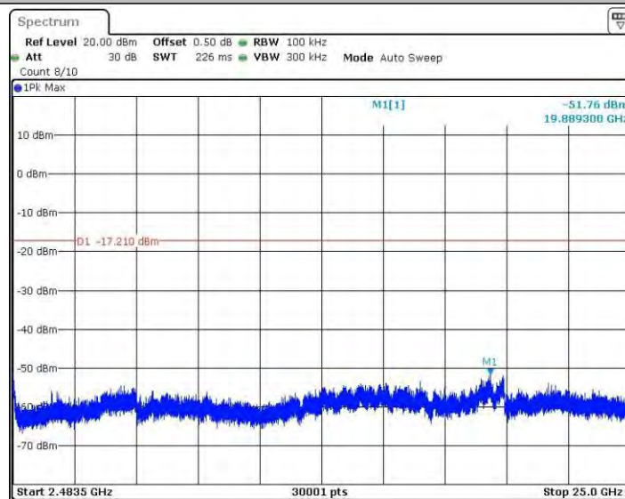
11N40SISO_Ant4_2422_2483.5~25000
