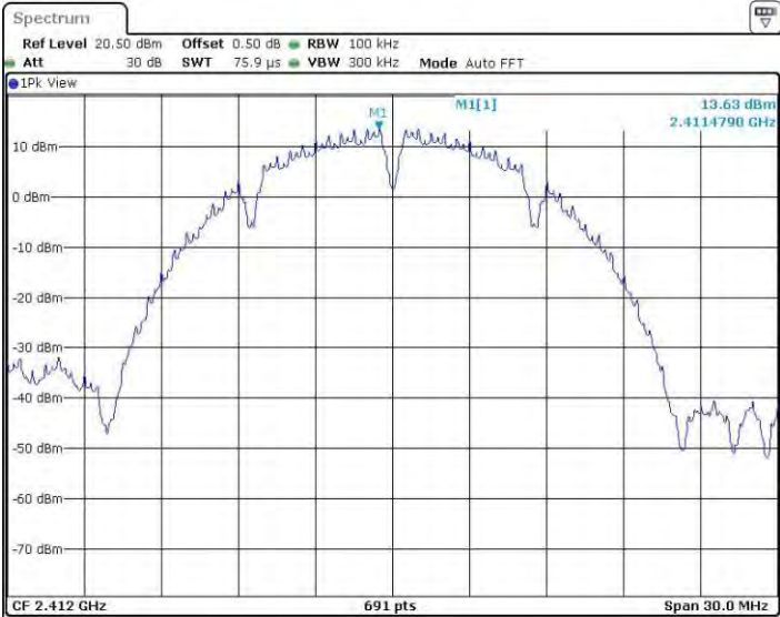
11BSISO_Ant2_2412_0~Reference
