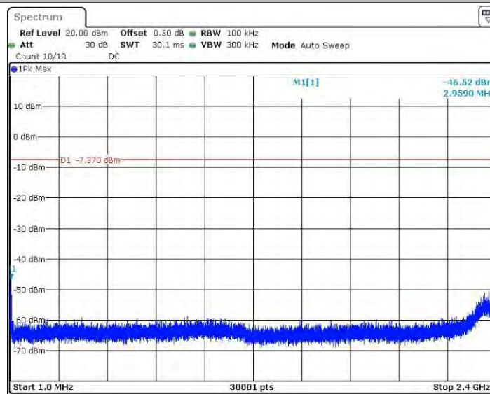
11BSISO_Ant4_2437_0~Reference
