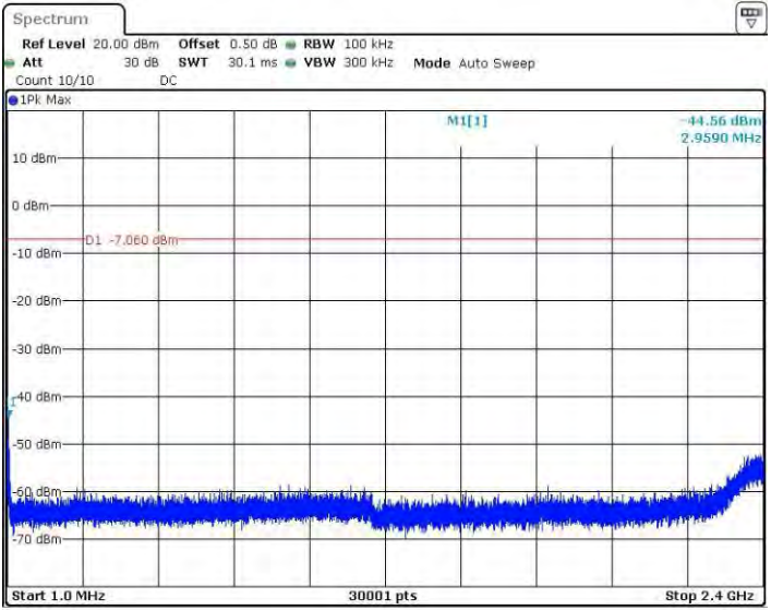
11BSISO_Ant4_2462_1~2400
