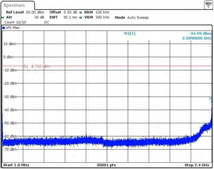
11BSISO_Ant3_2412_1~2400
