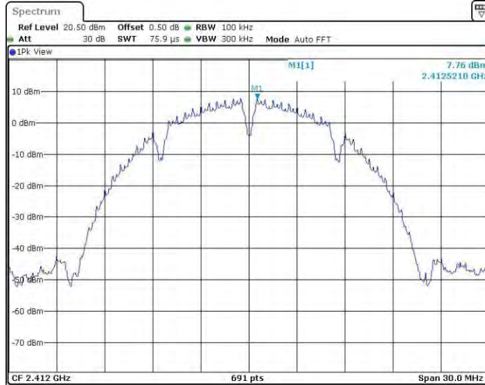
11BMINO_Ant3_2412_0~Reference
