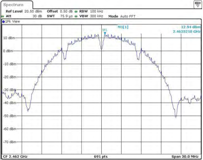
11BSISO_Ant4_2462_0~Reference
