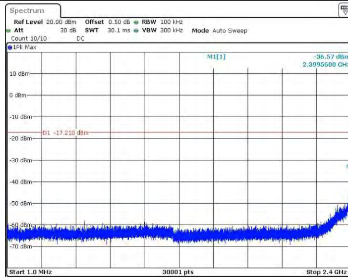
11N40SISO_Ant4_2422_1~2400
