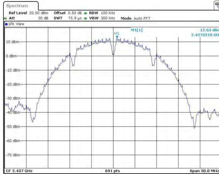
11BSISO_Ant4_2437_0~Reference
