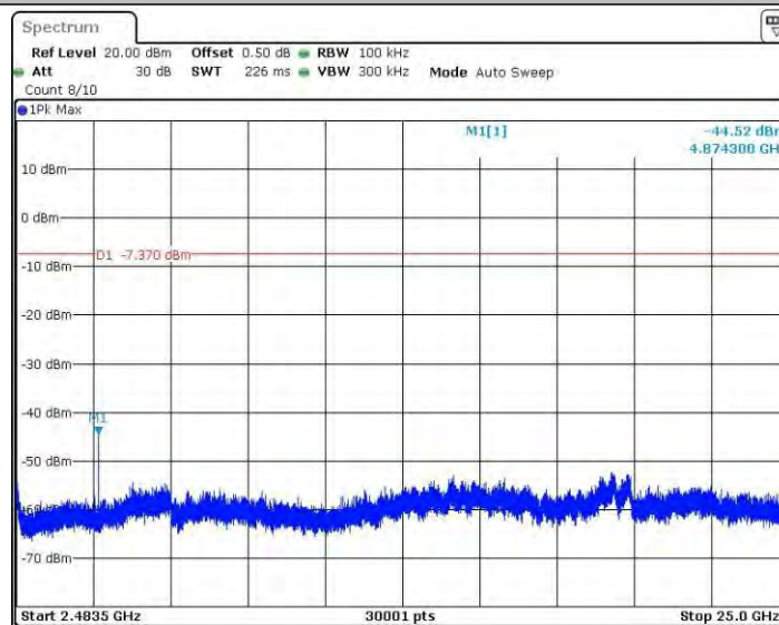
11BSISO_Ant4_2437_1~2400
