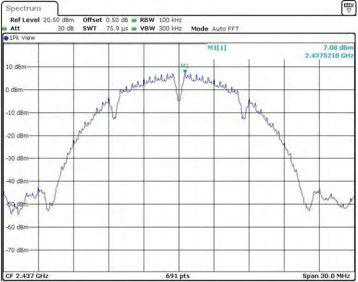
11BMINO_Ant3_2437_0~Reference
