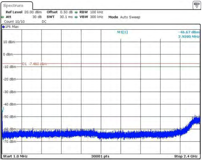
11BSISO_Ant3_2437_1~2400
