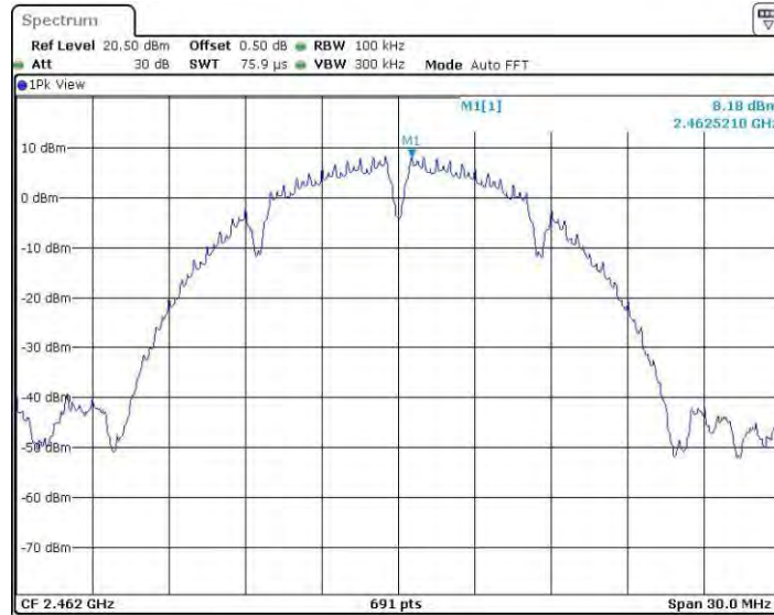
11BMINO_Ant4_2462_0~Reference
