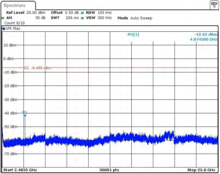
11BSISO_Ant1_2437_2483.5~25000
