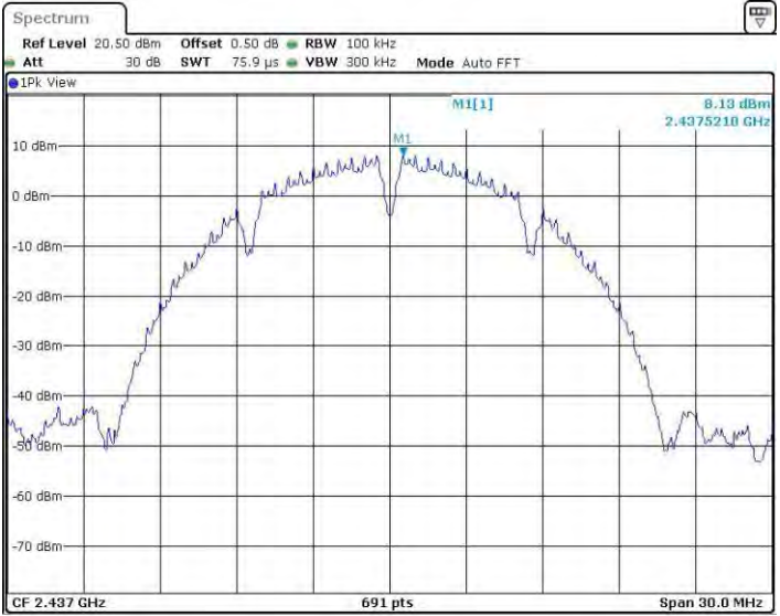
11BMINO_Ant1_2437_0~Reference
