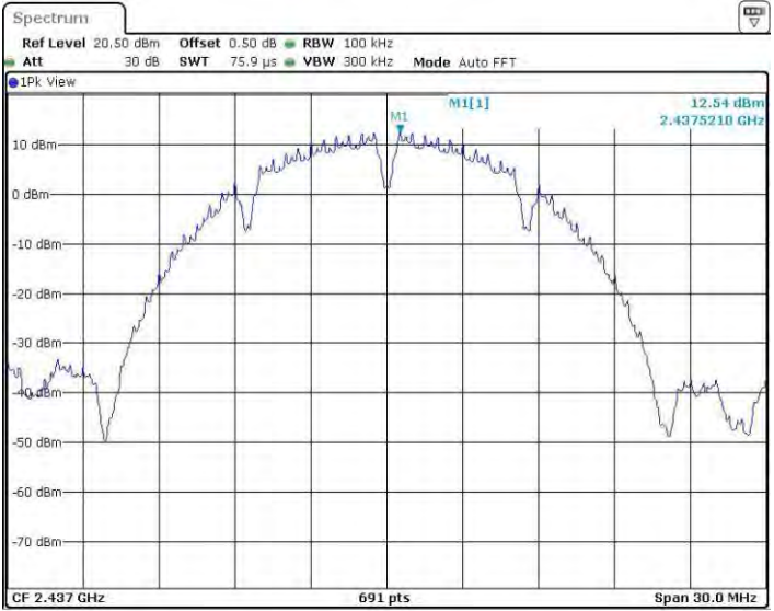
11BSISO_Ant3_2437_0~Reference
