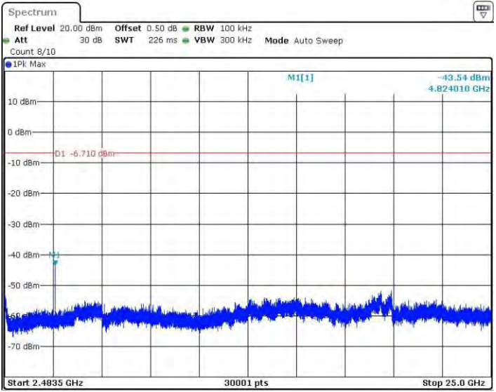
11BSISO_Ant3_2412_2483.5~25000
