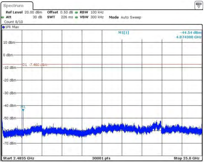
11BSISO_Ant3_2437_2483.5~25000
