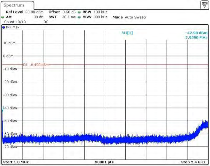
11BSISO_Ant1_2437_1~2400
