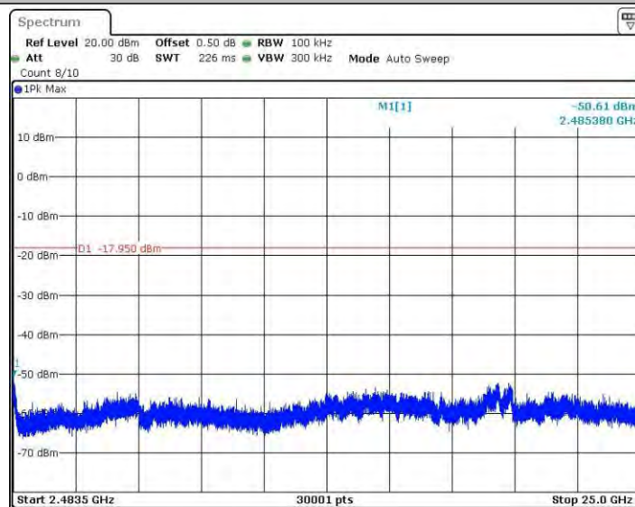
11N40SISO_Ant3_2437_1~2400
