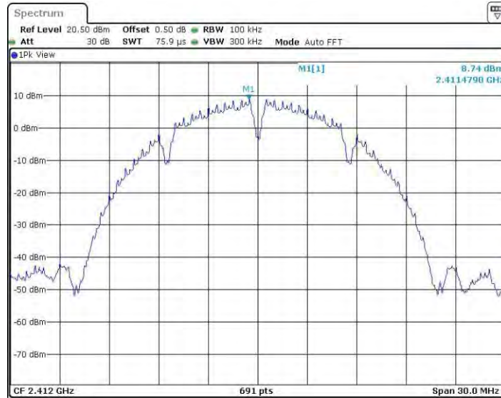
11BMINO_Ant4_2412_0~Reference
