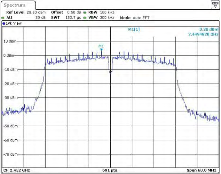
11N40SISO_Ant2_2452_0~Reference
