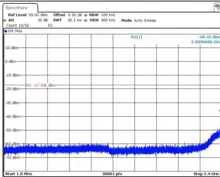
11N40SISO_Ant2_2422_0~Reference
