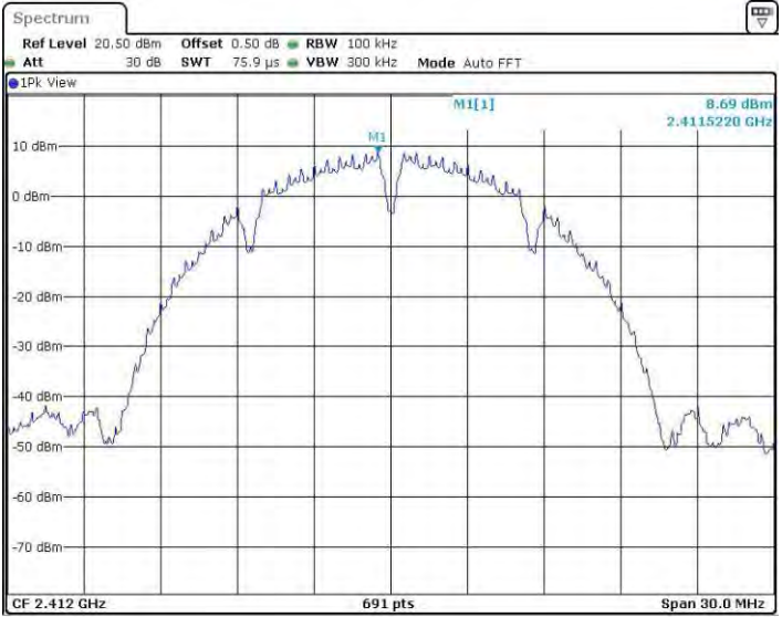
11BMINO_Ant1_2412_0~Reference
