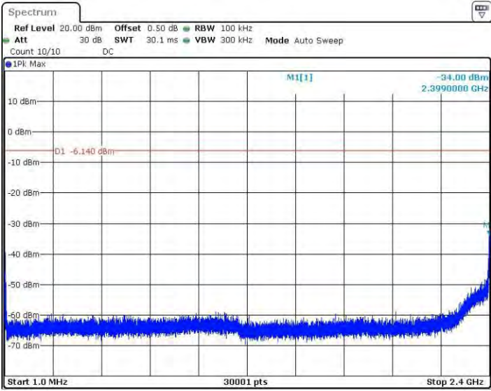
11BSISO_Ant1_2412_1~2400
