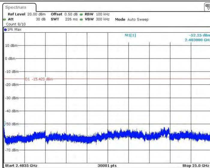
11N20SISO_Ant4_2462_2483.5~25000
