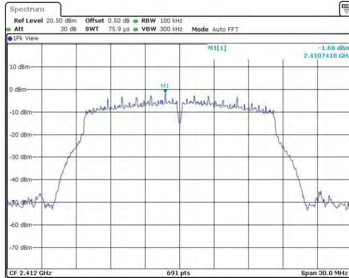
11GMINO_Ant1_2412_0~Reference
