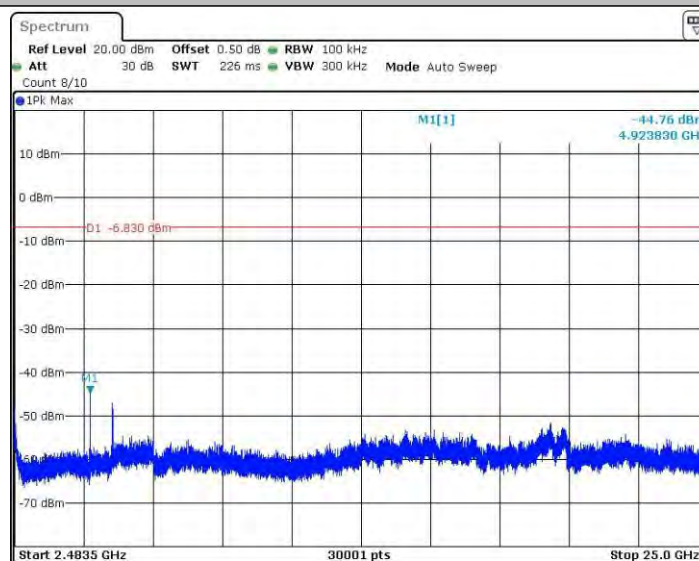
11BSISO_Ant3_2462_1~2400
