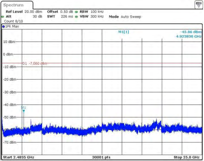
11BSISO_Ant4_2462_2483.5~25000
