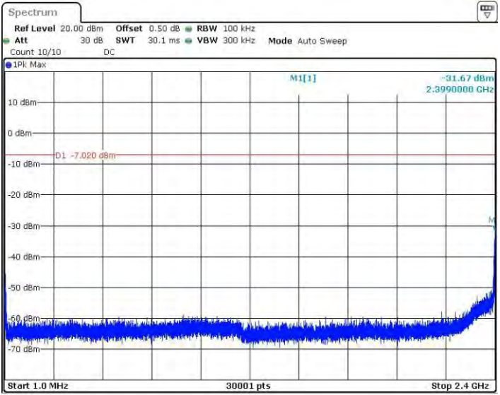
11BSISO_Ant4_2412_1~2400
