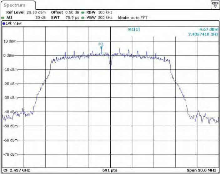
11GSISO_Ant1_2437_0~Reference
