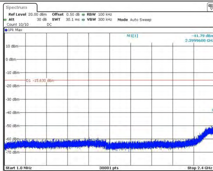
11N20SISO_Ant3_2412_0~Reference
