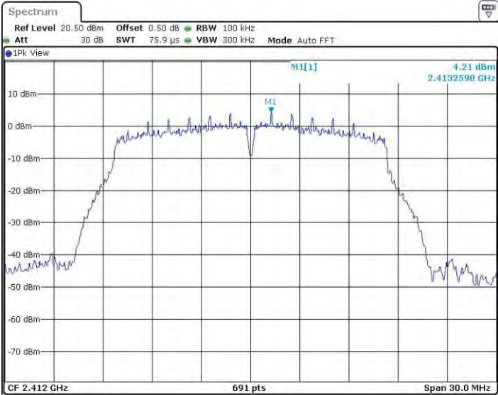
11GSISO_Ant4_2412_0~Reference
