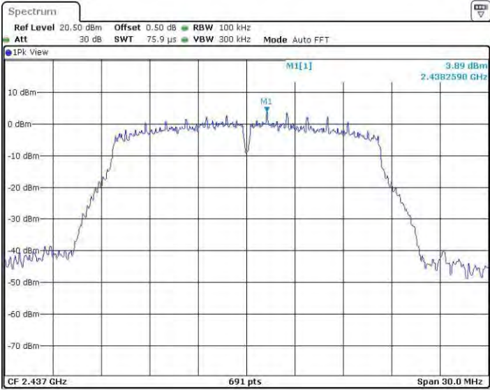
11GSISO_Ant2_2437_0~Reference
