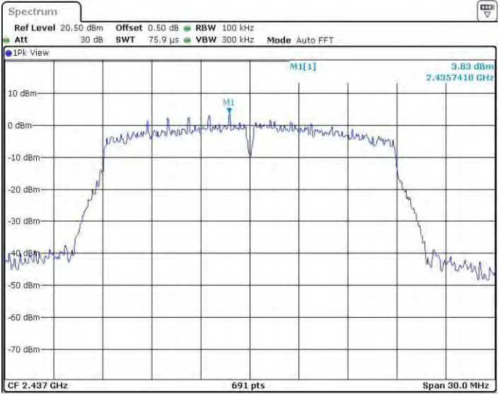
11N20SISO_Ant2_2437_0~Reference
