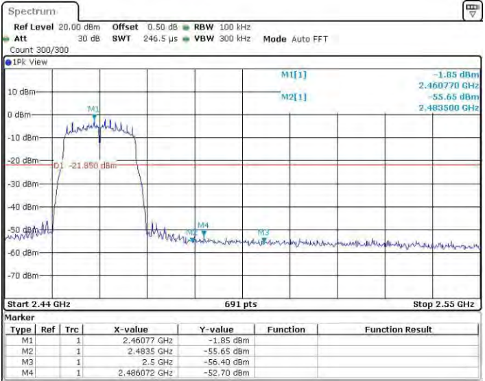
11GMINO_Ant4_High_2462
