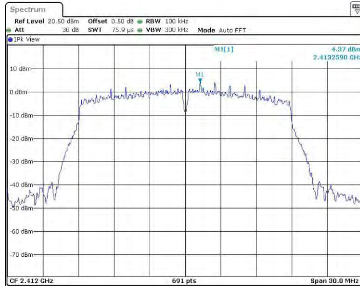
11N20SISO_Ant3_2412_0~Reference
