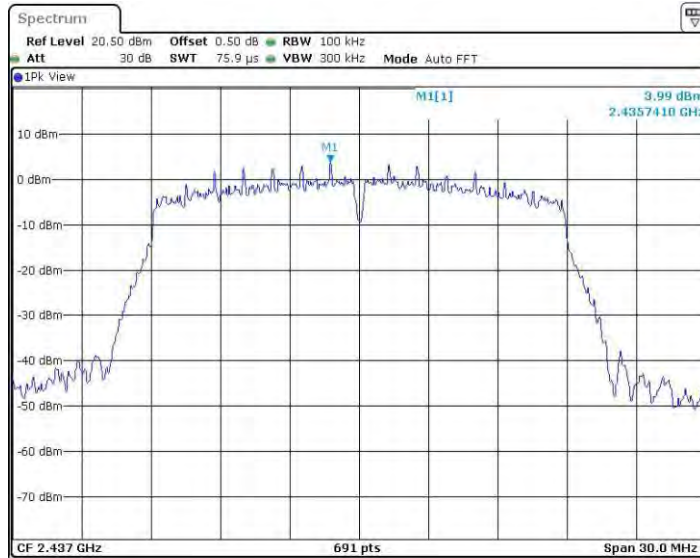
11N20SISO_Ant3_2437_0~Reference
