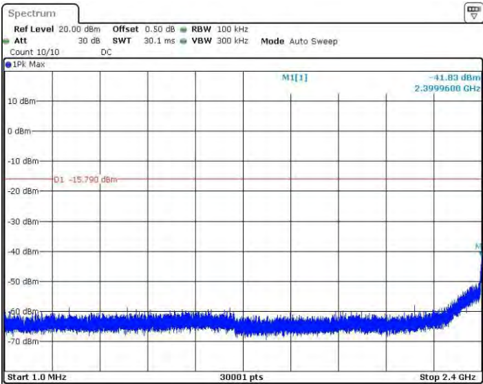
11GSISO_Ant4_2412_0~Reference
