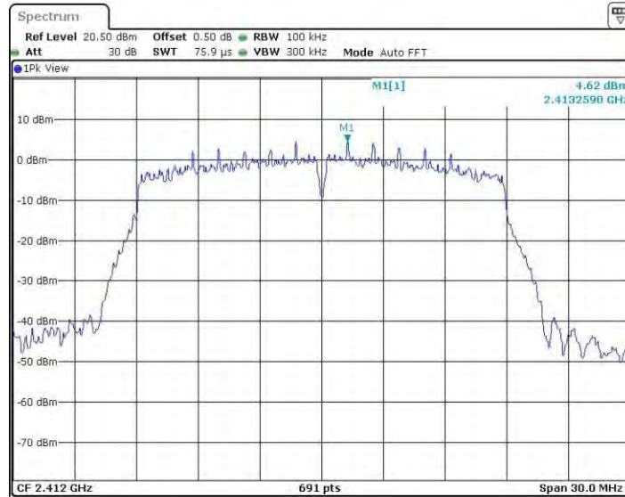
11N20SISO_Ant4_2412_0~Reference
