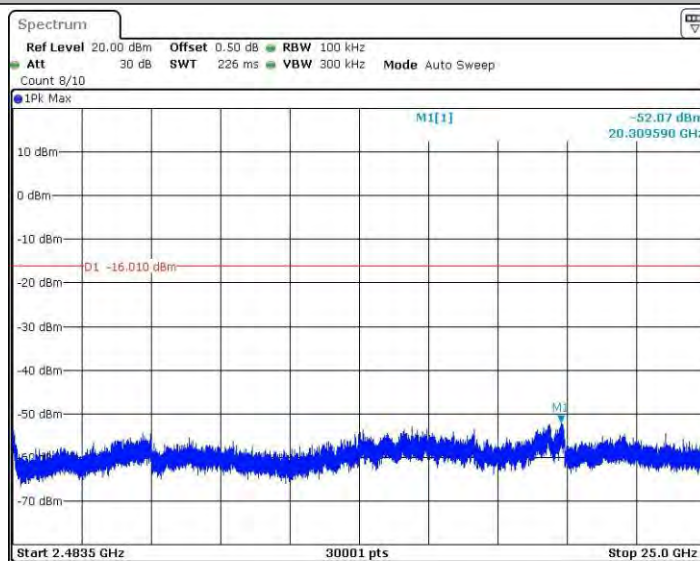
11N20SISO_Ant3_2437_2483.5~25000
