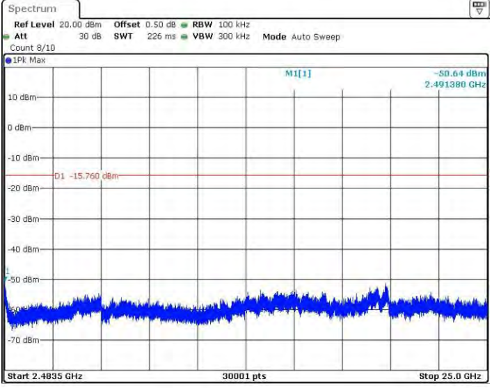
11N20SISO_Ant1_2437_2483.5~25000
