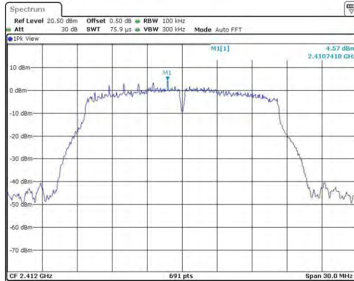
11GSISO_Ant3_2412_0~Reference
