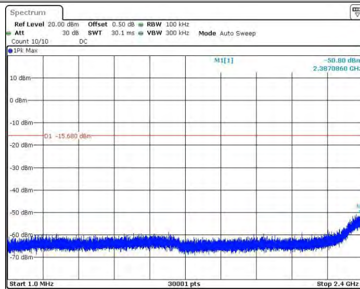
11GSISO_Ant1_2462_0~Reference
