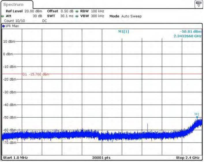
11N20SISO_Ant1_2437_1~2400
