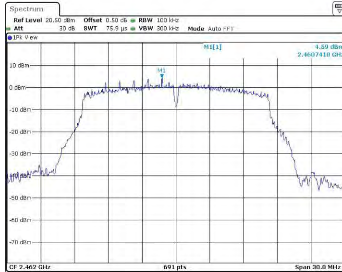
11GSISO_Ant3_2462_0~Reference
