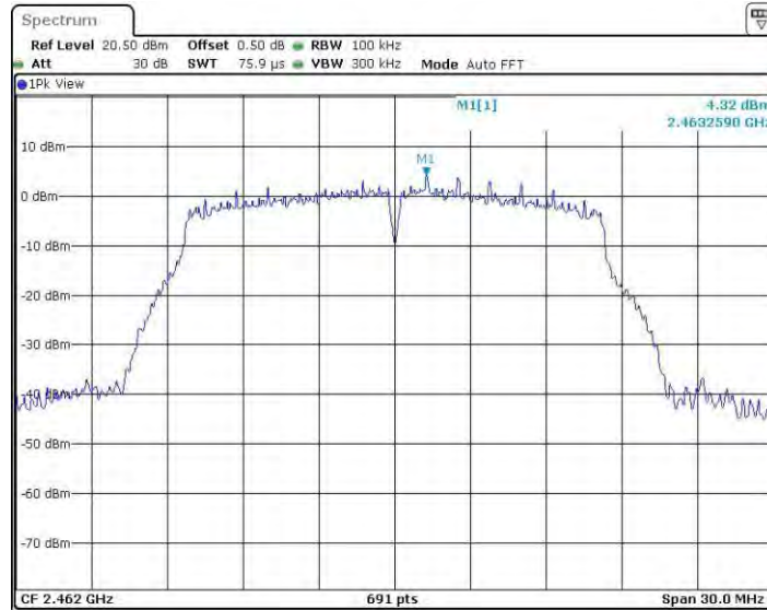
11GSISO_Ant1_2462_0~Reference
