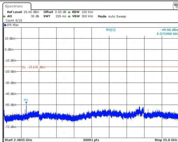
11N20SISO_Ant3_2412_2483.5~25000
