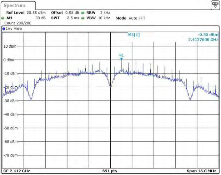
11BSISO_Ant3_2412
