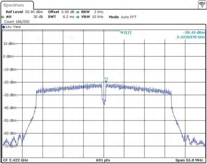
11N40SISO_Ant3_2422
