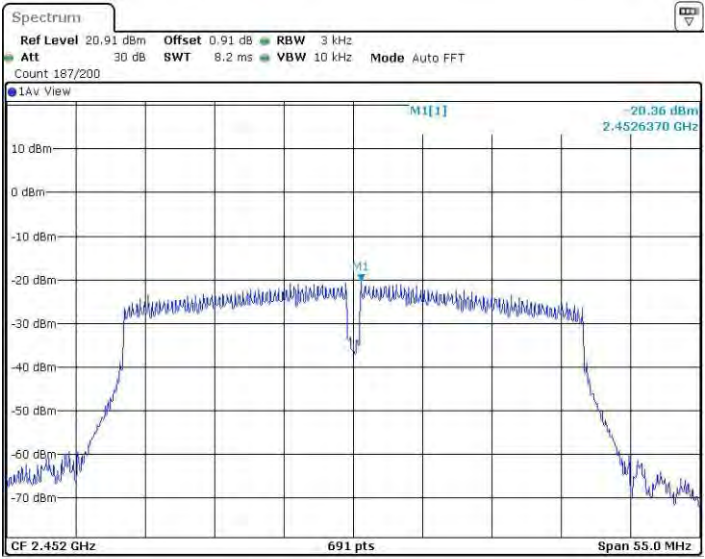
11N40SISO_Ant4_2452
