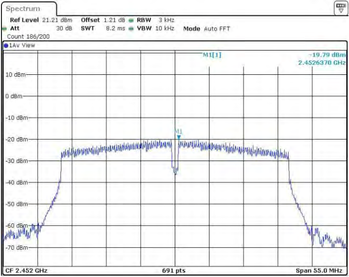
11N40SISO_Ant3_2452
