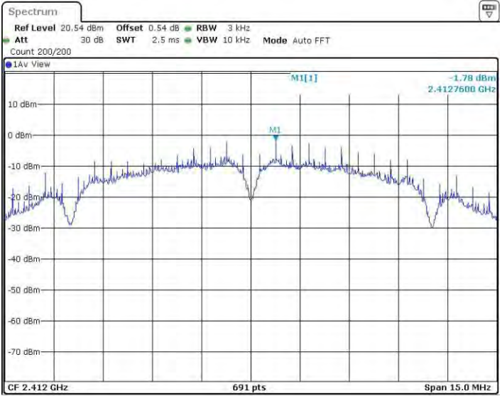
11BSISO_Ant4_2412
