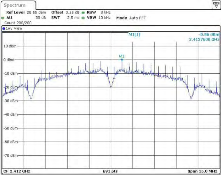
11BSISO_Ant1_2412
