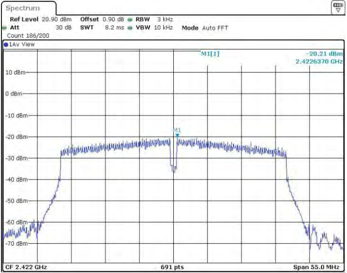
11N40SISO_Ant4_2422
