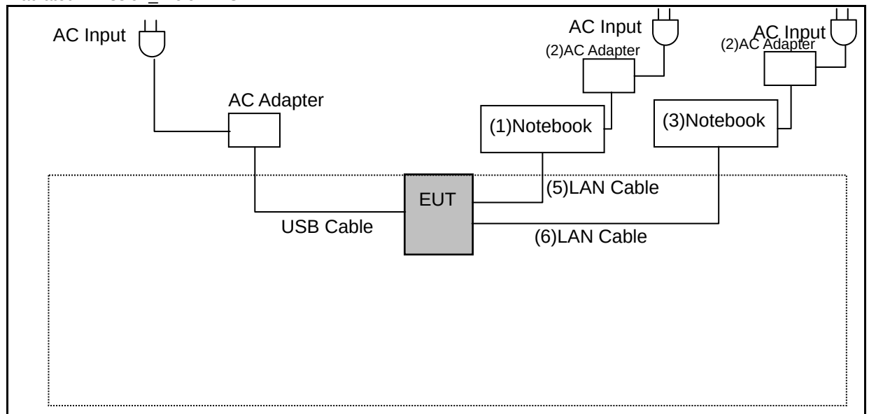
Radiated Emission_ Below 1 GHz
