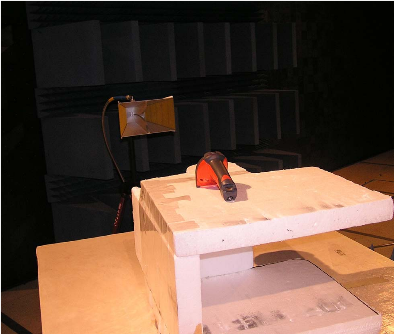
RADIATED EMISSIONS - Back
