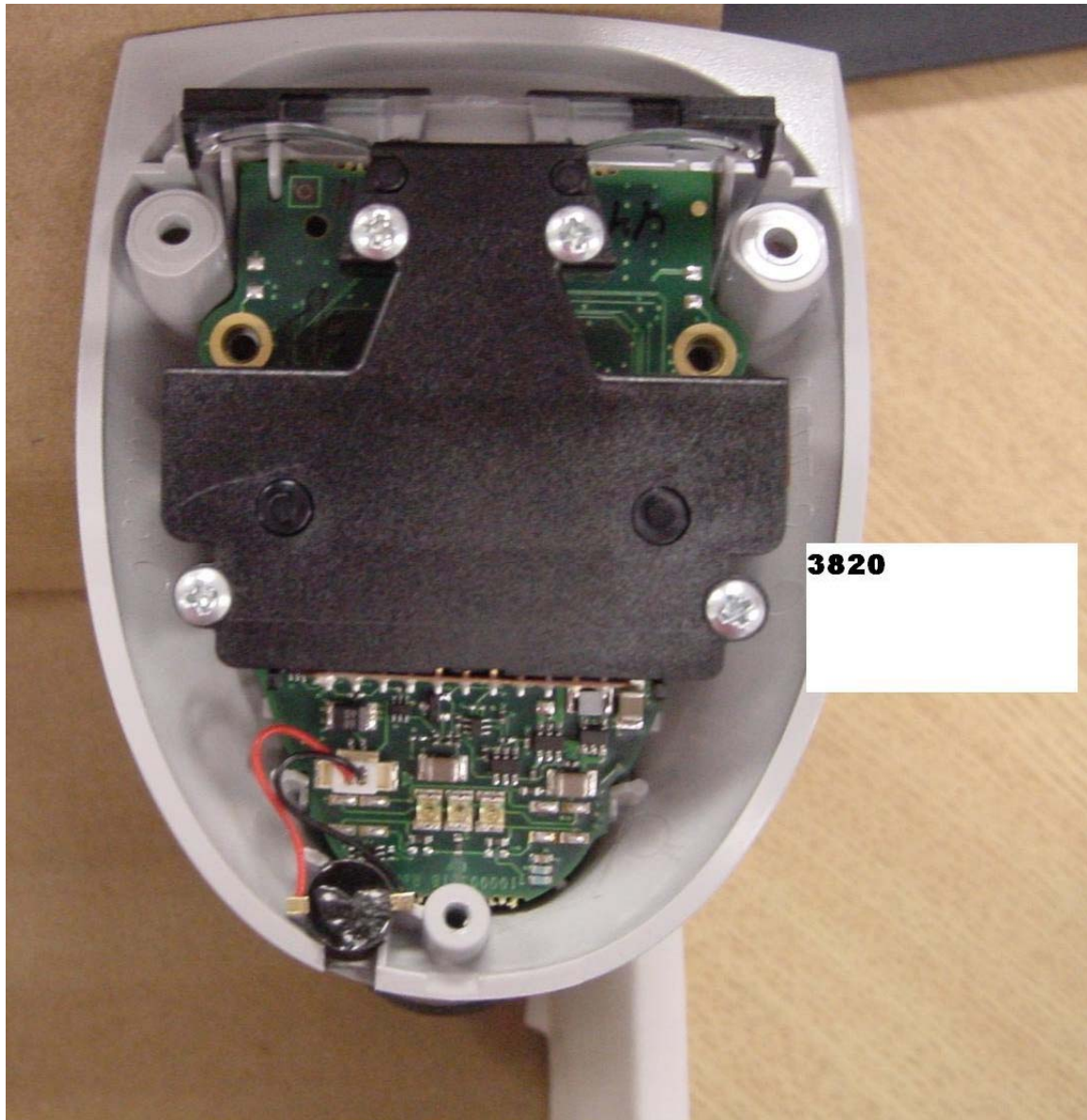
3820 Top view
