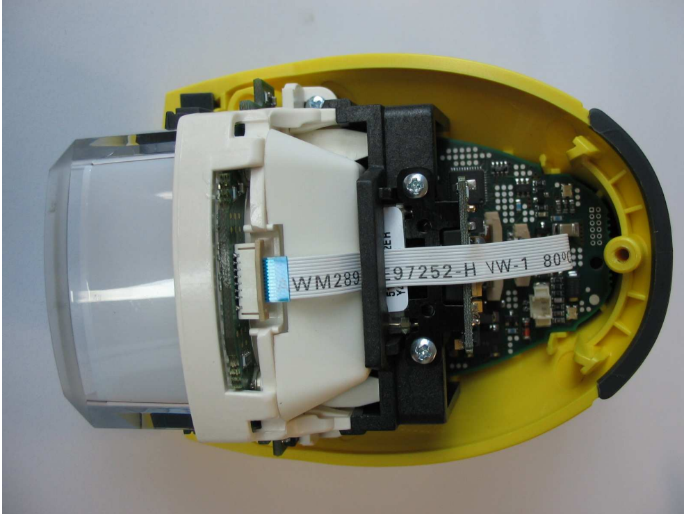
Open 6320 with imager, illumination and main board
