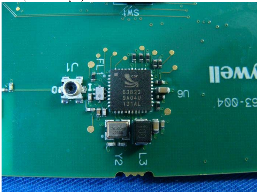
(10) EUT Photo (Bluetooth Chipset)
