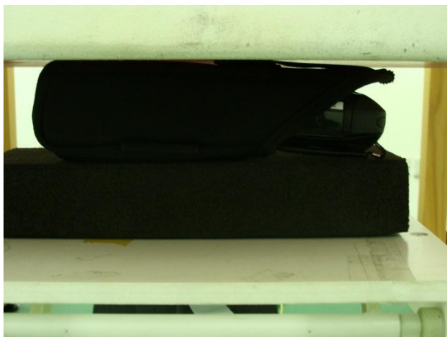
Face of the DUT and Holster 1 with Phantom 0 cm Gap (DUT with Keypad 1)
