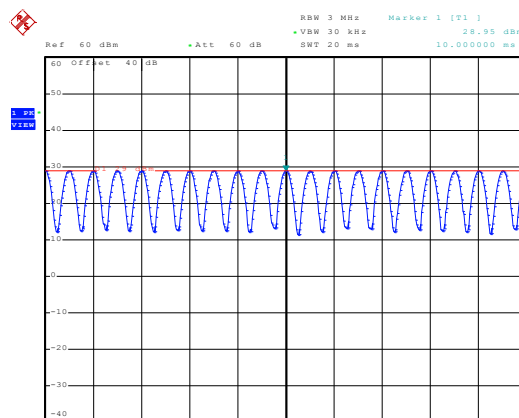
1880MHz - 80% AM
