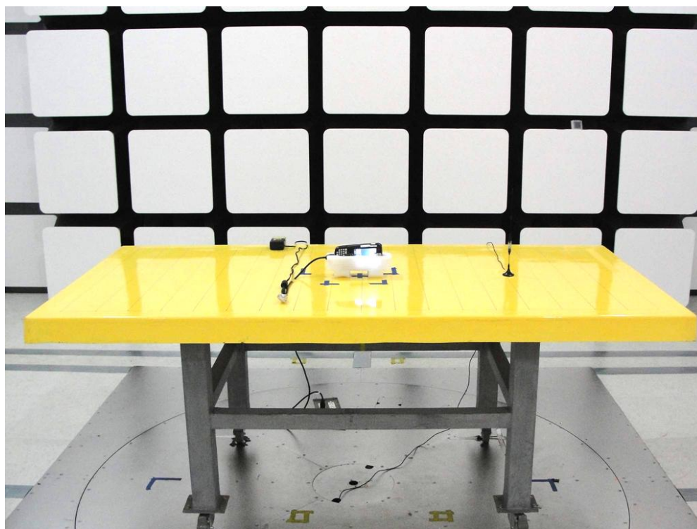
GSM Link + RS232 Cable 1 for EUT with Keypad 2 and Scanner 1
