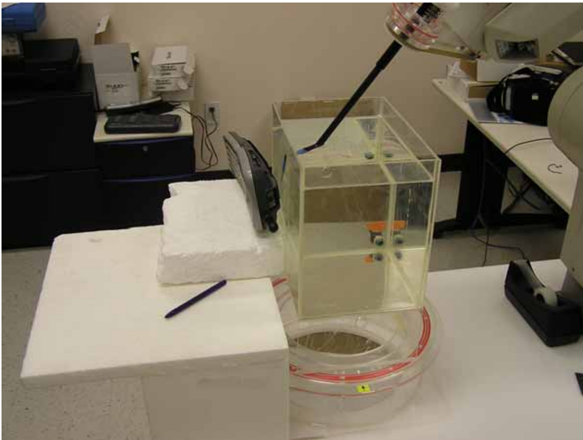
Photo 7 Body SAR WLAN
