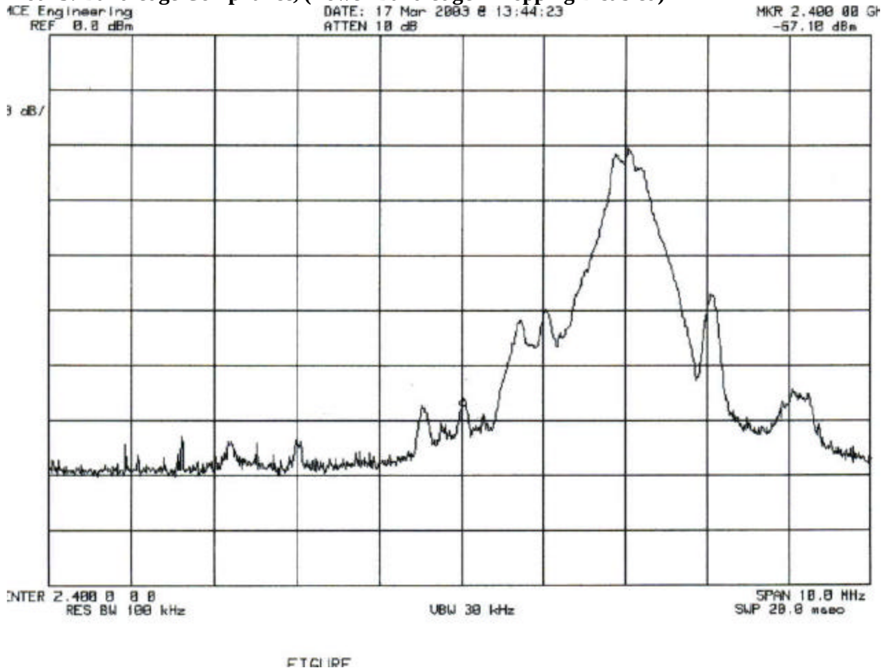
Plot 15: Band-edge Compliance, (Lower Band-edge – Hopping Disabled)
