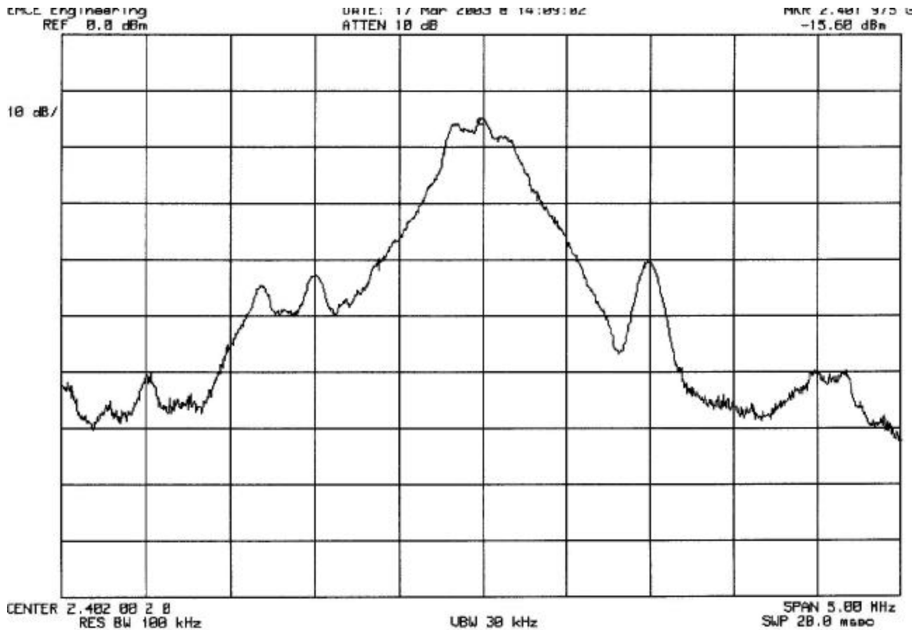
Plot 1: Peak output power 2402 MHz
