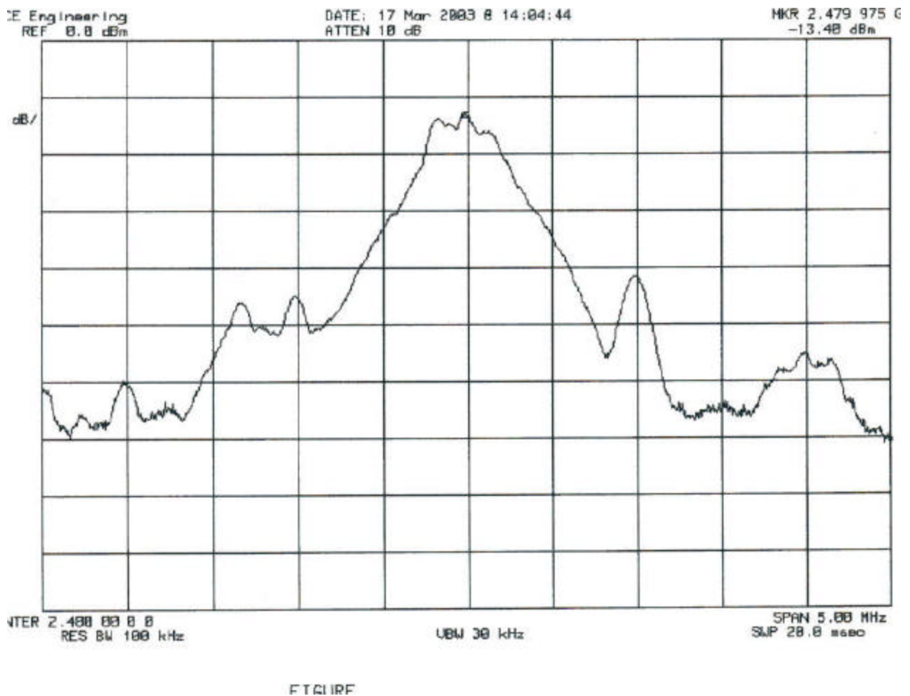
Plot 3: Peak output power 2480 MHz
