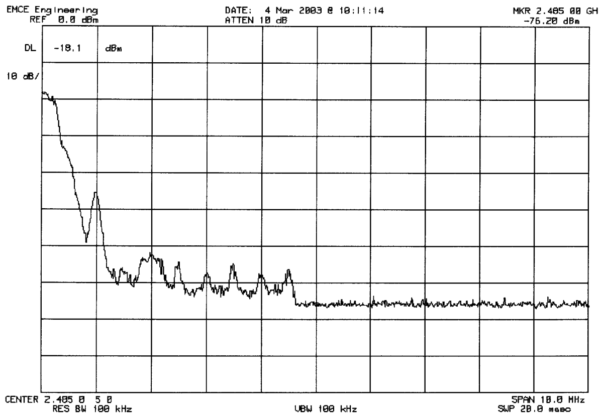
Plot 16: Band-edge compliance, (Upper Band-edge – Hopping Enabled)
