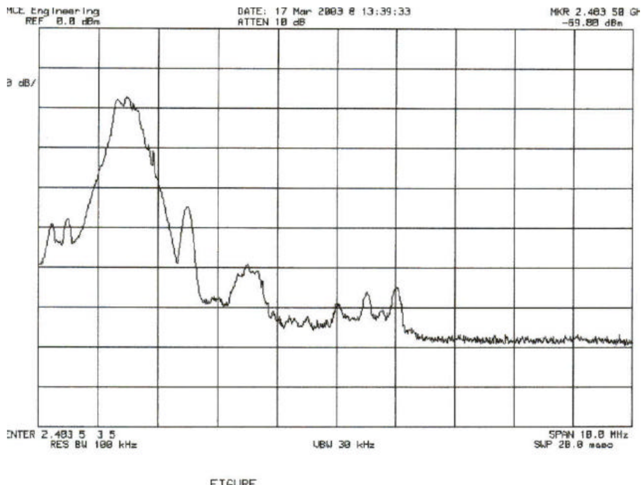
Plot 17: Band-edge compliance, (Upper Band-edge – Hopping Disabled)
