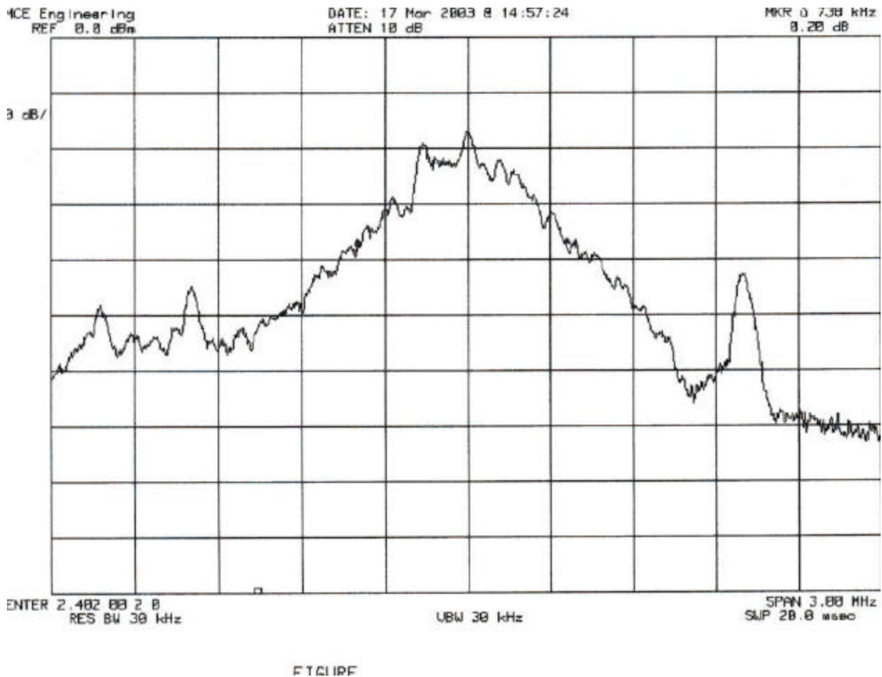
Plot 11: 20 dB BW 2402 MHz
