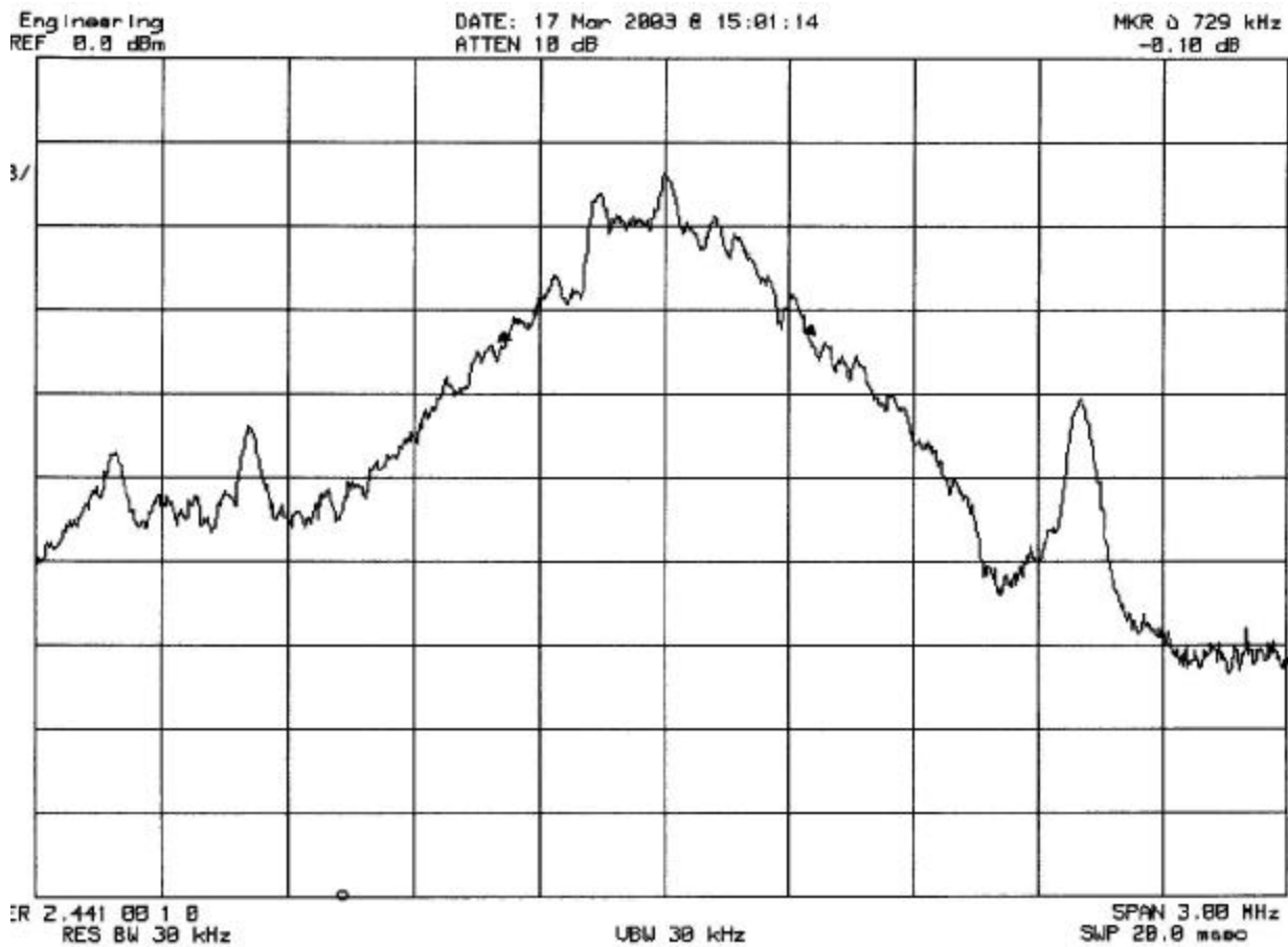
Plot 12: 20 dB BW 2441 MHz
