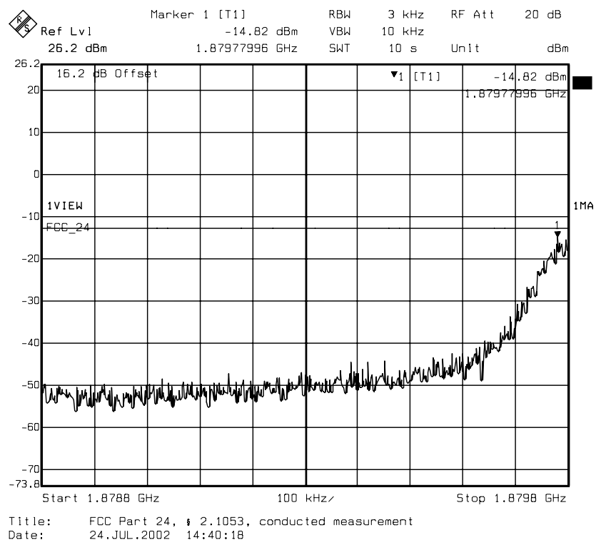
diagram 14.08: carrier on channel 661 (1880 MHz)
