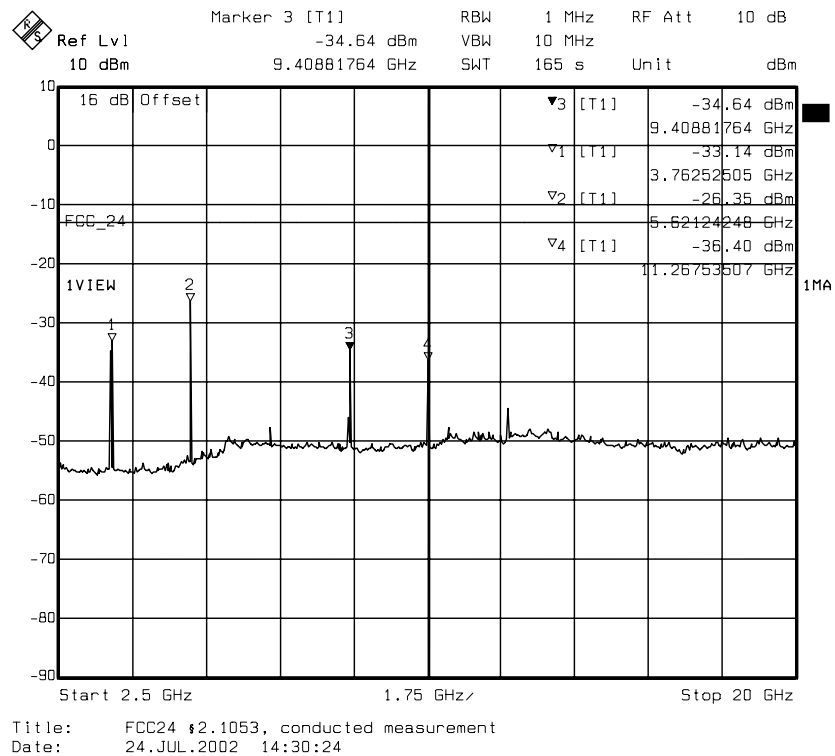
diagram 14.07: carrier on channel 661 (1880 MHz)
