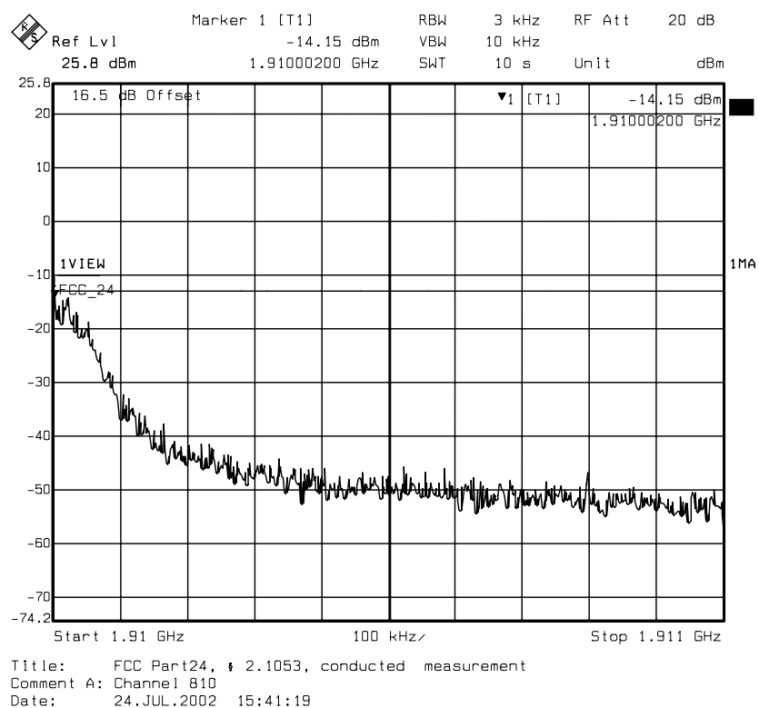
diagram 14.13: carrier on channel 810 (1909.8 MHz)
