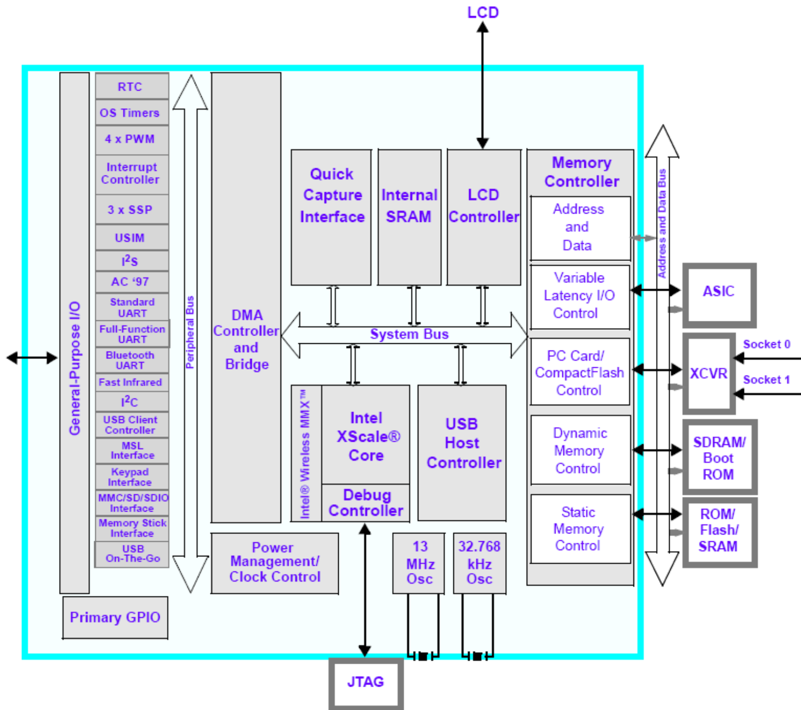
Figure 5. Intel PXA 270 block diagram.
