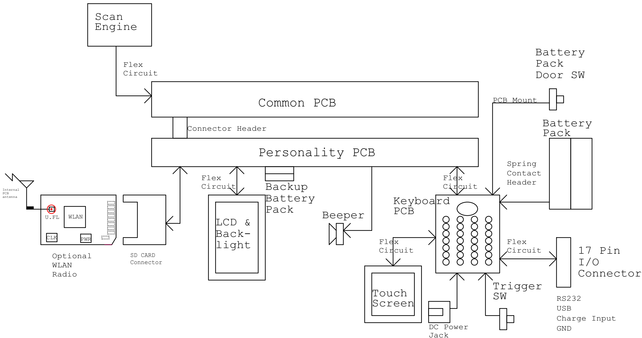
Figure 1. 7850-LOE/E0E 802.11g Terminal Block Diagram
